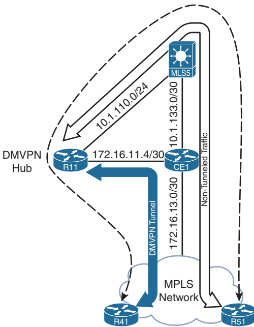
Figure 16-5 Traffic Patterns During Migration to DMVPN Networks
