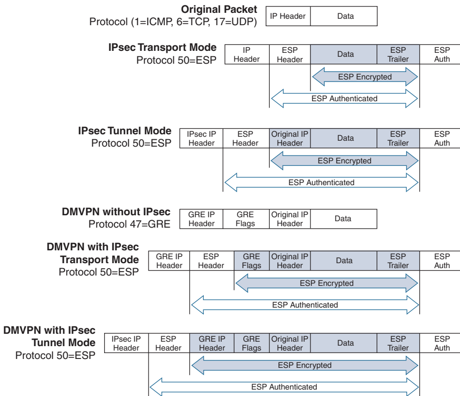
Figure 5-4 DMVPN Packet Headers
