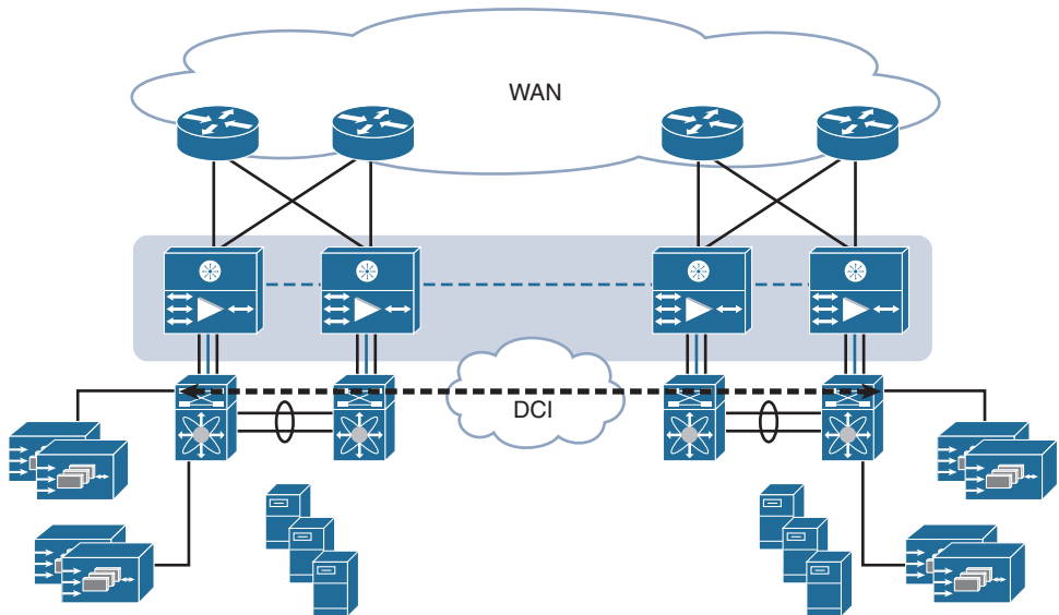
Figure 13-3 WAN Edge with AppNav-XE and WAVE Placement
