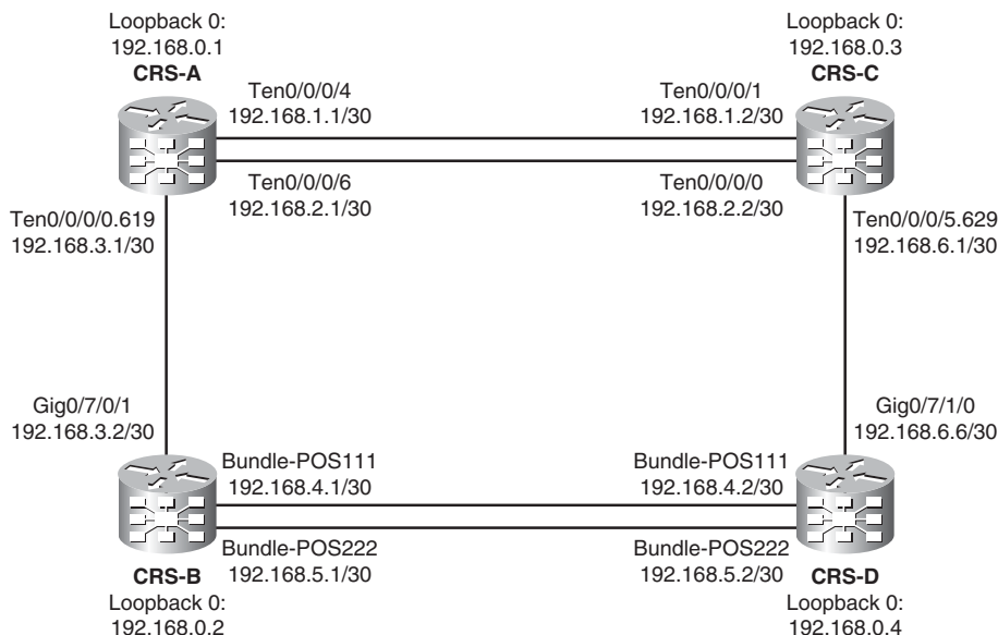
Figure 9-2 MPLS Network
