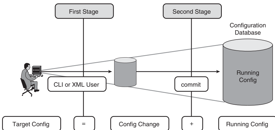
Figure 4-5 Two-Stage Configuration
