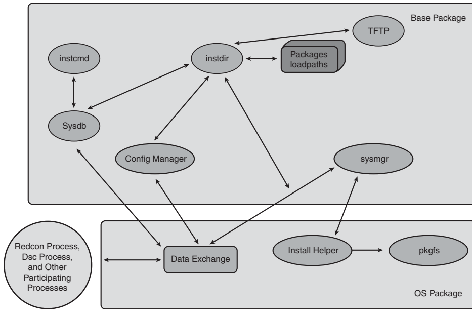
Figure 3-2 An Overview of Install Subsystems and Collaborating Processes
