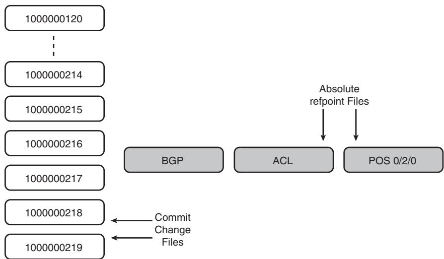
Figure 4-3 Absolute and Commit Reppoint Files
