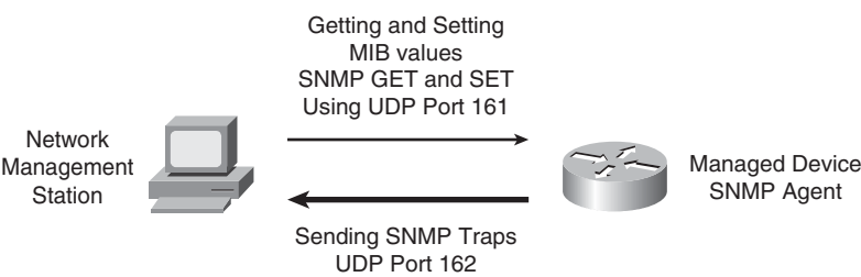
Figure 5-1 SNMP Traffic
