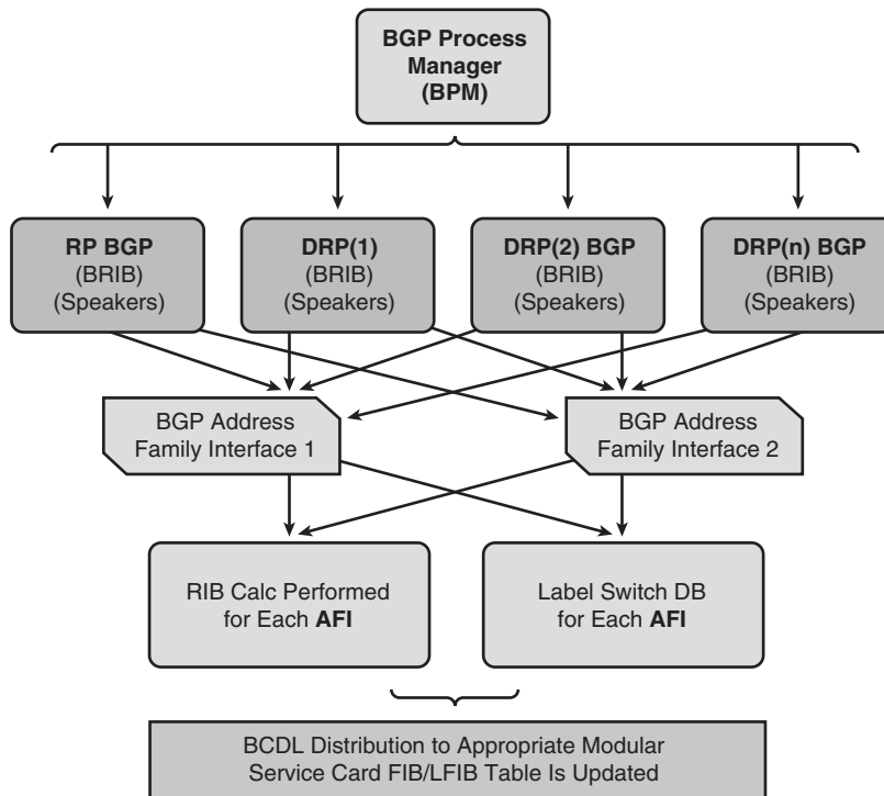
Figure 8-2 Distributed BGP
