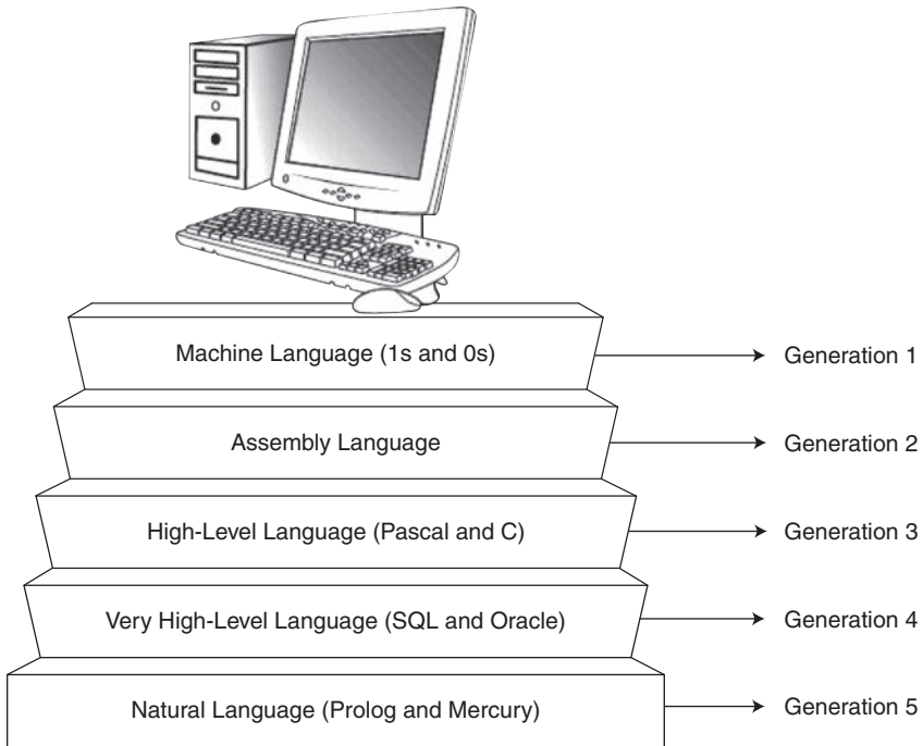
FIGURE 11.5 Programming Languages.
