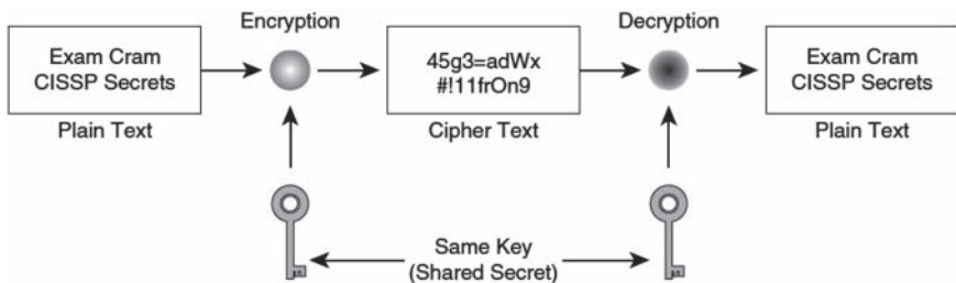
FIGURE 6.4 Symmetric encryption.
