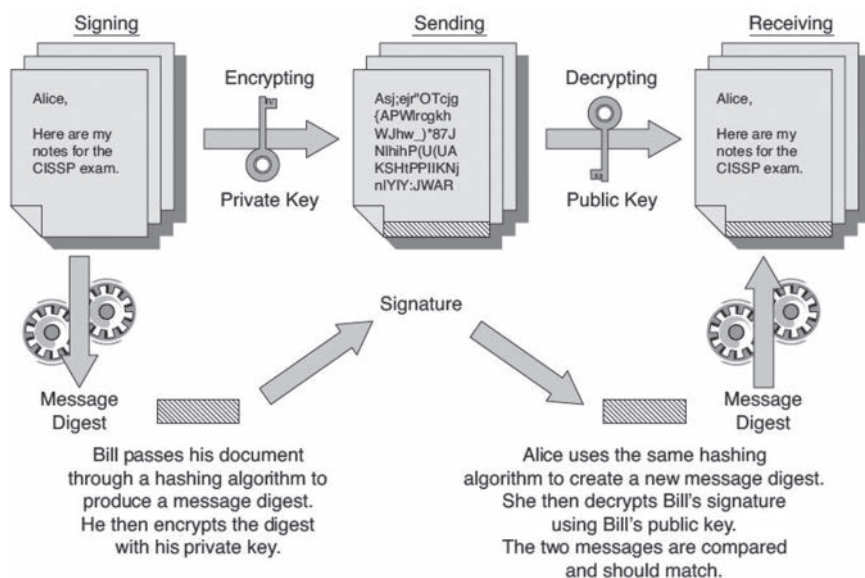
FIGURE 6.12 Digital signatures.
