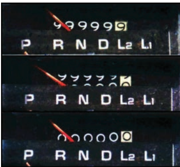
FIGURE 9.2 Integer overflow.
