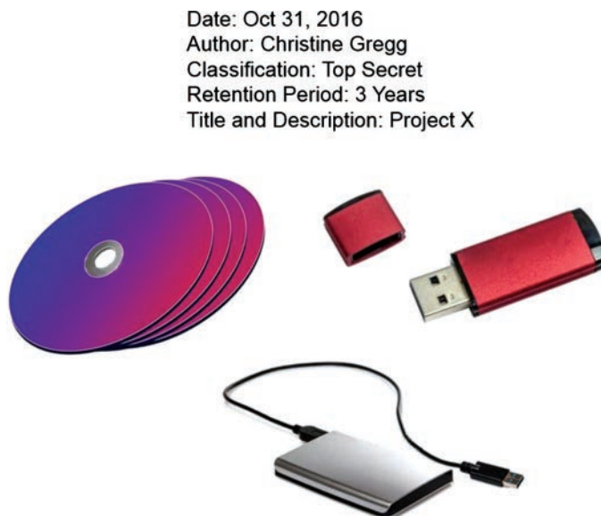
FIGURE 2.3 Data labeling.
