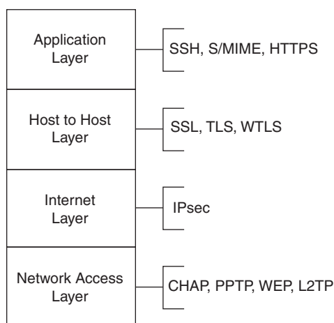
FIGURE 6.14 Layered security controls.
