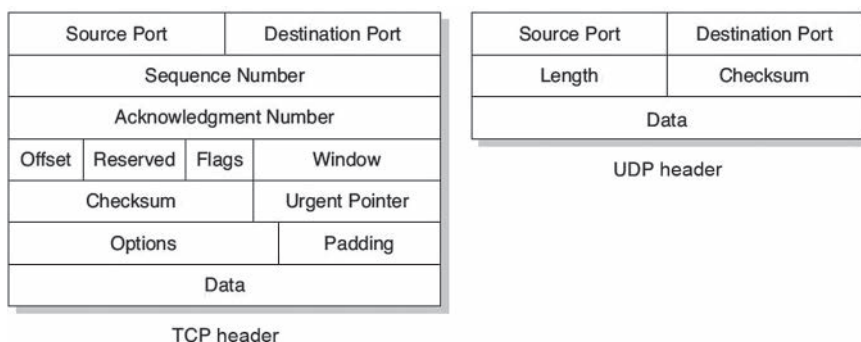
FIGURE 7.4 TCP and UDP header.
