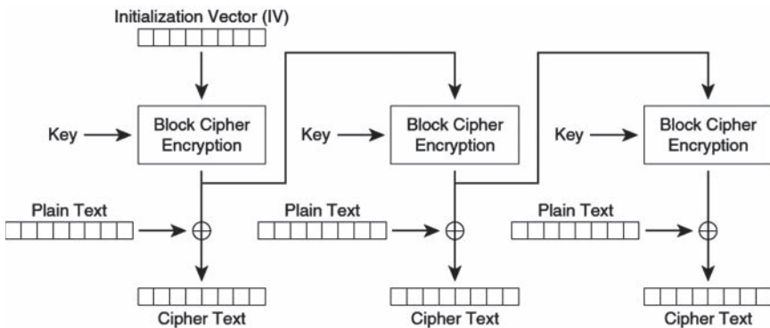
FIGURE 6.6 DES OFB encryption.
