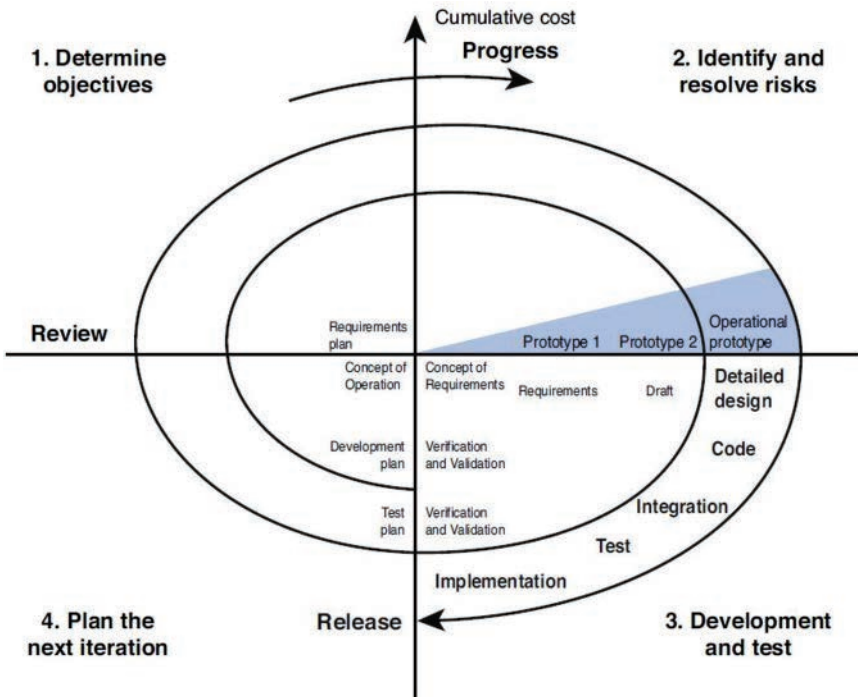
FIGURE 11.3 The Spiral Model.
