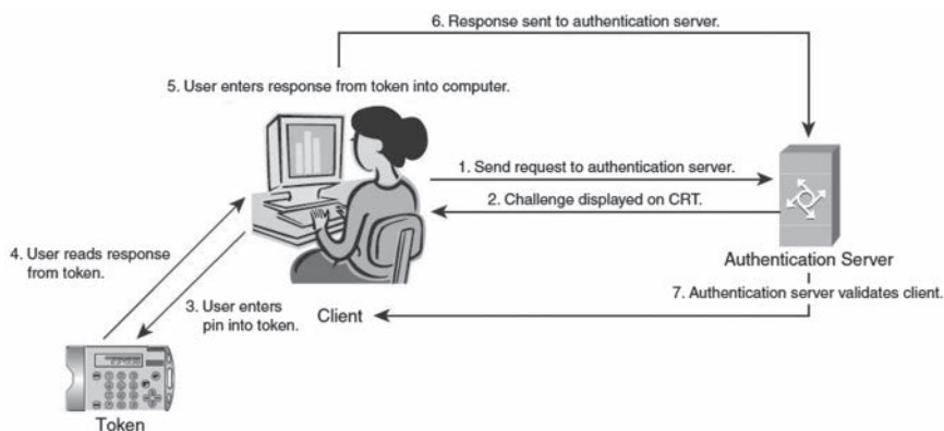
FIGURE 8.2 Asynchronous token authentication.
