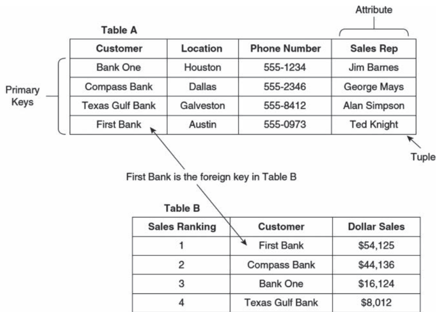
FIGURE 11.6 Primary and Foreign Keys.
