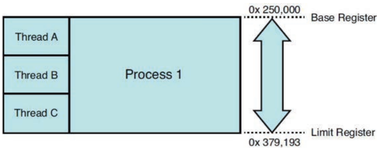
FIGURE 5.1 Processes and threads.
