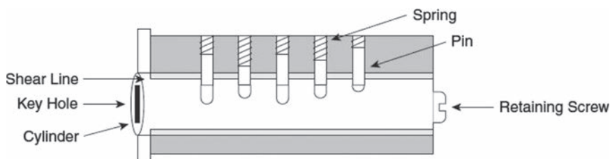
FIGURE 3.3 Tumbler lock design.
