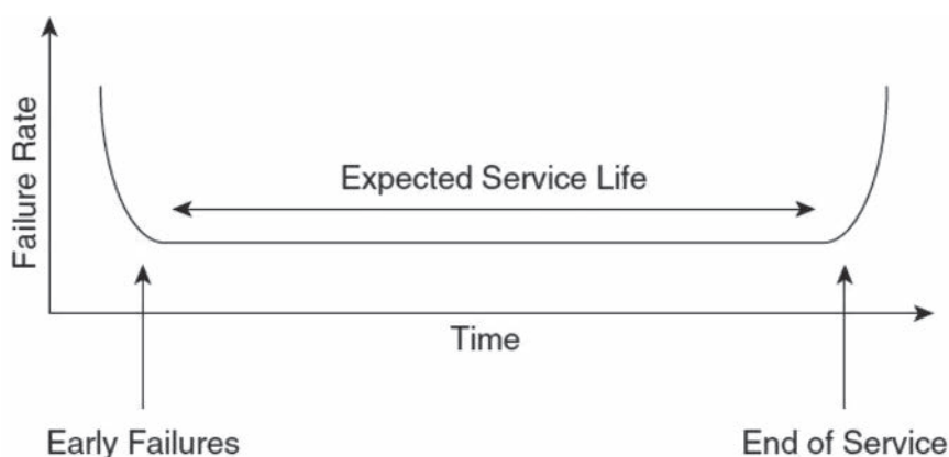
FIGURE 10.3 MTBF and the bathtub curve.
