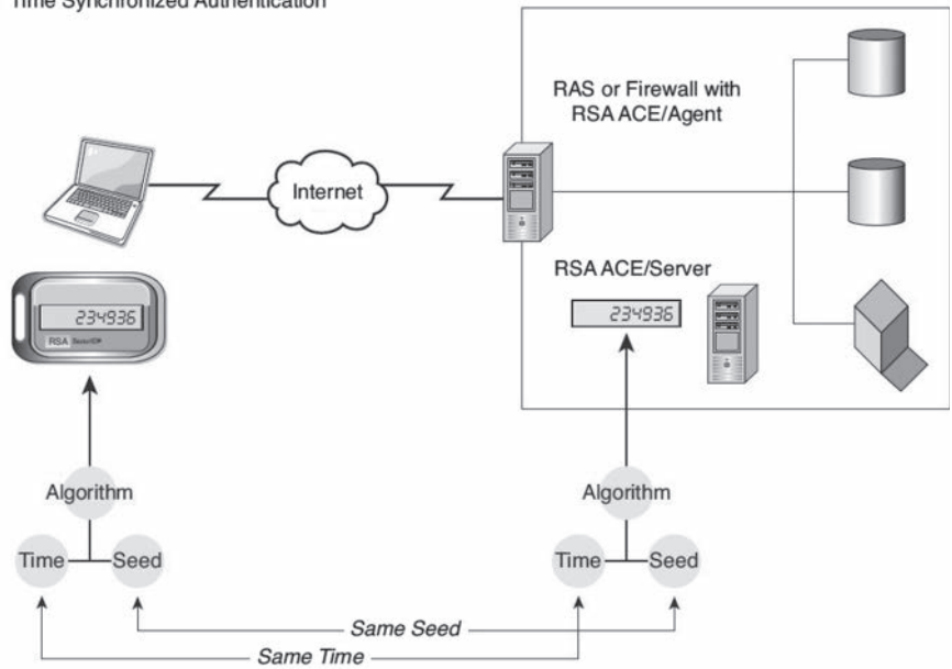
FIGURE 8.1 RSA token authentication.
