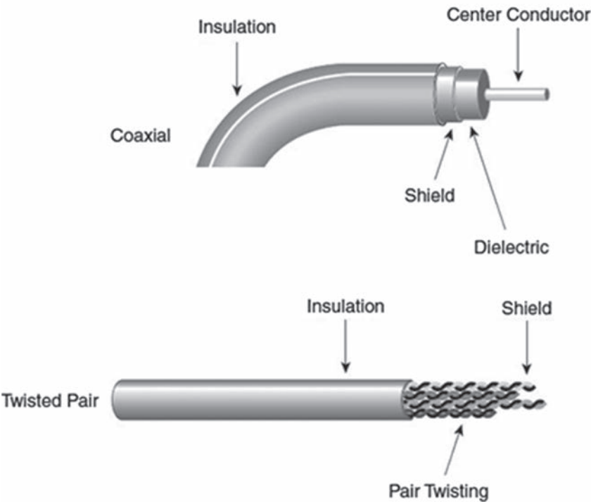
FIGURE 7.11 Coaxial and twisted pair.
