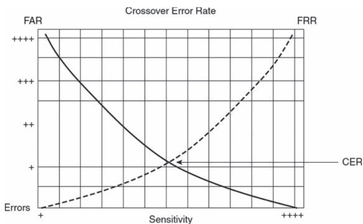
FIGURE 8.4 Crossover error rate.
