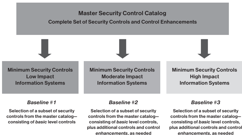
FIGURE 2.4 NIST 800-53 Scoping and Baselining Controls.
