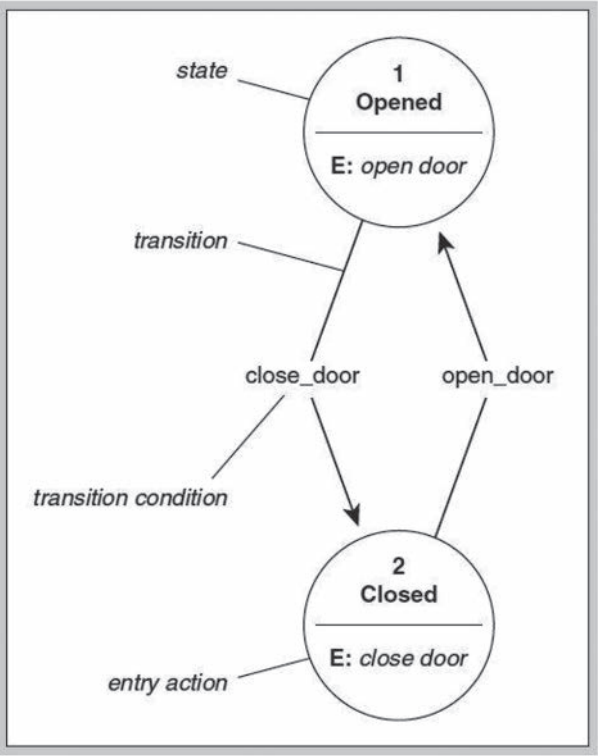
FIGURE 5.6 Finite state model.
