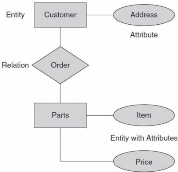
FIGURE 11.1 Entity Relationship Diagram.
