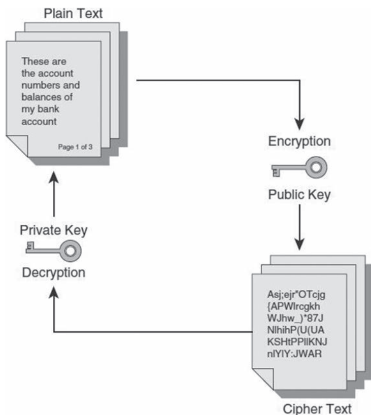
FIGURE 6.9 Asymmetric encryption.
