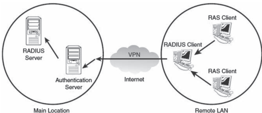
FIGURE 8.8 RADIUS authentication.
