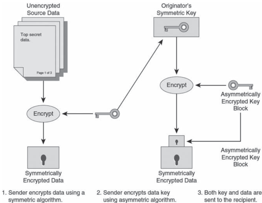
FIGURE 6.10 Hybrid encryption.
