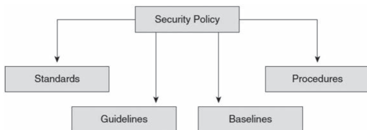
FIGURE 4.8 Policy structure.
