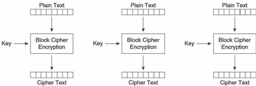
FIGURE 6.5 DES ECB encryption.
