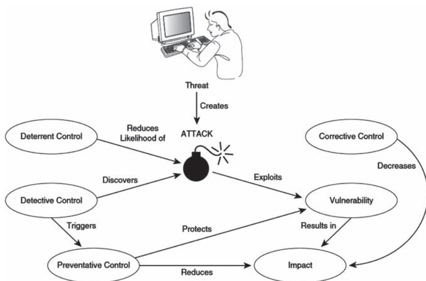
FIGURE 4.6 Threats, vulnerabilities, and controls.
