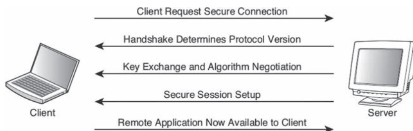
FIGURE 6.15 Secure Sockets Layer (SSL).
