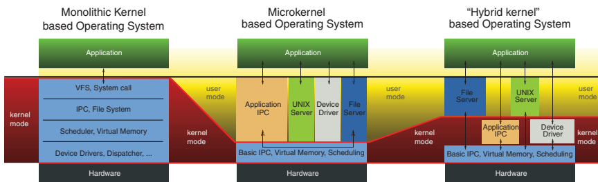
FIGURE 5.4 Operating System Architecture.
