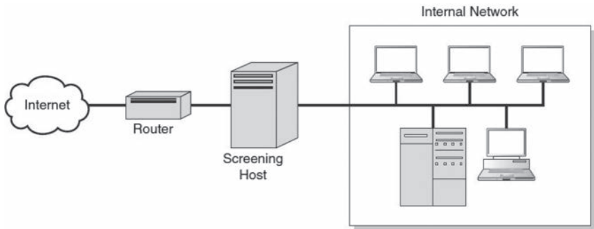
FIGURE 7.15 Screened host.
