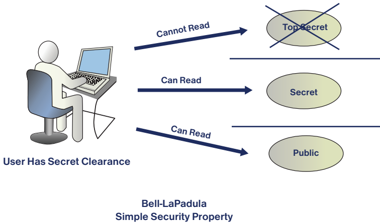
FIGURE 5.7 Bell-LaPadula Simple Security Model.
