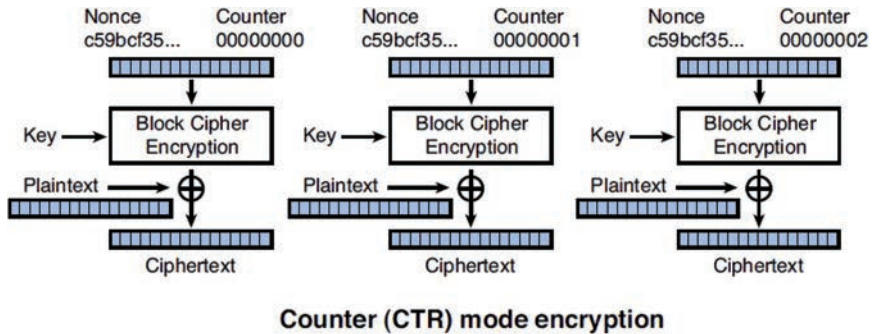
FIGURE 6.7 Counter mode encryption.
