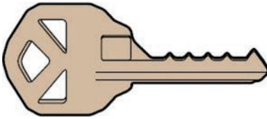
FIGURE 3.4 Key-bumping key.
