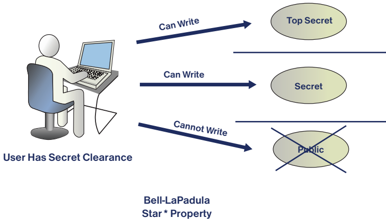
FIGURE 5.8 Bell-LaPadula Star * Property.
