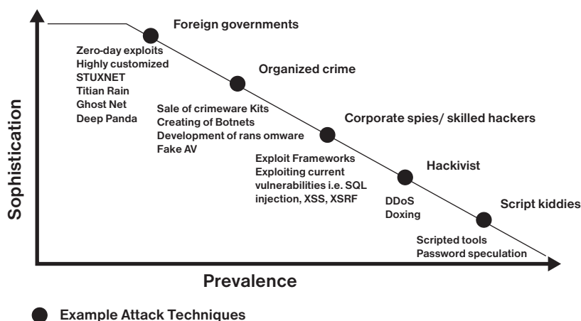
FIGURE 9.3 Threat actors.
