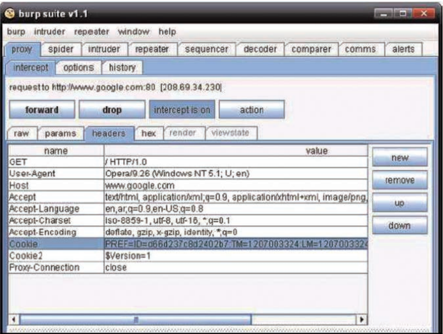
FIGURE 5.12 Burp proxy.
