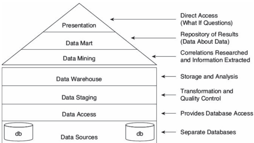
FIGURE 2.2 Data mining.
