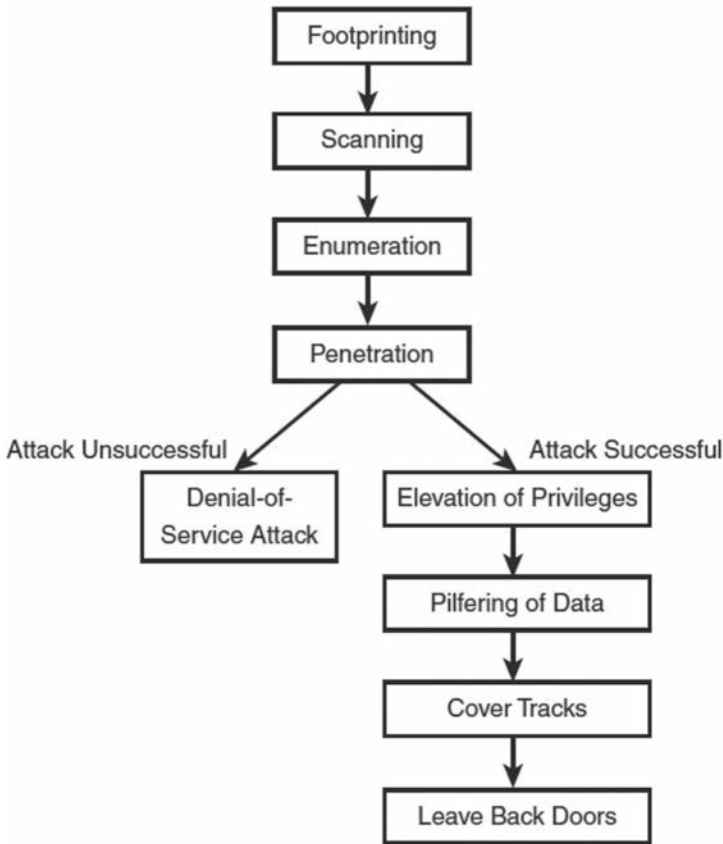
FIGURE 9.4 Attack methodology.
