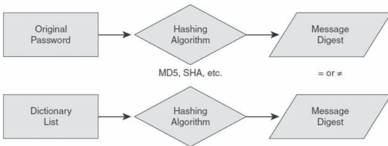
FIGURE 9.8 Password cracking.
