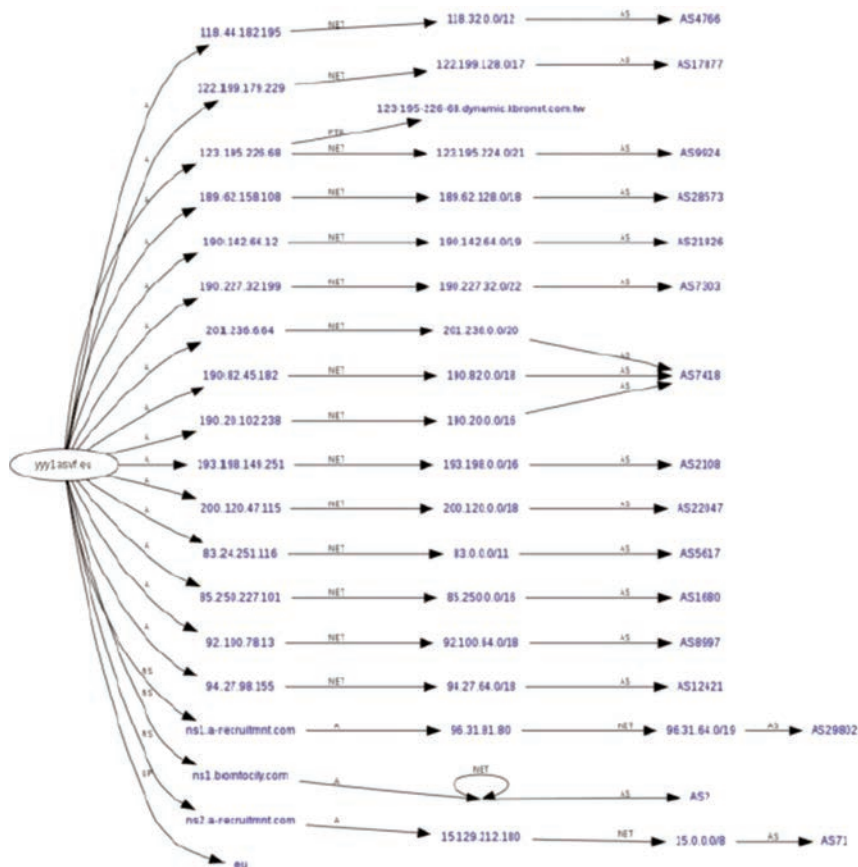
FIGURE 9.7 Fast-flux botnet.
