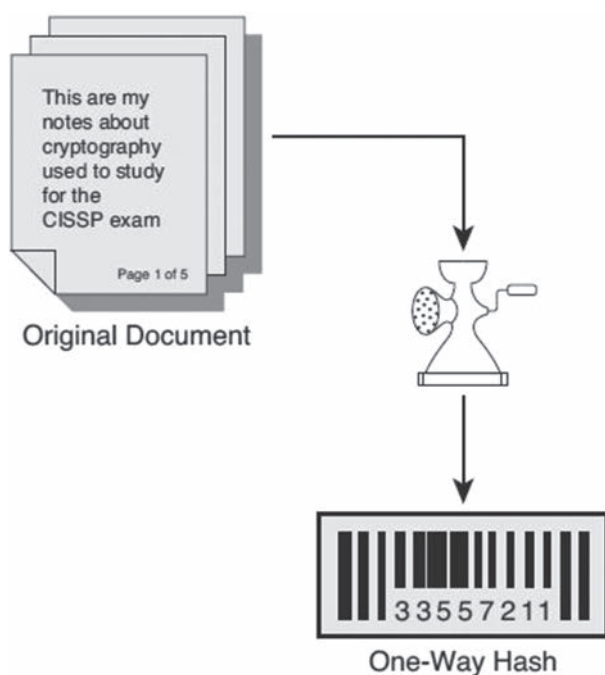
FIGURE 6.11 Hashing.
