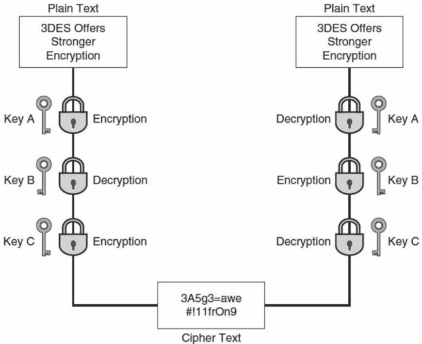
FIGURE 6.8 3DES EDE3.
