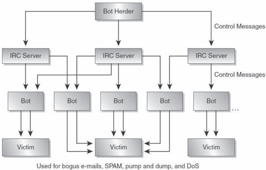
FIGURE 9.6 Botnets.
