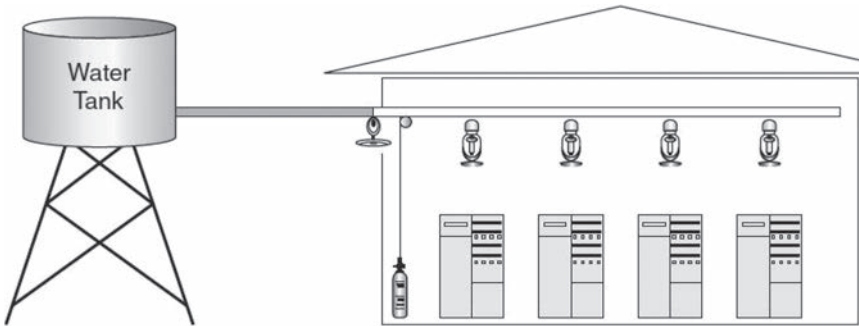
FIGURE 3.6 Dry pipe fire suppression system.
