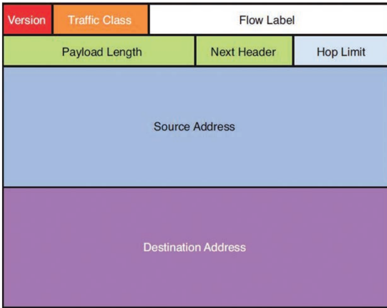
FIGURE 7.3 IPv6 header.
