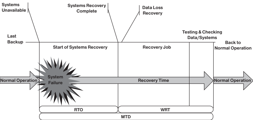
FIGURE 12.6 MTD, RTO, and WRT.
