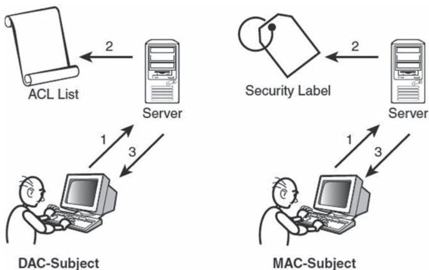
FIGURE 8.7 Differences between DAC and MAC.
