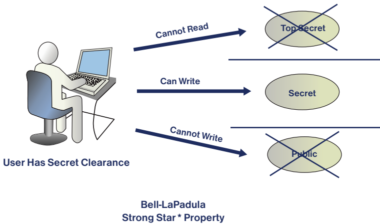
FIGURE 5.9 Bell-LaPadula Strong Star Property.
