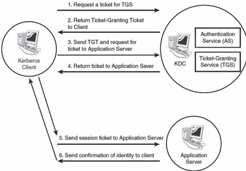
FIGURE 8.6 Kerberos operation.
