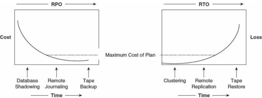
FIGURE 12.5 RPO and RTO.
