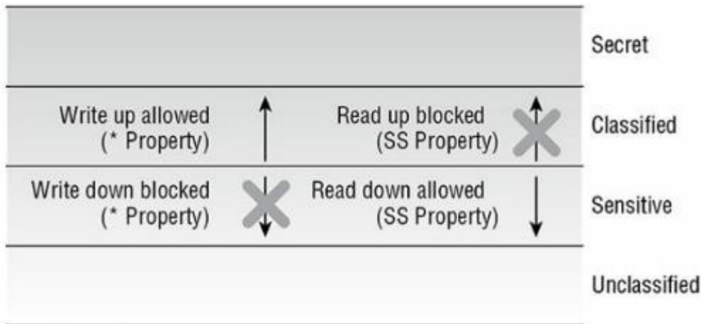
FIGURE 8.3 The Bell-LaPadula model
