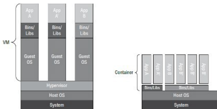
FIGURE 9.4 Application containers versus a hypervisor
