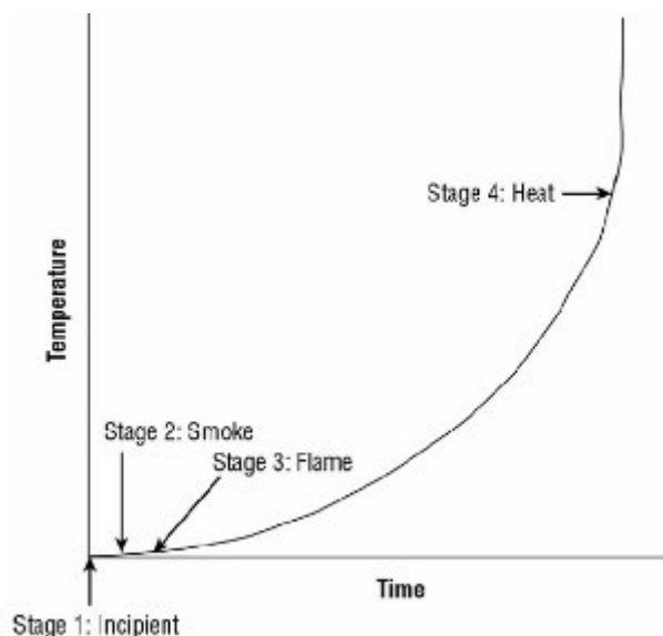
FIGURE 10.3 The four primary stages of fire
