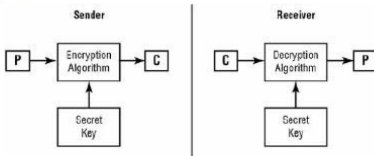
FIGURE 6.3 Symmetric key cryptography
