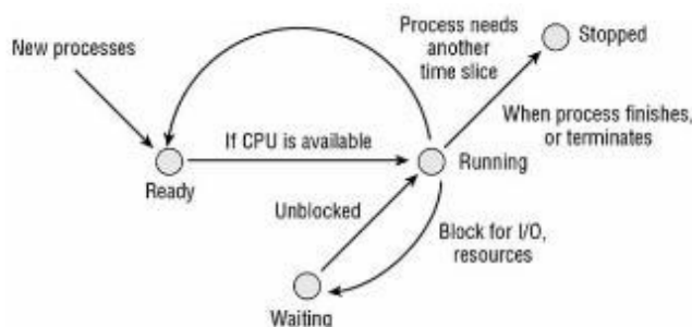
FIGURE 9.2 The process scheduler
