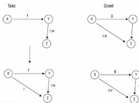
FIGURE 8.2 The Take-Grant model's directed graph
