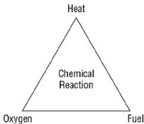
FIGURE 10.2 The fire triangle
