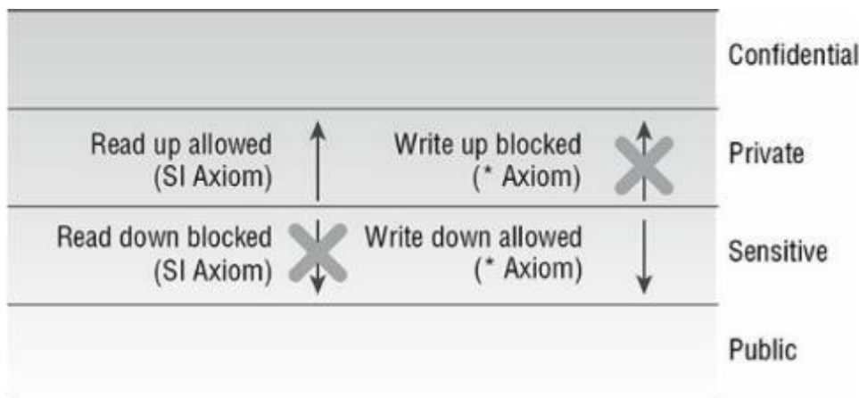
FIGURE 8.4 The Biba model
