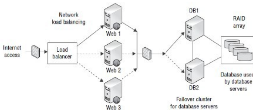
FIGURE 18.3 Failover cluster with network load balancing
