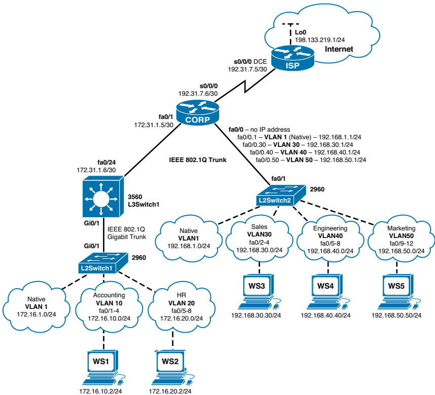
Figure 11-1 Network Topology for Inter-VLAN Communication Configuration
