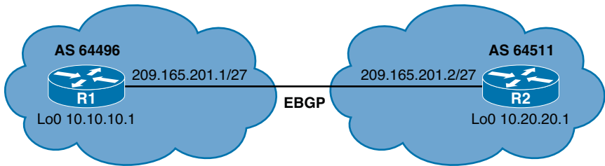
Figure 6-10 eBGP Multihop
