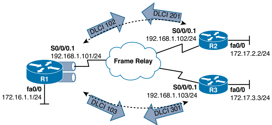
Figure 2-3 Network Topology for EIGRP over Frame Relay Using Multipoint Subinterfaces
