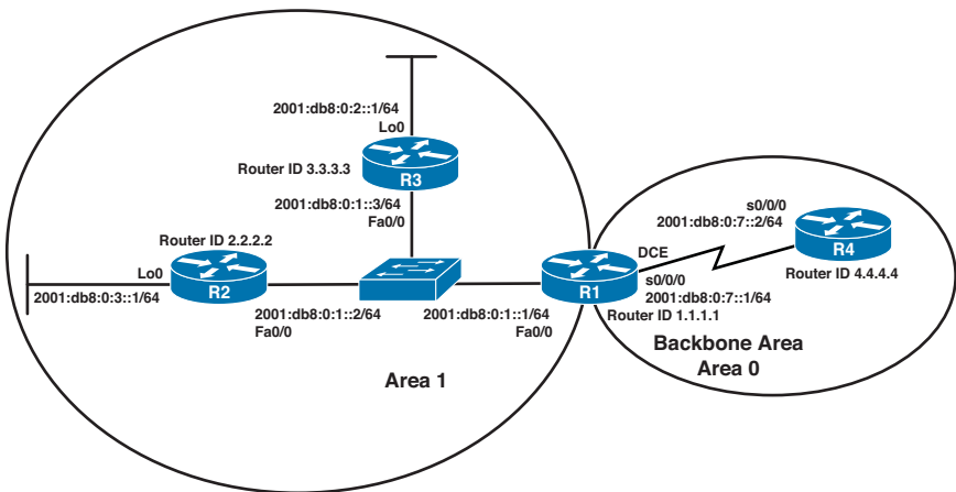
Figure 3-8 Network Topology for IPv6 and OSPFv3 Configuration
