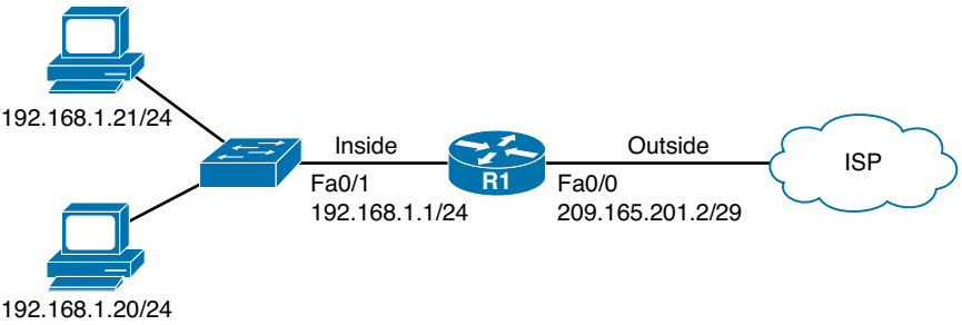
Figure 6-3 Configuring Dynamic NAT
