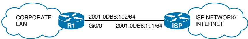
Figure 6-6 Configure Basic IPv6 Connectivity
