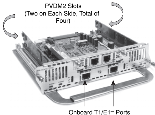
Figure 1-8 Network Module with PVDMs
