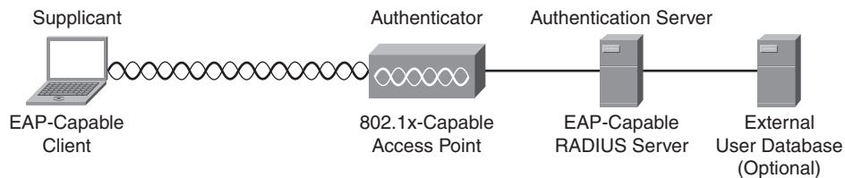
Figure 9-1 802.1x (EAP) Authentication Components
