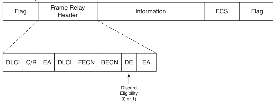
Figure 3-2 DE Field on Frame Relay Frame Header
