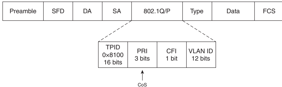
Figure 3-1 802.1Q/P Field
