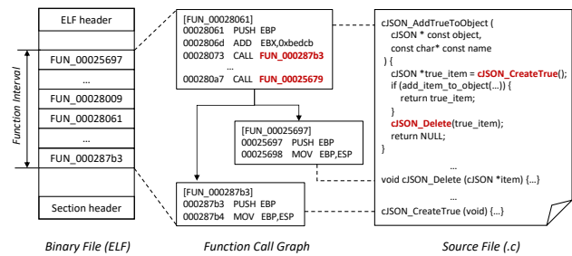
Figure 4: Function matching between source and binary files
