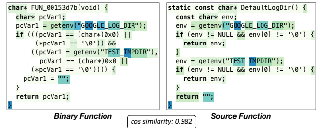
Figure 3: Retrieved binary and source function pair
