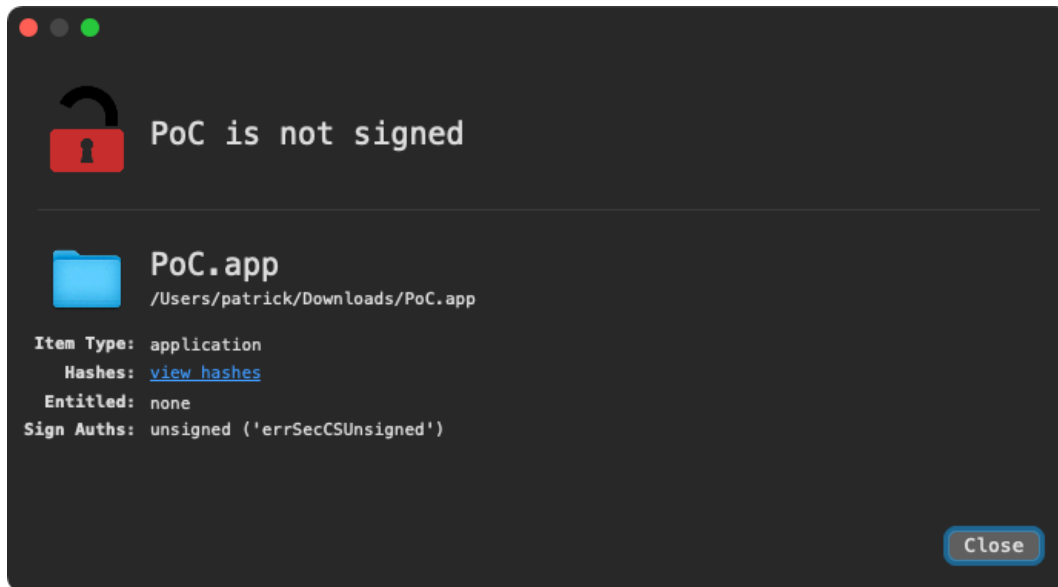
PoC.app: unsigned/unnotarized
