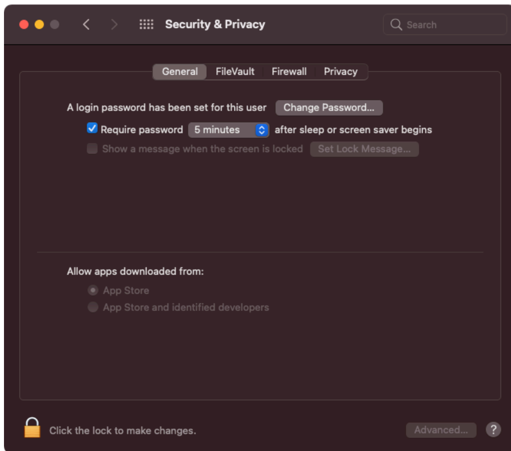
Application policy
