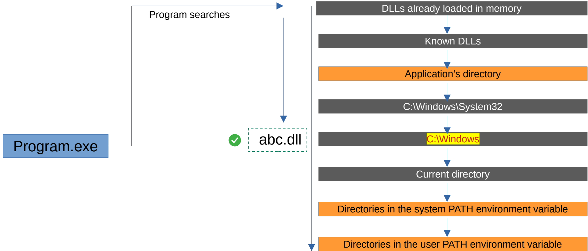
DLL search order in windows
