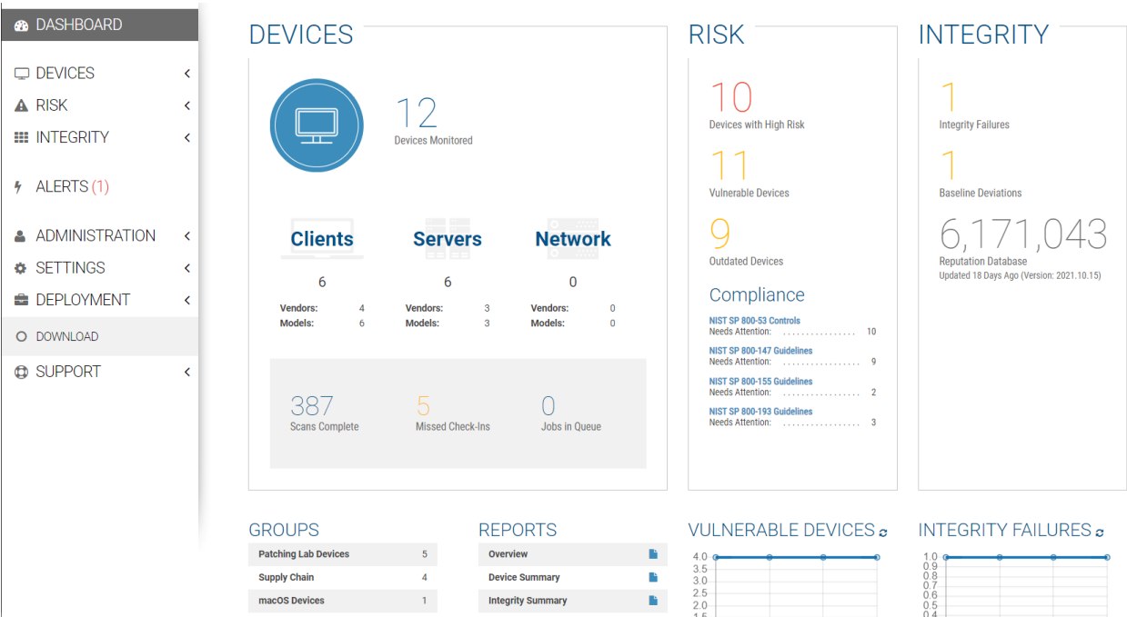
836 Figure 3-1 Eclypsium Main Dashboard
