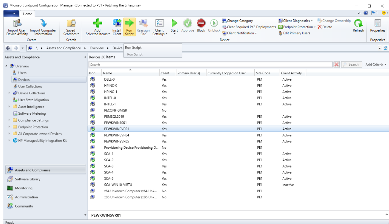
Figure 6-5 Devices View with Run Script Option Selected
