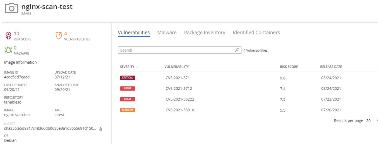
Figure 2-7 Example of Container Vulnerability Information
