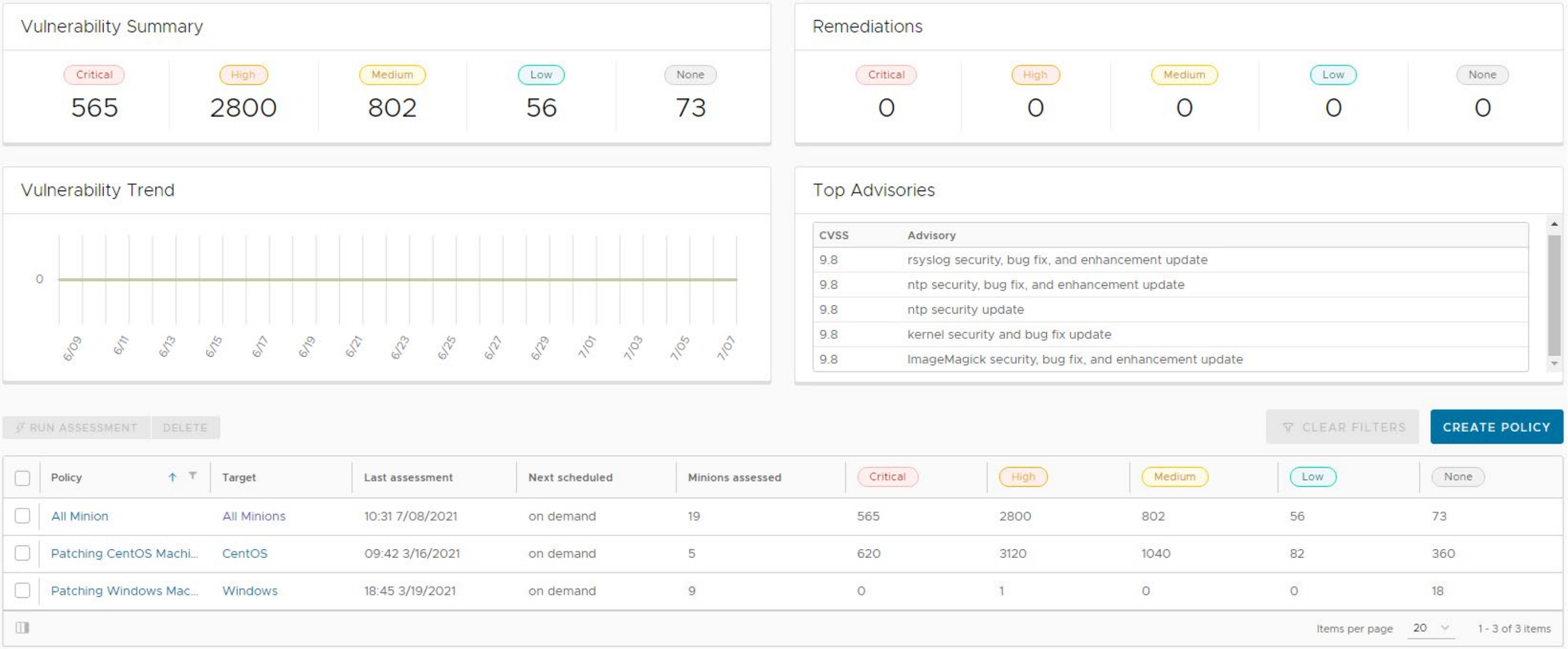
966 Figure 4-1 SaltStack SecOps Vulnerability Summary and Top Advisories Dashboard
