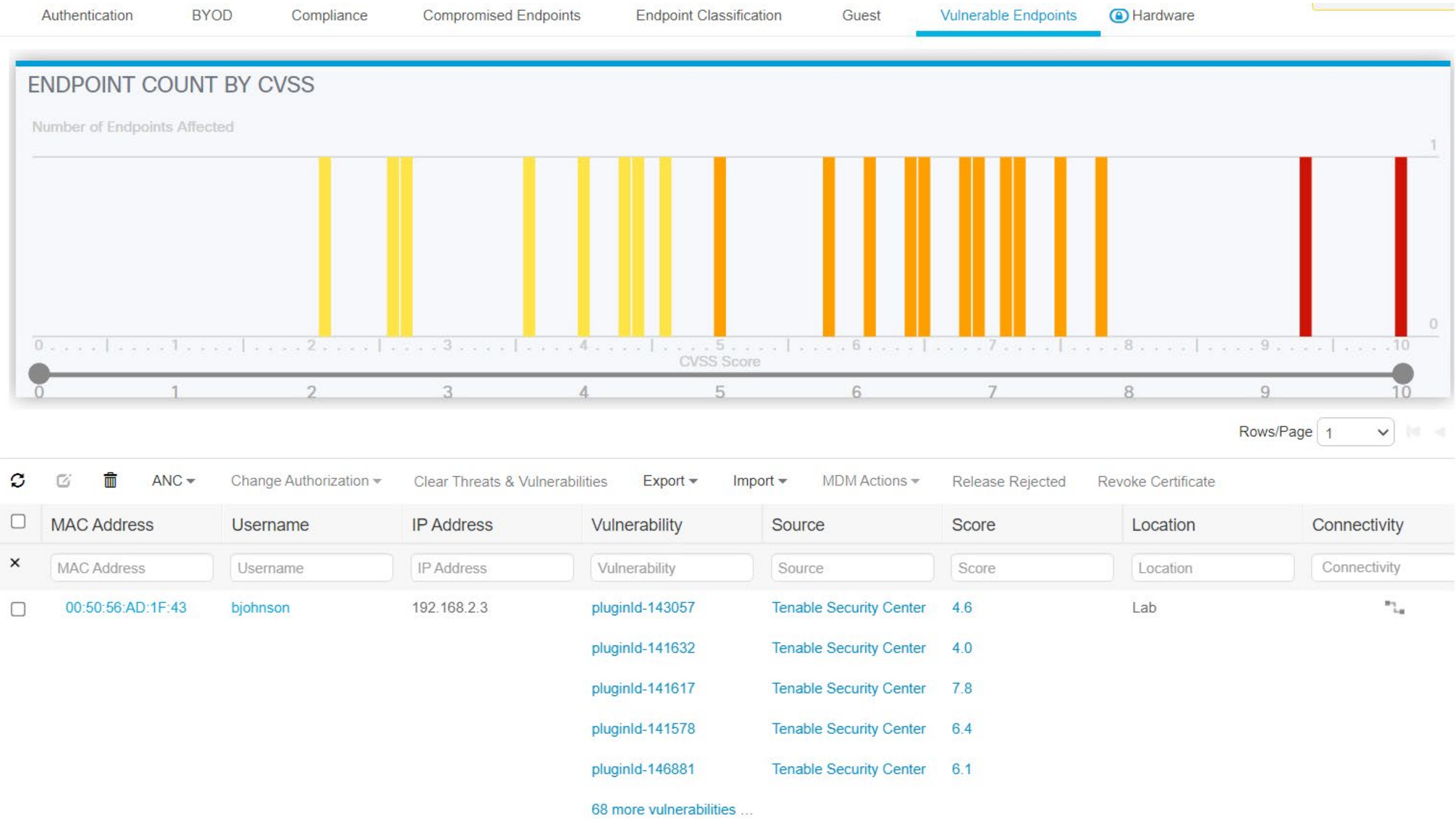
1142 Figure 5-1 Cisco ISE View of Vulnerability Data for Connected Devices
