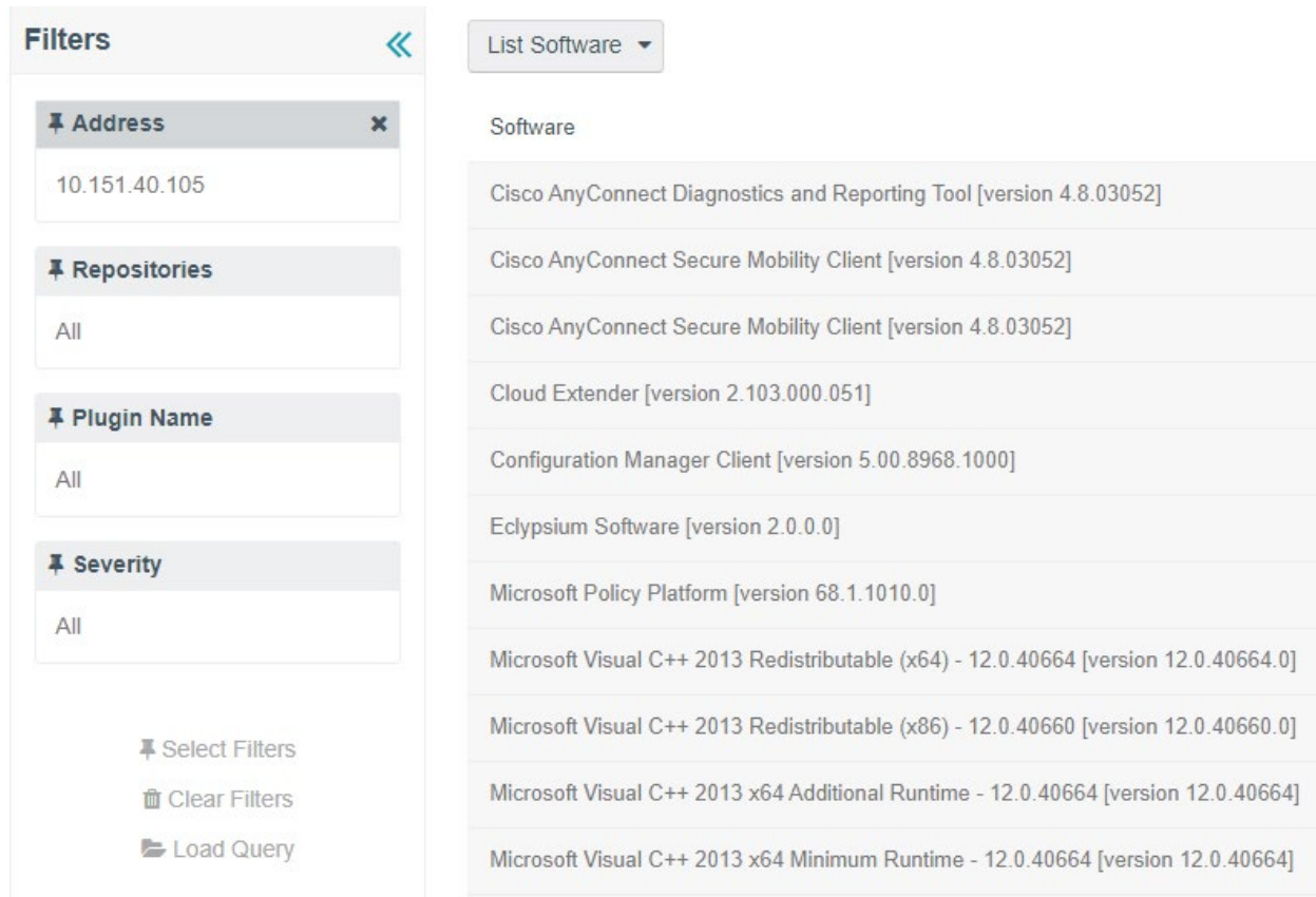
667 Figure 2-2 Applying Filters to Scan Results
