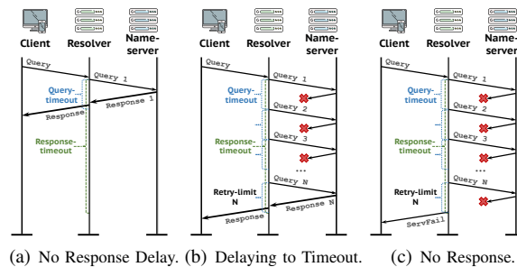
Figure 4. DNS Resolution under the DNS Timeout Mechanism.
