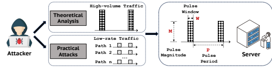
Figure 1. Concept of the Pulsing DoS Attack.
