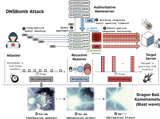
Figure 3. Threat Model of the DNSBOMB Attack.
