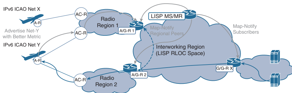
Figure 7-14 Multihoming and Mobility in the Aeronautical Telecommunications Network Using LISP
