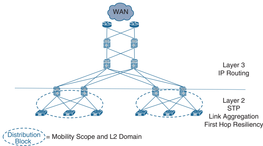
Figure 5-1 Standard Layer 2 Access Network Design
