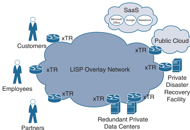
Figure 3-12 LISP Hybrid Cloud Connectivity
