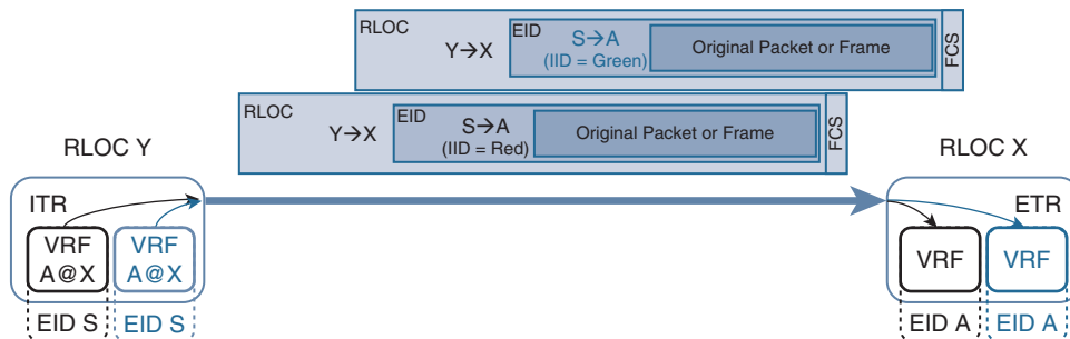
Figure 6-5 Virtual Network Data Plane Segmentation
