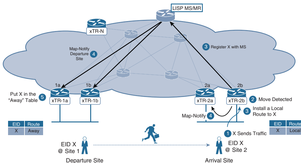
Figure 7-2 LISP EID Mobility Convergence
