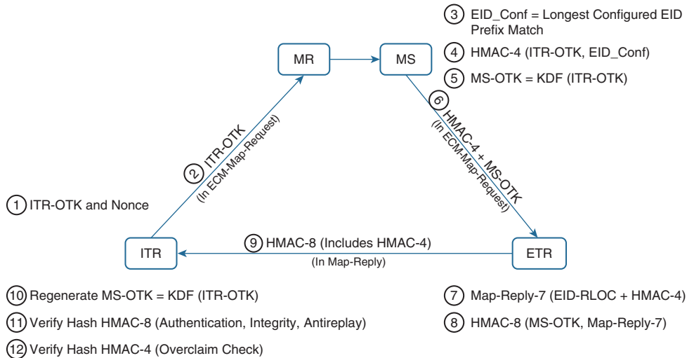
Figure 6-12 A Detailed View of LISP-SEC
