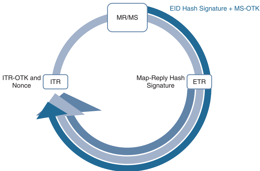
Figure 6-11 A High-Level View of LISP-SEC
