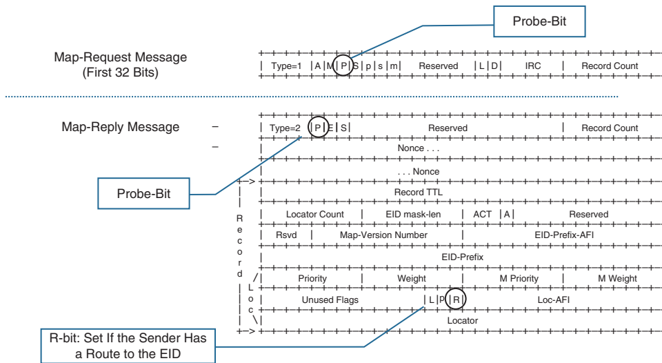
Figure 2-10 LISP Message Fields Relevant to RLOC Probes
