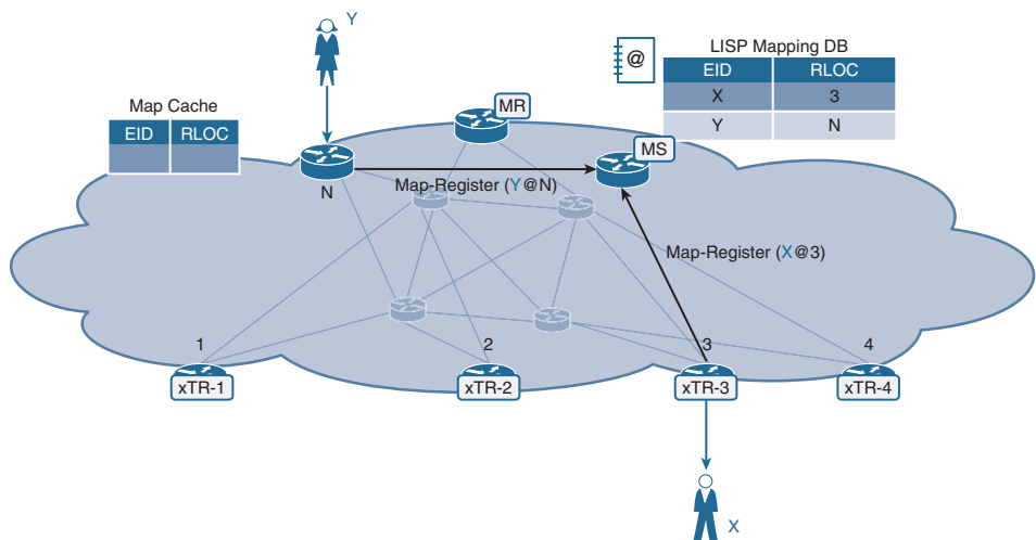
Figure 2-4 Registration of EID to RLOC Mappings
