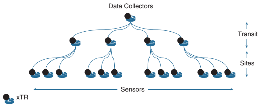
Figure 5-14 LISP Hierarchical Sensor Network Design
