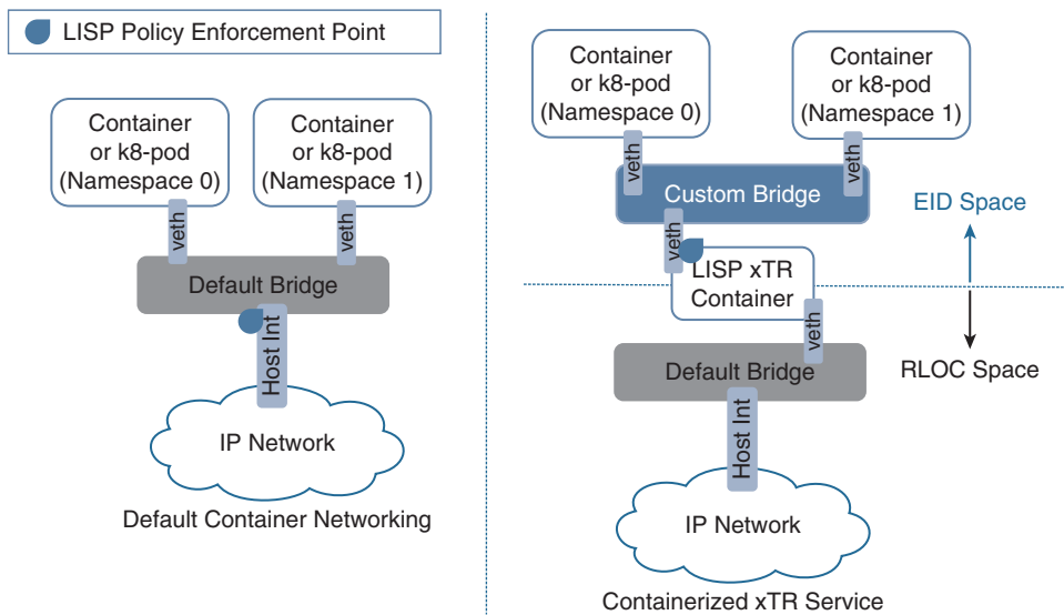
Figure 6-6 Containerized LISP xTR as Default Gateway on Logical Bridge
