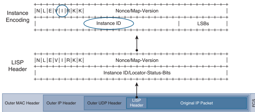
Figure 2-8 LISP Header with Instance-ID
