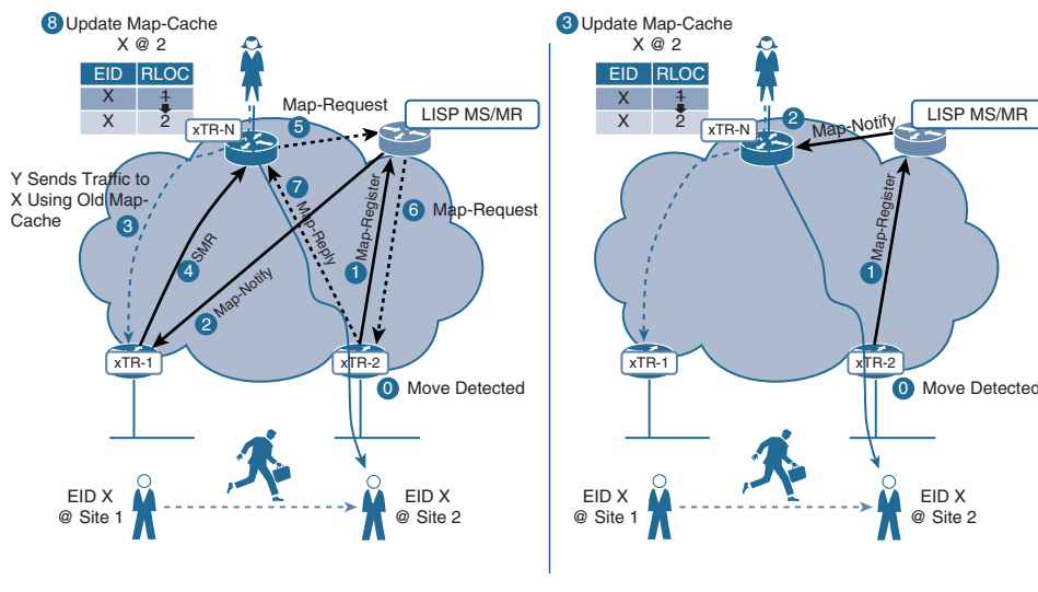
Figure 7-10 Message Reduction and Signaling Delay in EID Mobility
