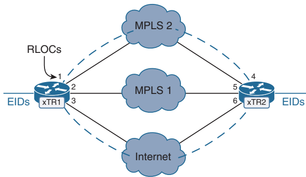
Figure 4-2 An Overlay-Enabled Hybrid WAN
