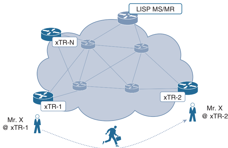
Figure 7-1 LISP EID Mobility
