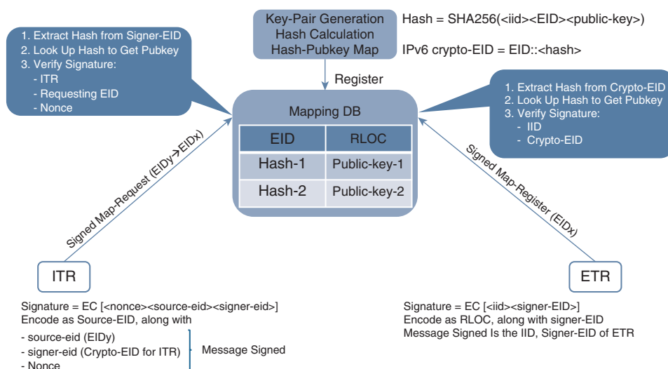
Figure 6-13 LISP ECDSA Authentication and Authorization
