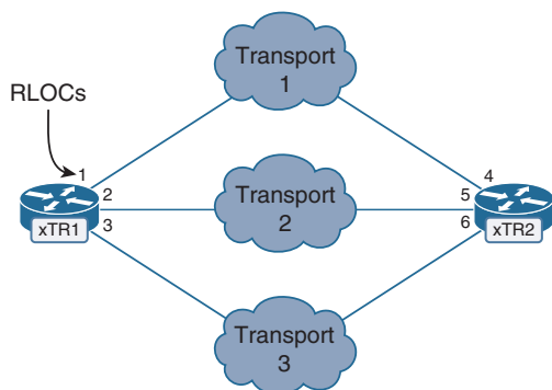
Figure 4-4 Connecting an xTR to Different WAN Transports
