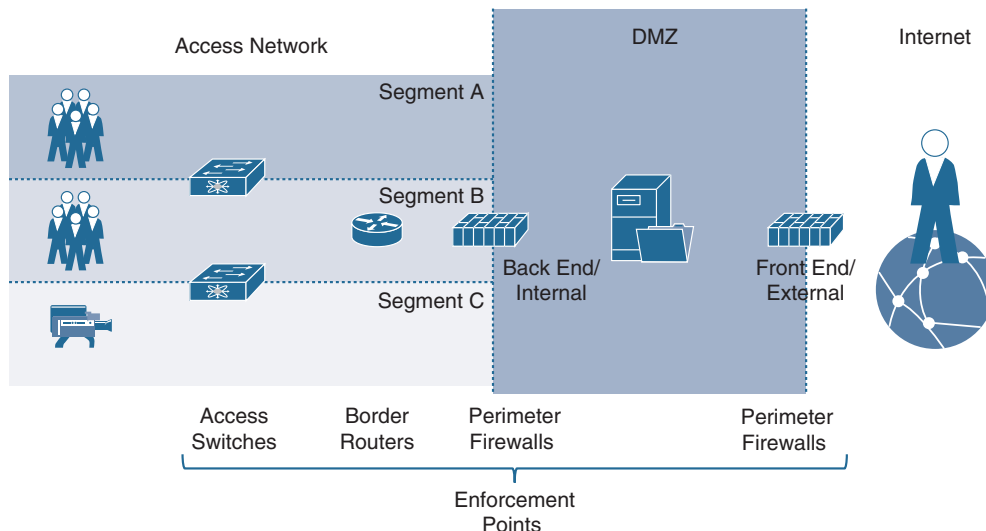
Figure 6-2 Security Enforcement Points in the Virtualized Network Perimeter
