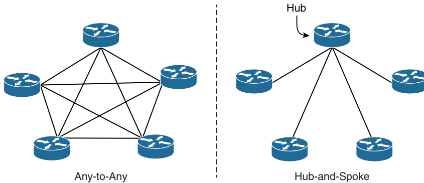
Figure 4-6 WAN Distribution Scenarios
