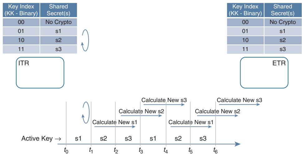
Figure 6-9 LISP Cryptography Data Plane and Rekeying
