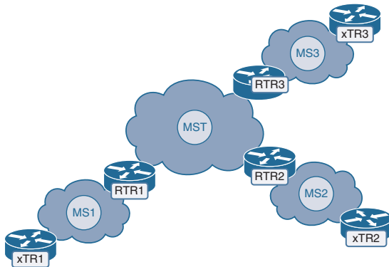
Figure 4-10 LISP Multisite Federated Network
