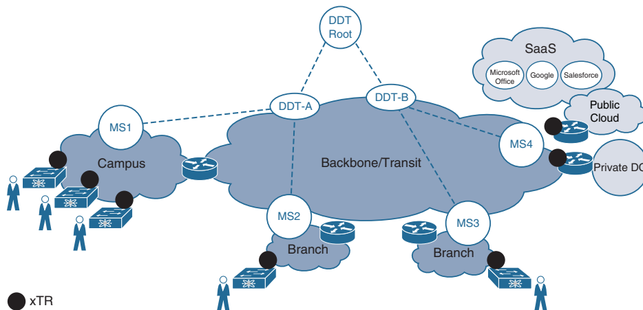
Figure 4-9 LISP Multisite with a DDT Mapping Database System
