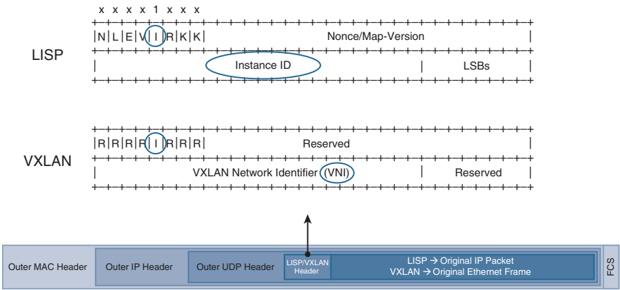
Figure 2-11 LISP and VXLAN Headers Compared
