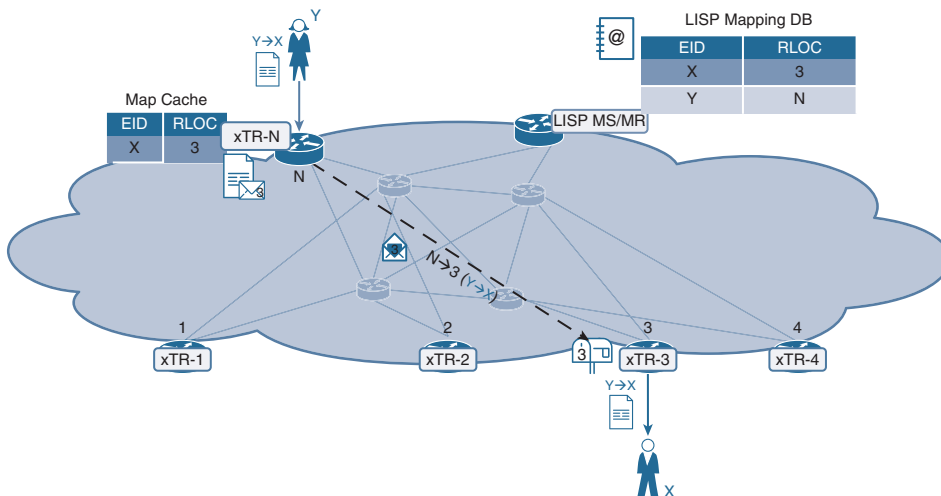
Figure 2-3 Location Resolution on Demand
