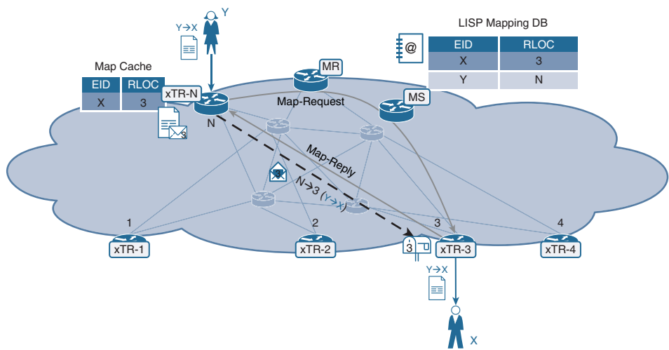
Figure 2-5 Mapping Resolution
