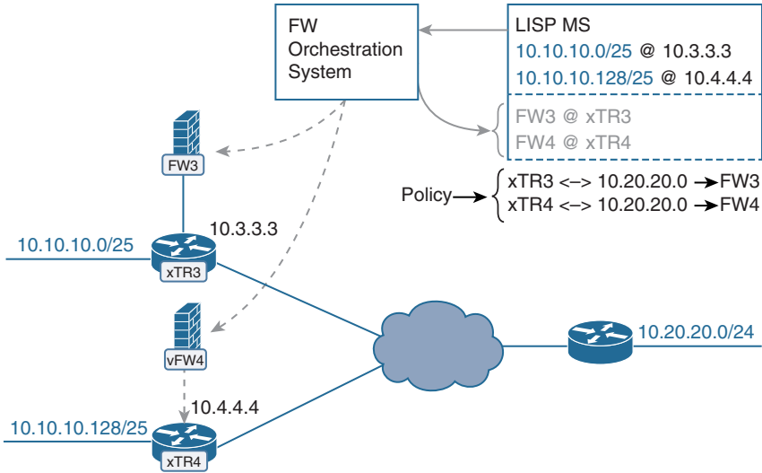
Figure 4-7 Service Insertion Workflow
