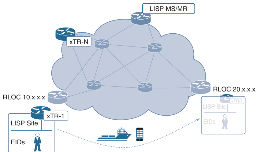
Figure 7-4 LISP Mobile Node
