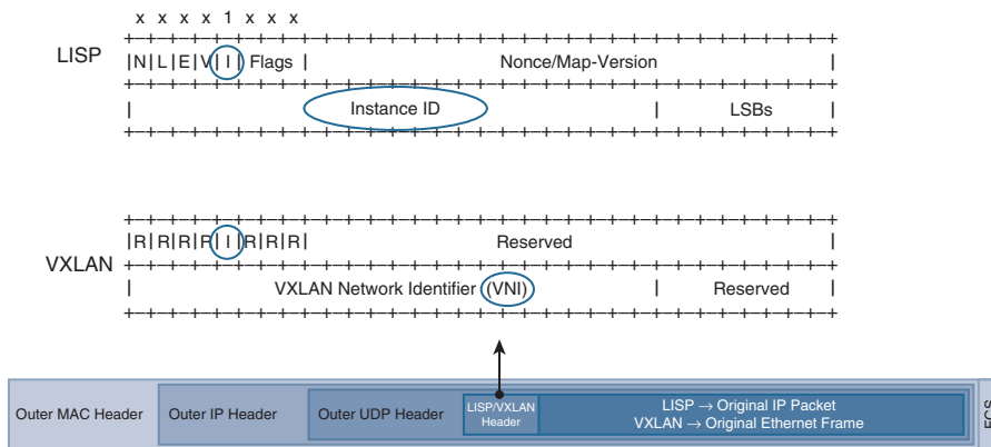
Figure 3-8 L2-LISP and VXLAN Headers
