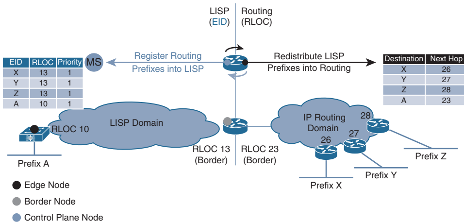
Figure 5-6 Route to EID Redistribution at the LISP Domain Border
