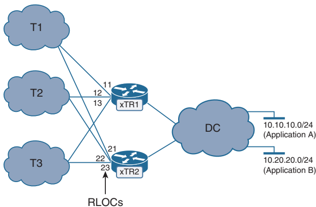
Figure 4-5 Applications in a Multihomed Data Center
