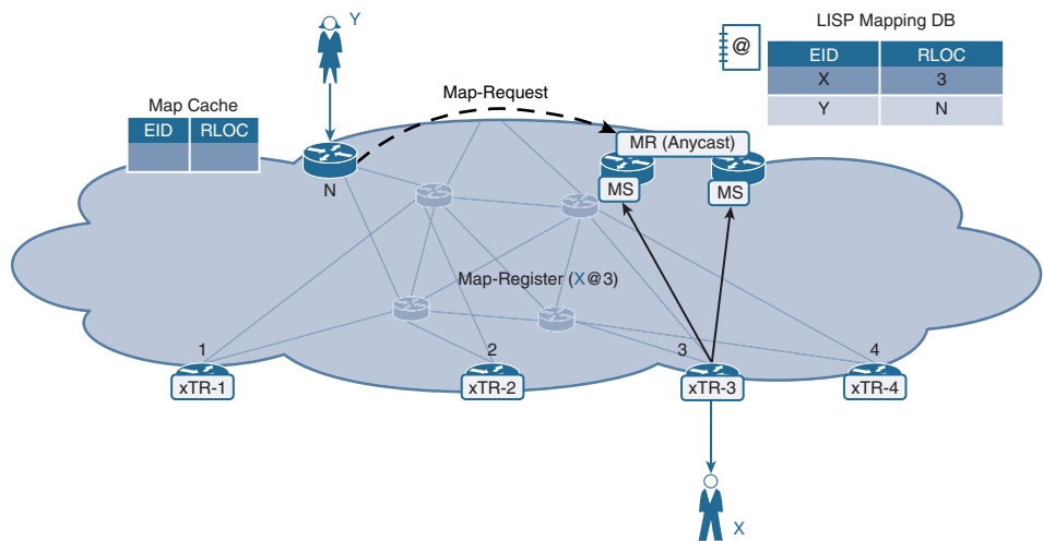
Figure 2-6 Map-Server/Map-Resolver Resiliency
