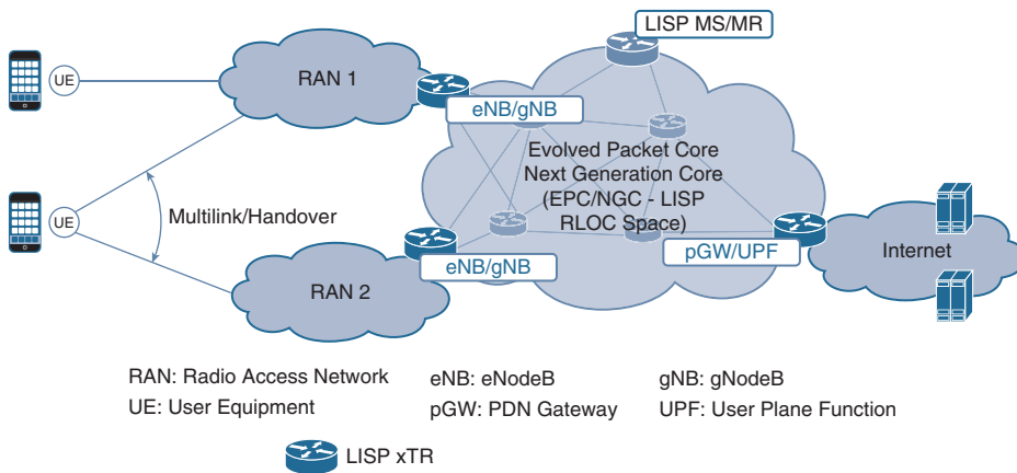
Figure 7-15 LTE/5G Mobile Network Architecture
