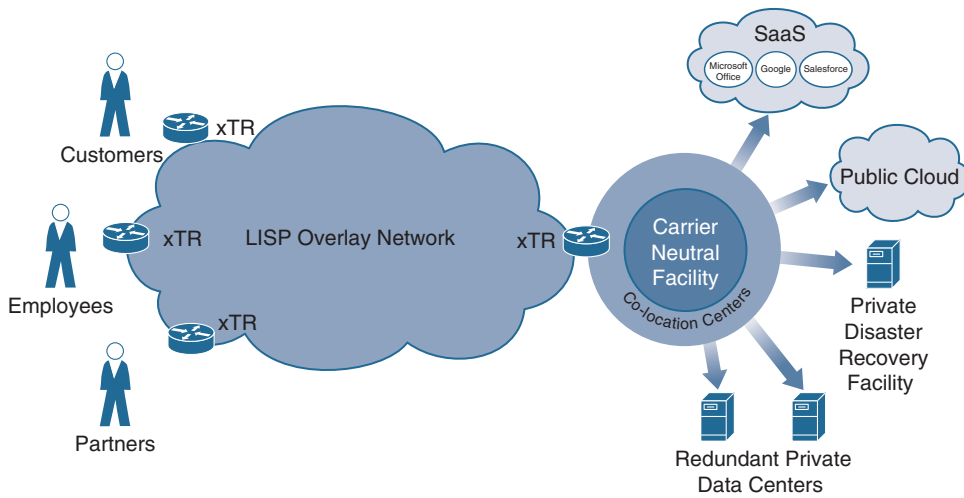
Figure 3-11 LISP Connectivity to Cloud Neutral Facilities
