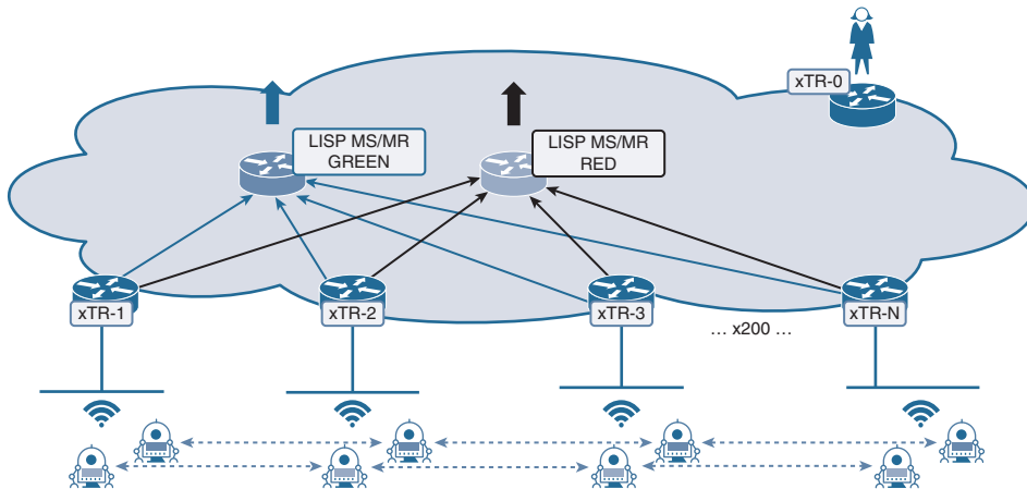
Figure 7-11 Horizontal Scaling of the Control Plane with LISP Delegated Database Tree (DDT)
