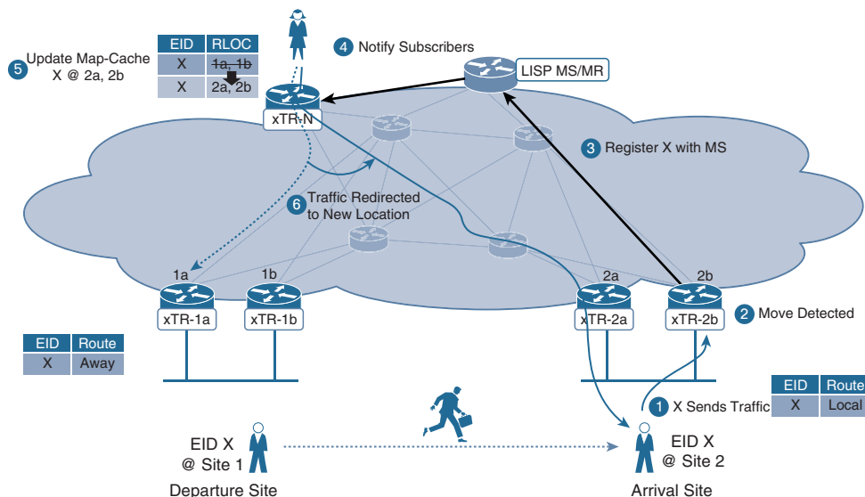
Figure 7-6 Pub-Sub-Enabled LISP EID Mobility
