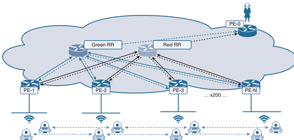
Figure 7-12 Horizontal Scaling of Control Plane Elements in Push Protocols
