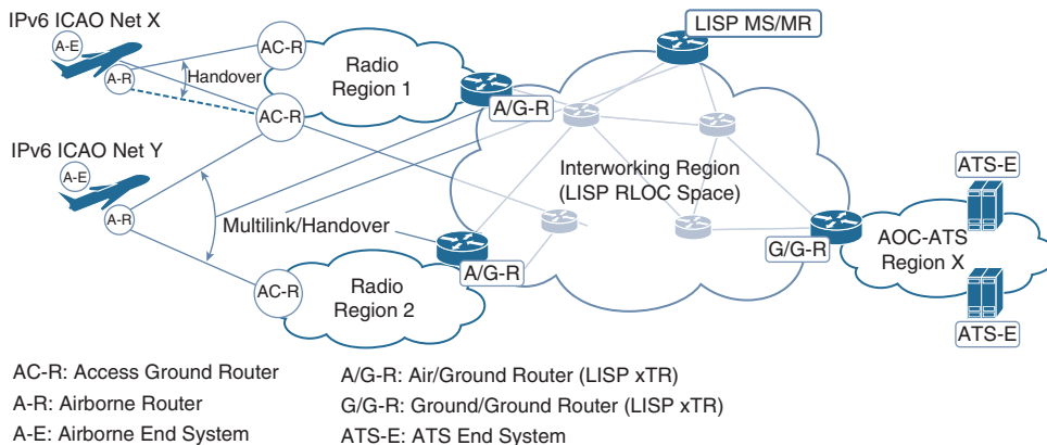
Figure 5-9 LISP-Based Ground Network
