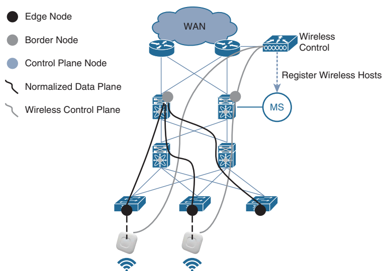
Figure 5-8 Integrated Wired and Wireless
