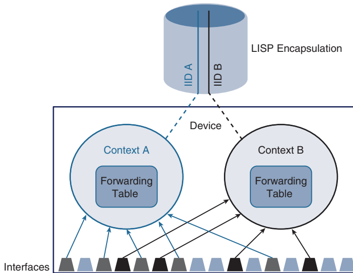
Figure 3-10 Forwarding Contexts
