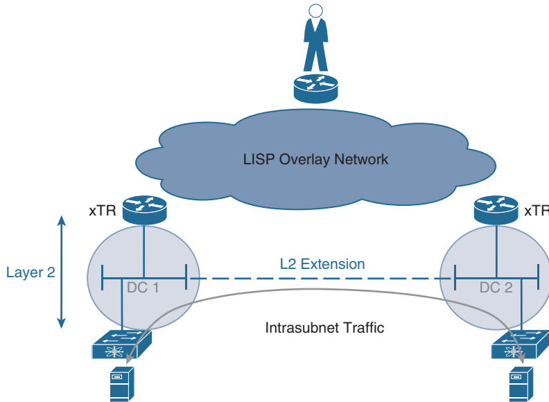
Figure 3-7 Mobility and L2 Extensions
