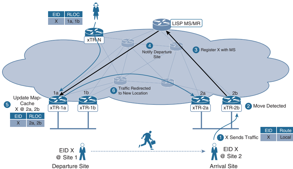
Figure 7-5 LISP Traffic Redirection to Assist Convergence
