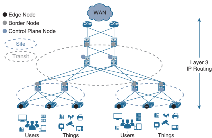
Figure 5-4 Multidomain Access Network Design
