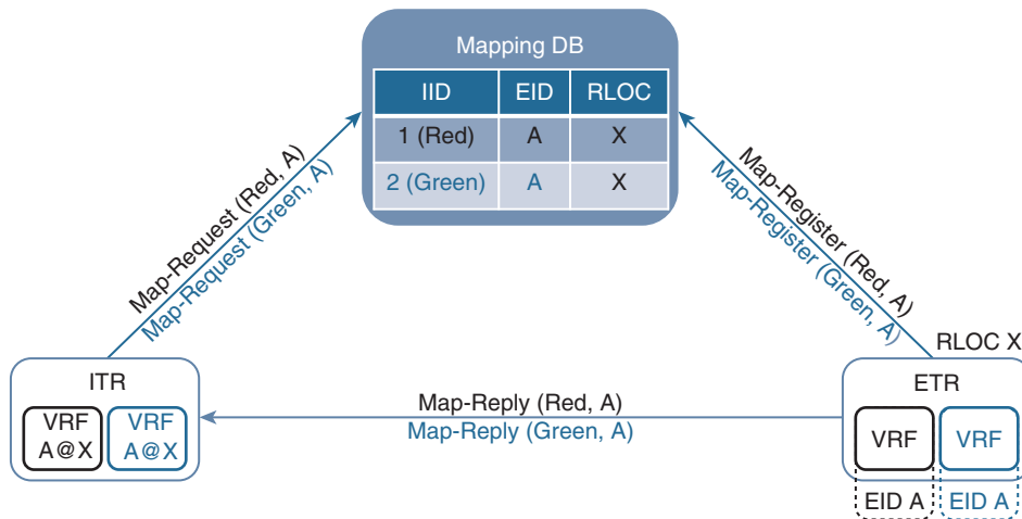
Figure 6-4 Virtual Network Control Plane Segmentation
