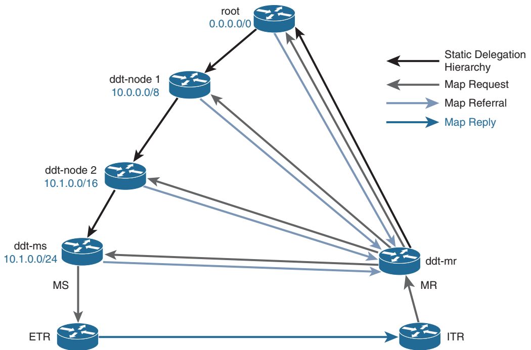
Figure 2-7 Delegated Database Tree (DDT)
