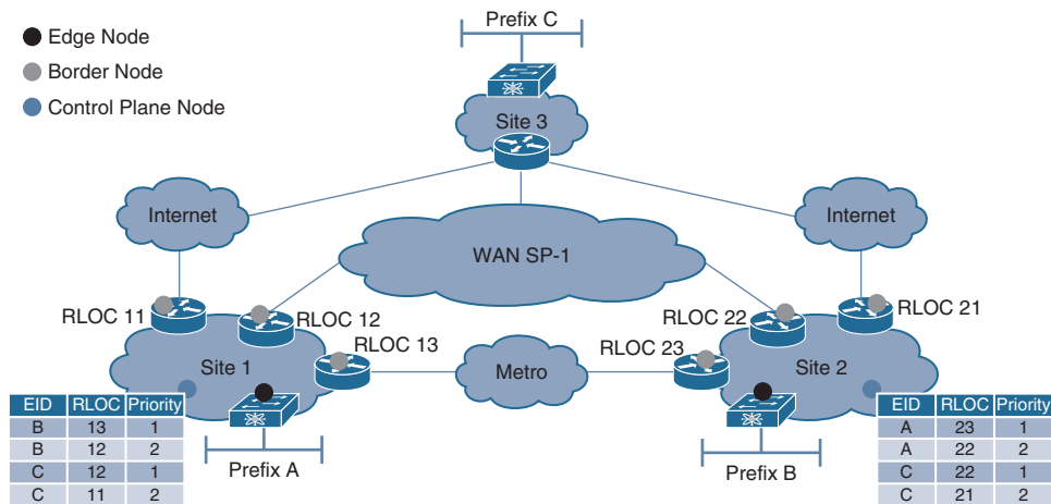
Figure 5-5 External Connectivity for the LISP Access Network
