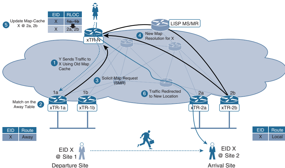
Figure 7-3 LISP EID Mobility Data-Driven Map-Cache Refresh
