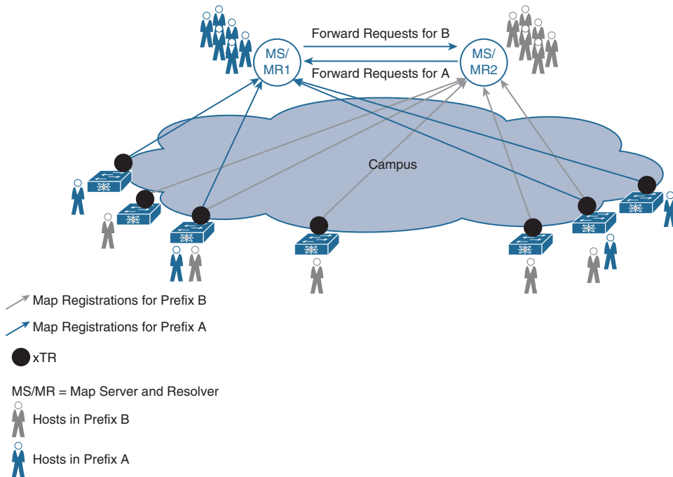
Figure 5-7 Topology-Independent Addressing with Control Plane Summarization
