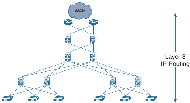
Figure 5-2 Routed Access Network Design
