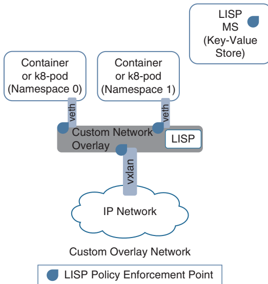
Figure 6-7 LISP-Based Container Overlay Custom Network
