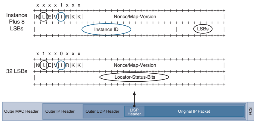
Figure 2-9 LISP Header Locator Status Bits
