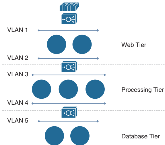
Figure 3-2 Service Stitching in Multitiered Applications
