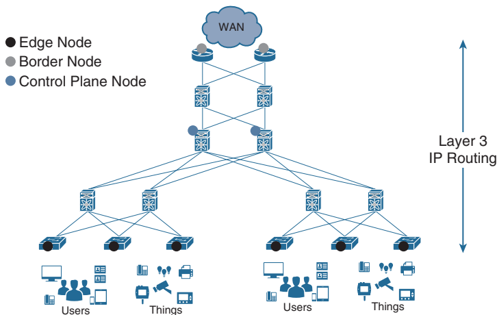
Figure 5-3 LISP Overlay Access Network
