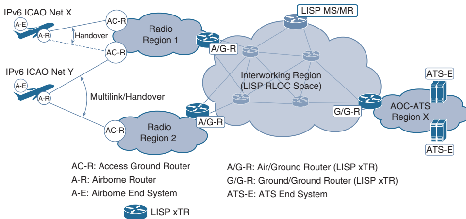
Figure 7-13 Aeronautical Telecommunications Network Using LISP
