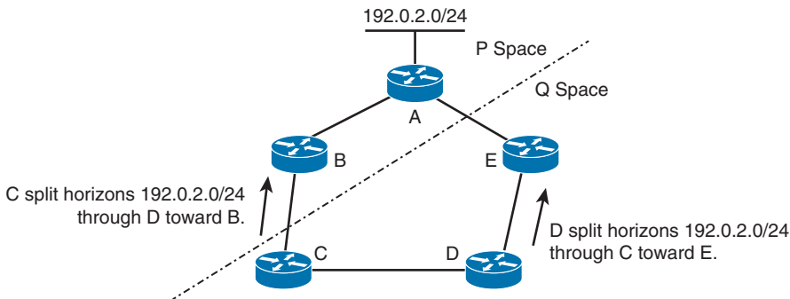
Figure 8-9 P Space and Q Space
