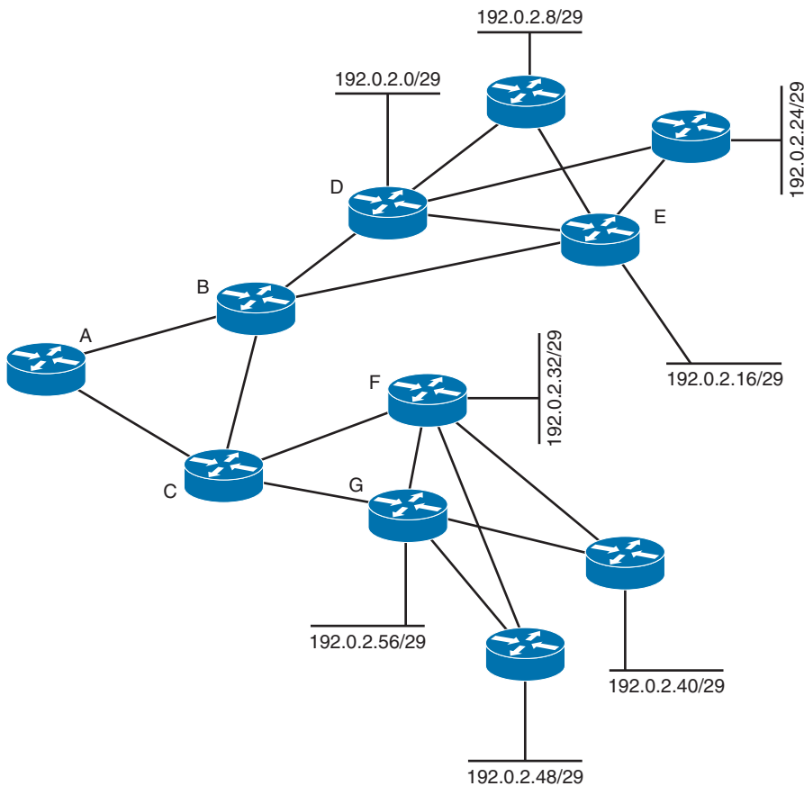
Figure 14-2 Illustration of Policy Dispersion
