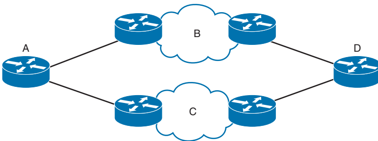
Figure 13-2 Example of BGP Policy
