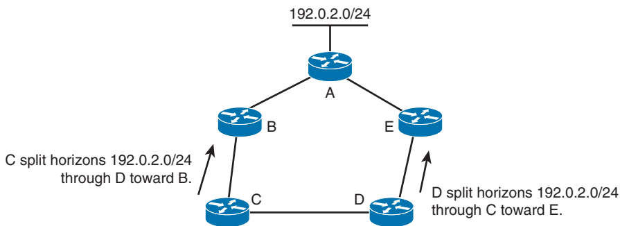
Figure 8-8 The Fast Reroute Problem
