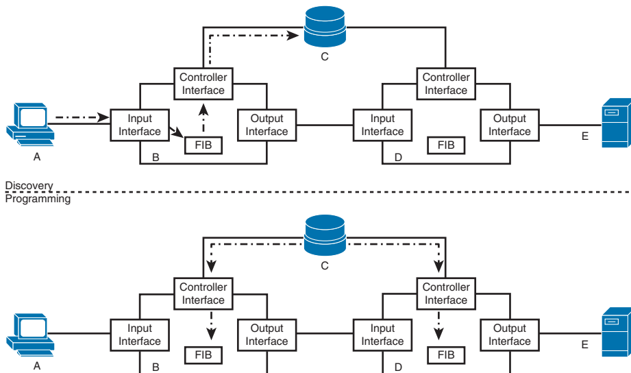
Figure 17-4 Reactive OpenFlow Operation
