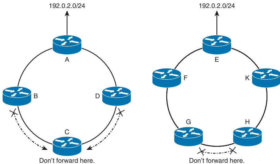
Figure 11-5 Loop Avoidance in Ring Topologies
