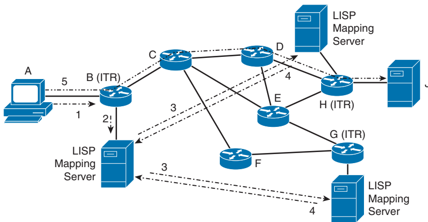
Figure 15-3 LISP Operation
