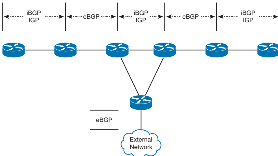
Figure 13-5 eBGP Edge-to-Edge
