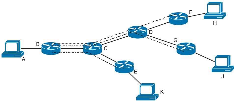
Figure 12-6 Multicast Replication in a Virtual Topology
