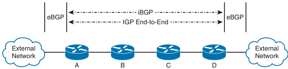
Figure 13-3 BGP Overlaid on IGP End-to-End
