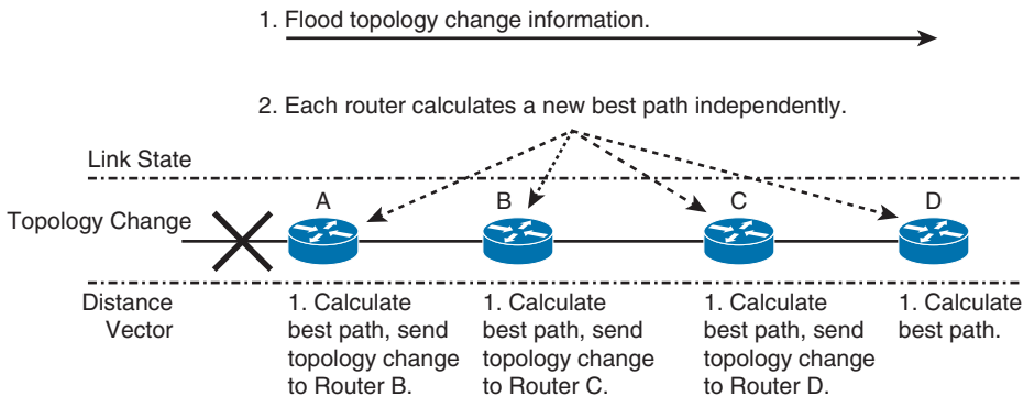
Figure 8-6 Distance Vector and Link State Convergence
