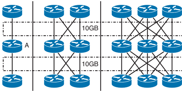
Figure 18-4 Spine and Leaf
