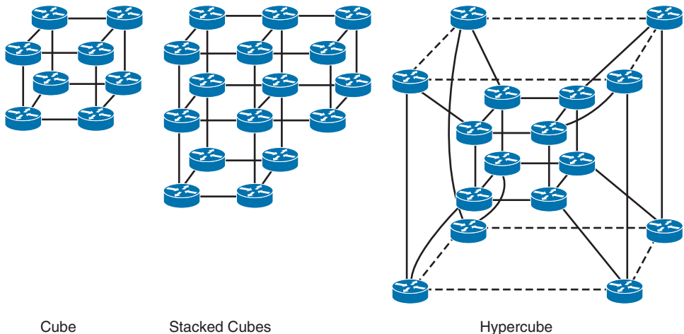
Figure 11-13 Cube Topologies
