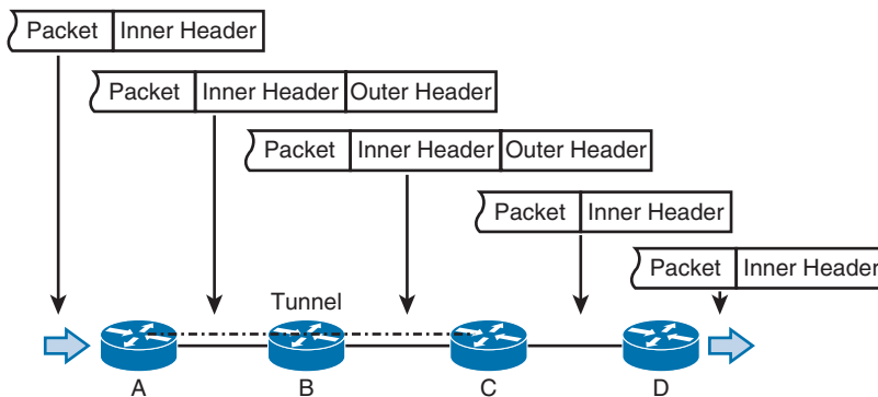
Figure 12-3 Tunneling or Not?
