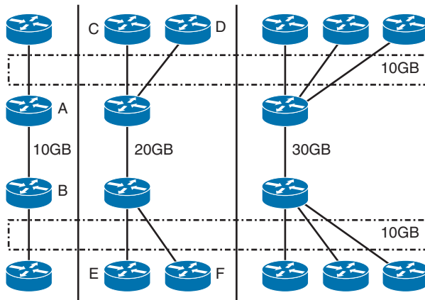
Figure 18-1 Traditional Aggregation Topology
