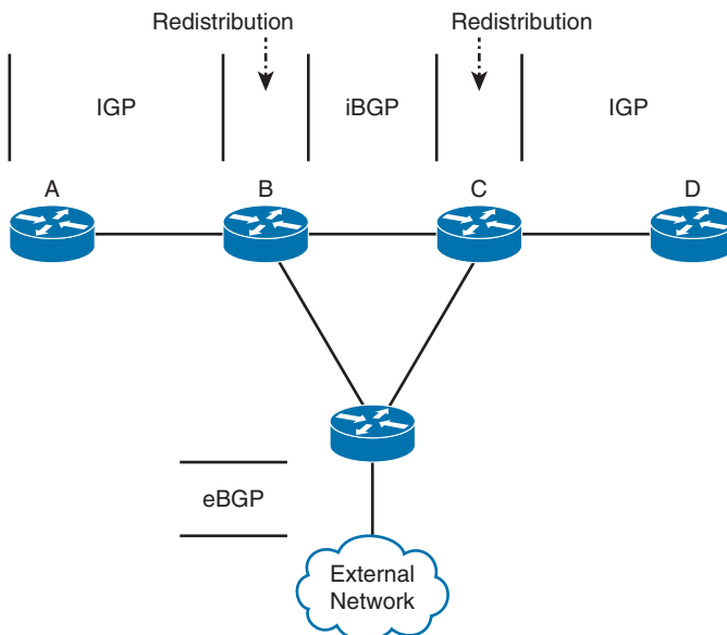
Figure 13-4 iBGP Core Deployment
