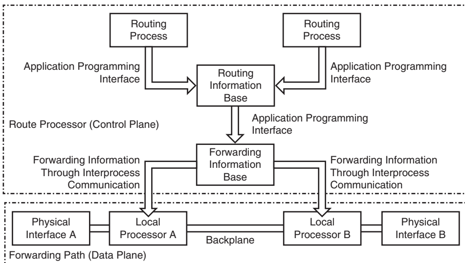
Figure 17-2 Model of Router Operation
