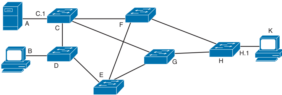
Figure 5-2 Example Network for TRILL Operation
