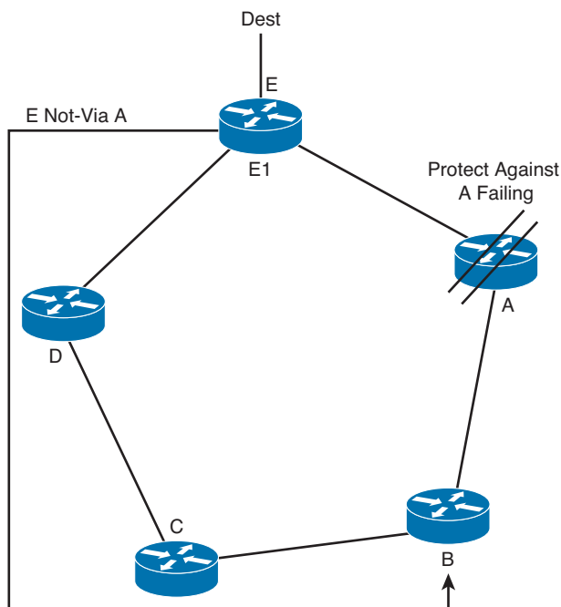
Figure 8-11 Not-Via Operation
