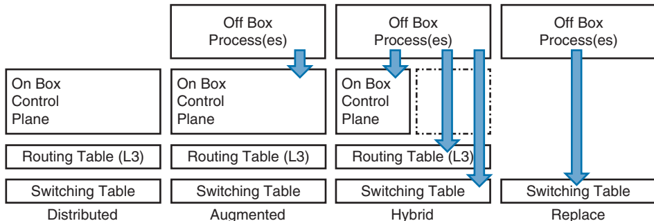
Figure 17-1 Software-Defined Networking Frameworks
