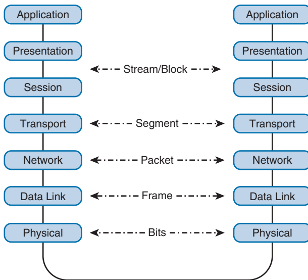
Figure 4-1 Seven-Layer Model
