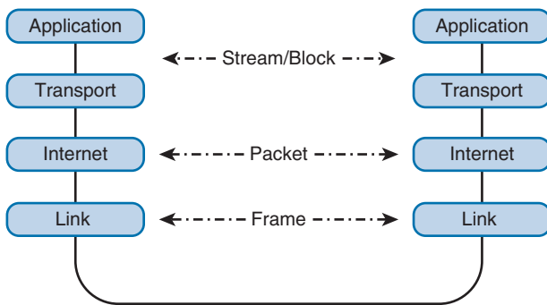
Figure 4-2 Four-Layer Model
