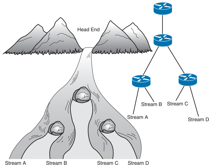
Figure 4-8 Waterfall Model
