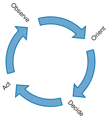
Figure 9-1 OODA Loop
