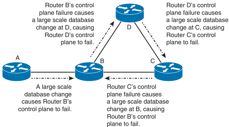
Figure 6-1 Positive Feedback Loop
