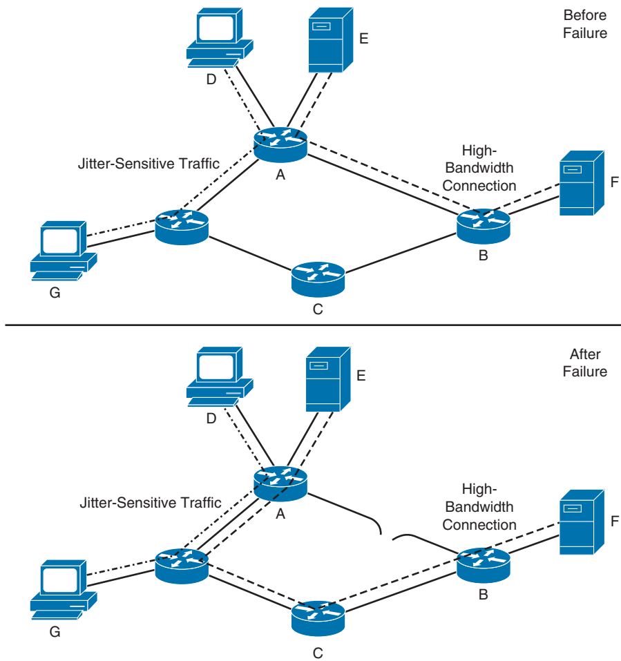
Figure 11-3 Traffic Engineering in a Ring Network
