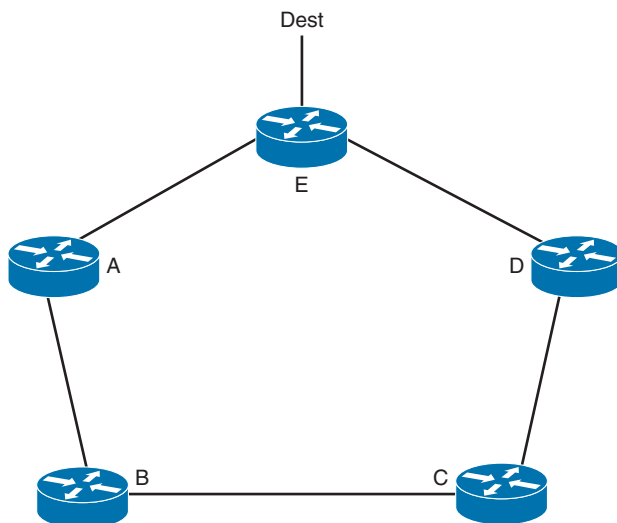
Figure 8-10 Remote LFA Operation
