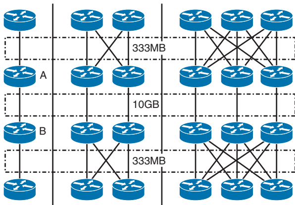
Figure 18-3 Next Step to a Fabric
