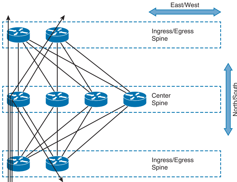
Figure 11-8 Traffic Flow in a Clos Fabric
