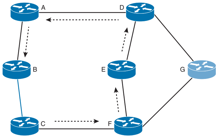
Figure 8-13 The First Tree Built Through MRT
