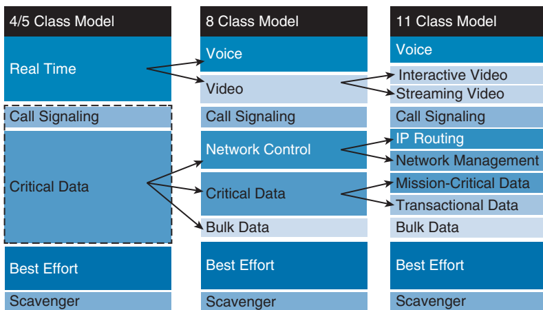
Figure 14-3 Queue Designs Compared
