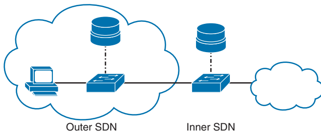
Figure 17-5 Hierarchical Replacement Model SDNs
