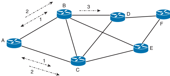
Figure 15-5 OSPF Overlapping Relay Operation
