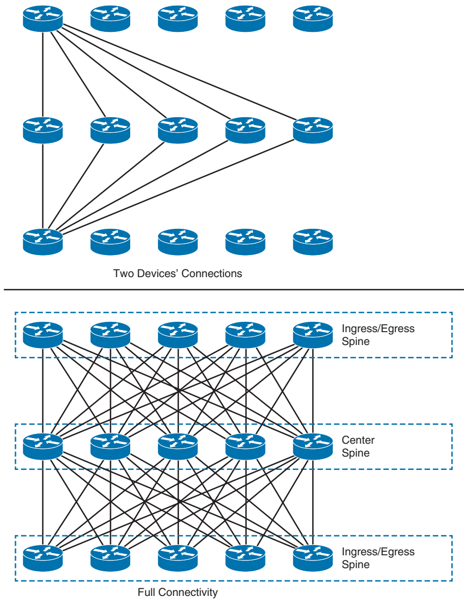
Figure 11-7 Clos Fabric
