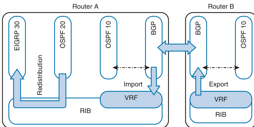
Figure 4-7 Redistribution and Import/Export
