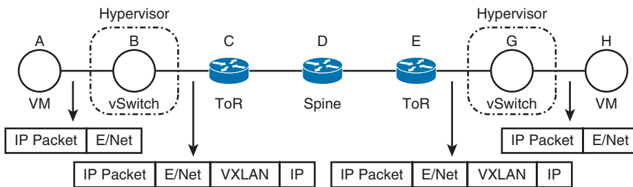
Figure 12-9 VXLAN Traffic Flow
