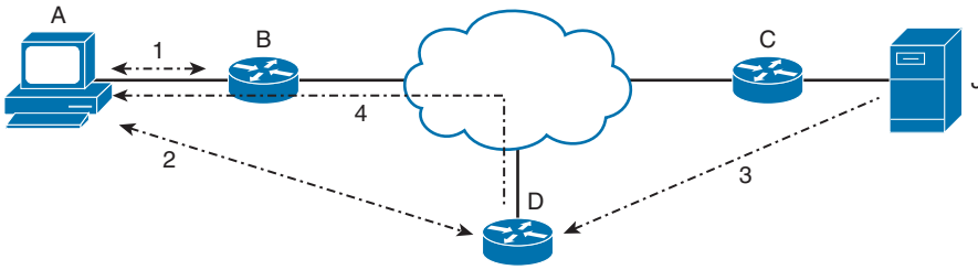
Figure 15-4 Mobile IP Operation
