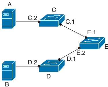
Figure 17-6 Moving a Flow in a Data Center
