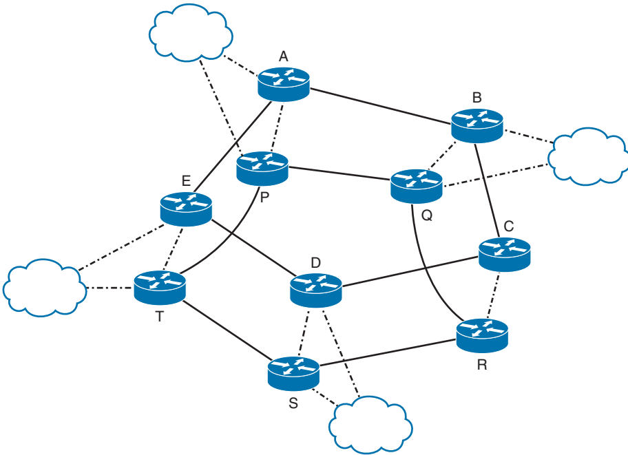
Figure 11-12 Diverse Data Plane Topology
