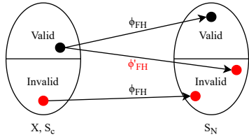
Figure 3: Mapping of valid and invalid input tuples to a valid or invalid next state.
