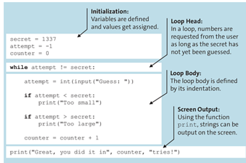
Figure 4.3 Guessing Numbers: A Simple Example
