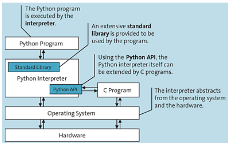
Figure 2.1 Overview of the Basic Concepts of Python
