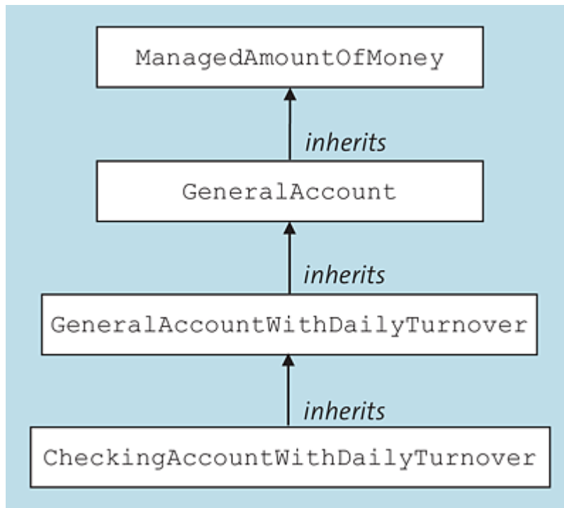
Figure 19.2 Class Hierarchy of the Account Example
