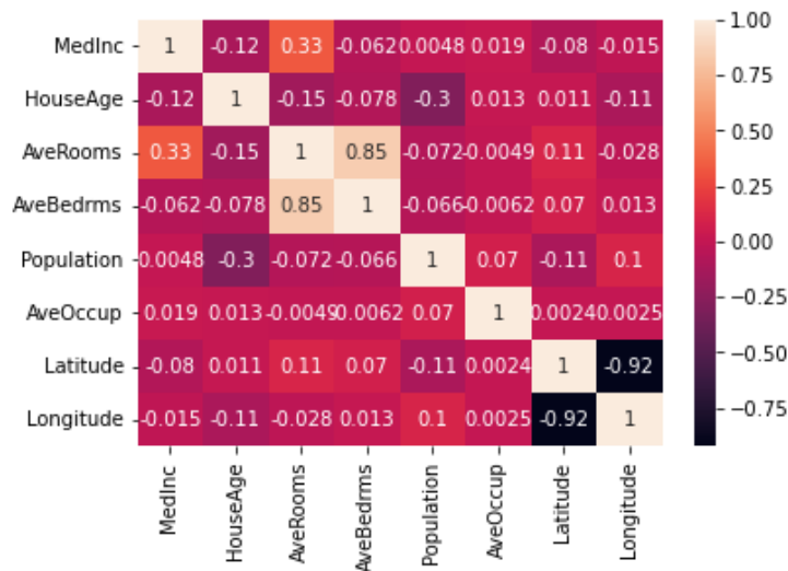
Figure 7.14 – The Correlation Coefficient technique shows some interesting relationships between variables
