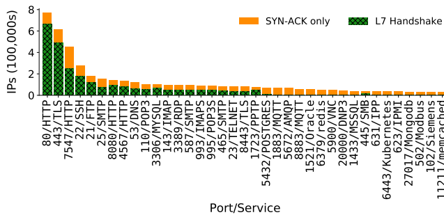
Figure 1: L4 vs. L7 Responsiveness —A significant fraction of hosts that respond with a SYN-ACK packet never complete the expected application-layer handshake. The difference varies dramatically across ports by both percent difference (14–96%) and raw count (21,050–200,902).
