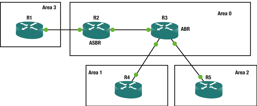
Figure 15-2. OSPF diagram
