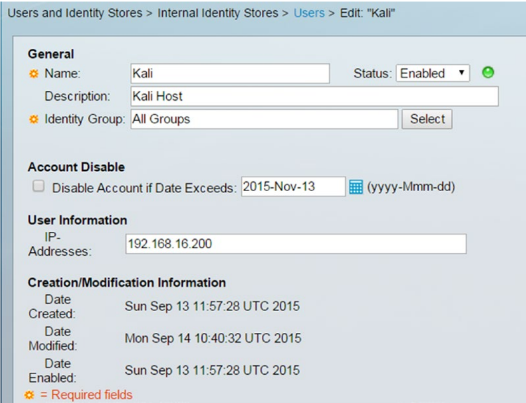
Figure 16-32. Local store user settings
