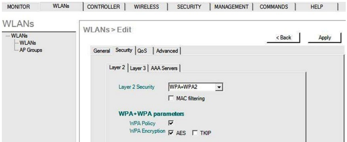
Figure 20-5. Wireless controller GUI 4
