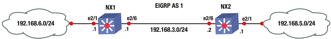
Figure 19-2. EIGRP diagram
