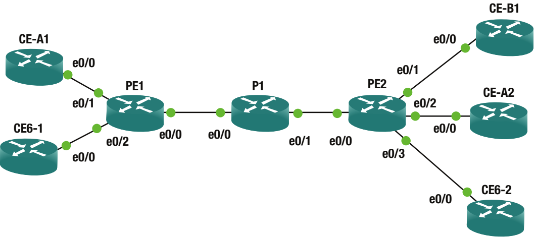
Figure 23-3. Exercise topology
