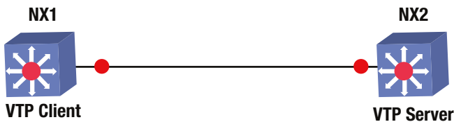
Figure 19-1. VTP diagram
