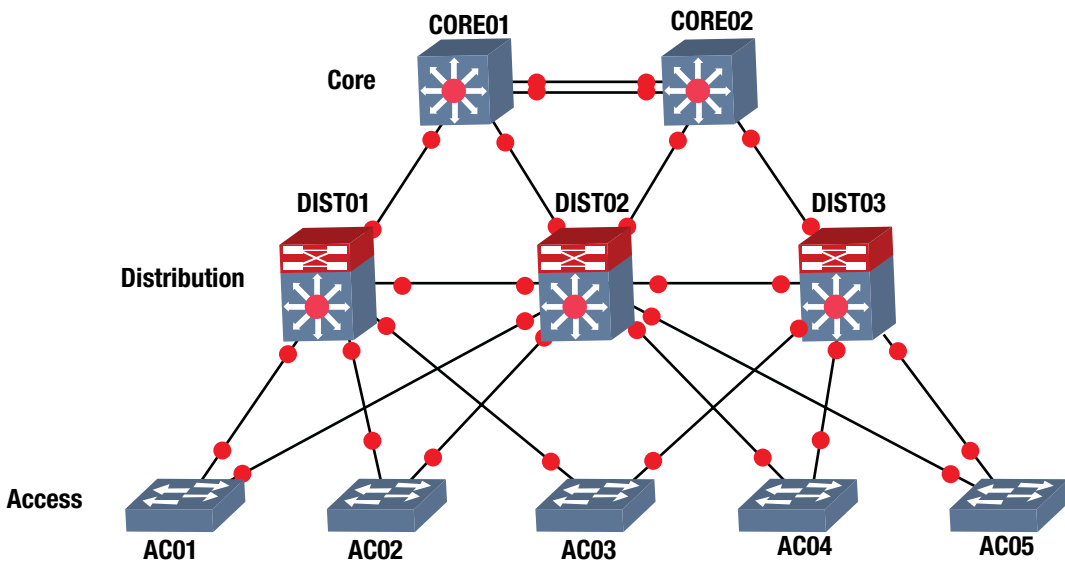
Figure 1-11. Hierarchical model
