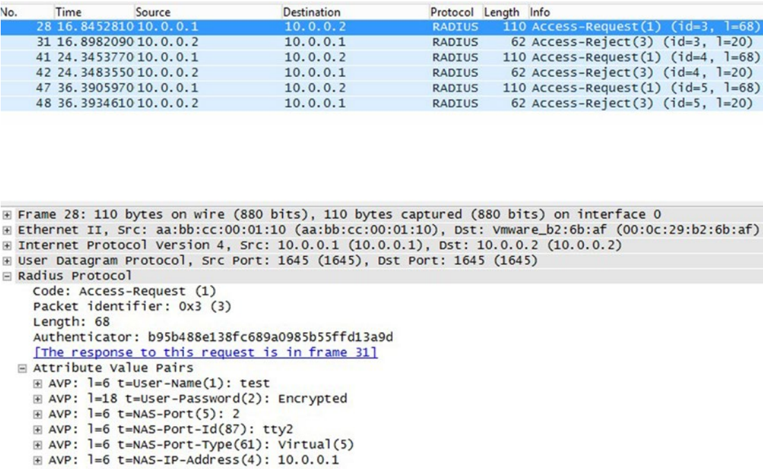
Figure 10-3. RADIUS authentication
