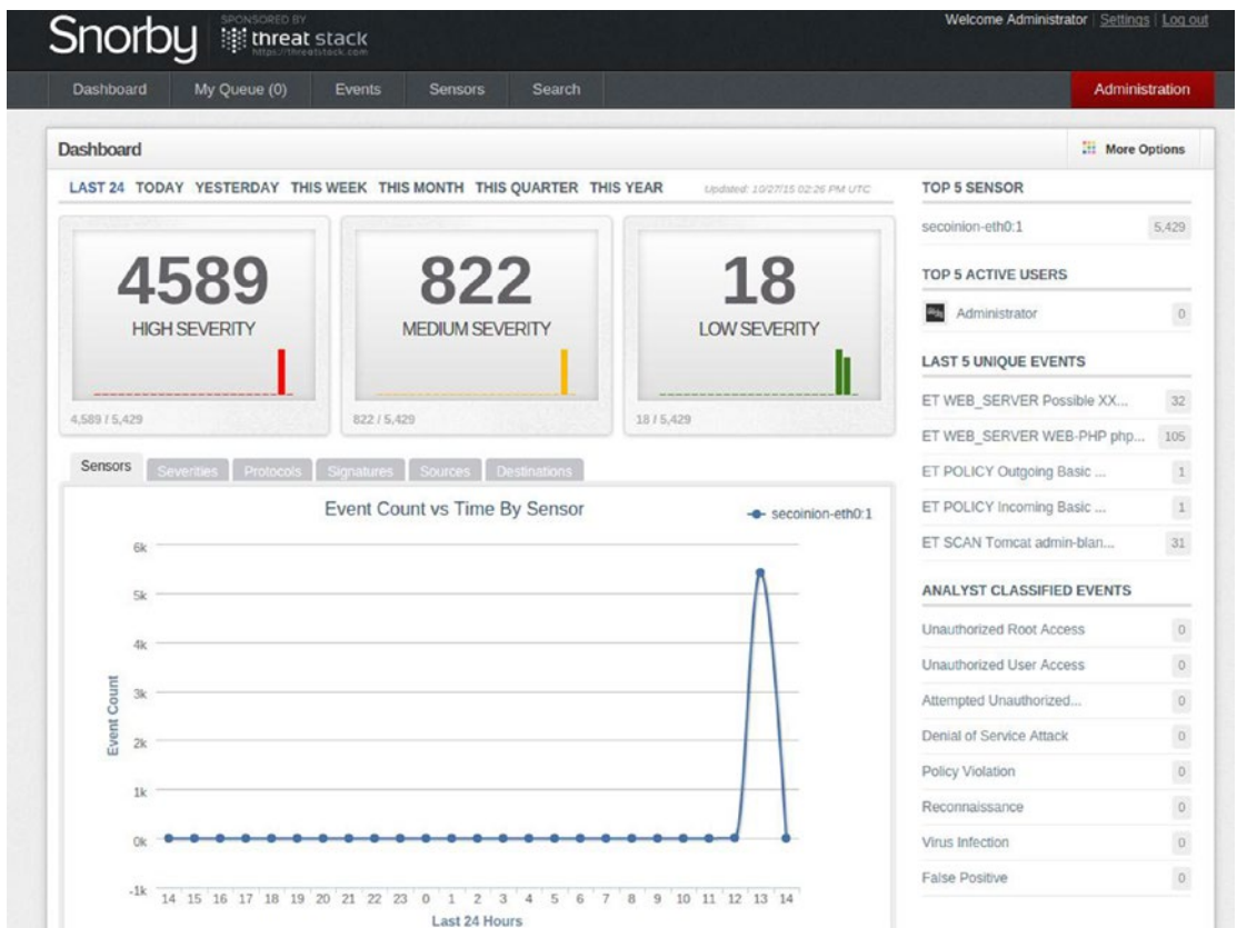
Figure 21-17. Snorby view of baseline event detection from Snort caused by the Sparta scan
