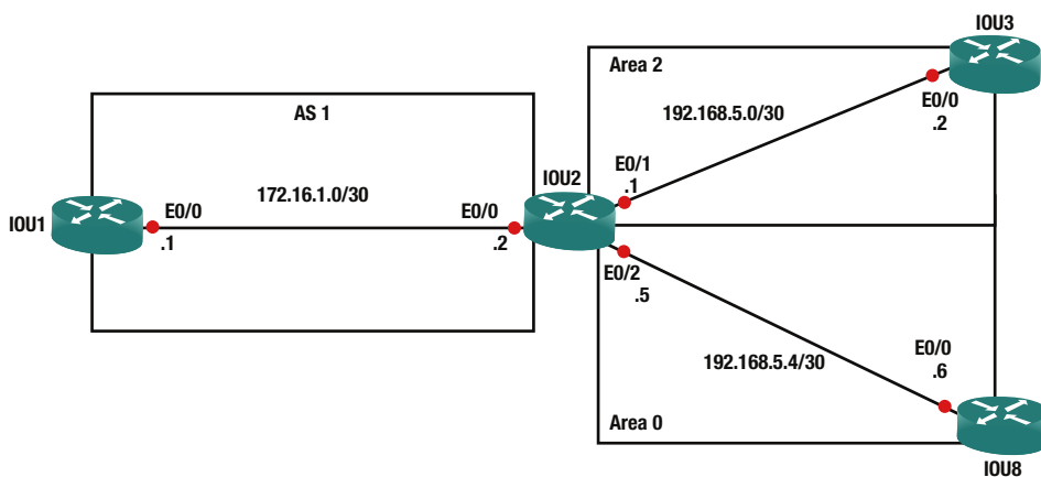
Figure 15-9. Exercise 1 diagram
