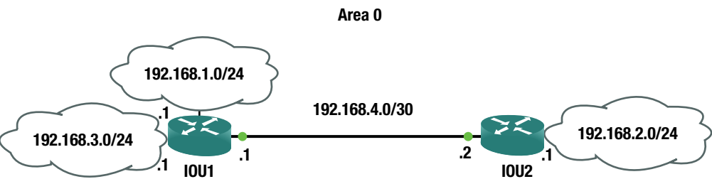
Figure 8-9. OSPF example diagram
