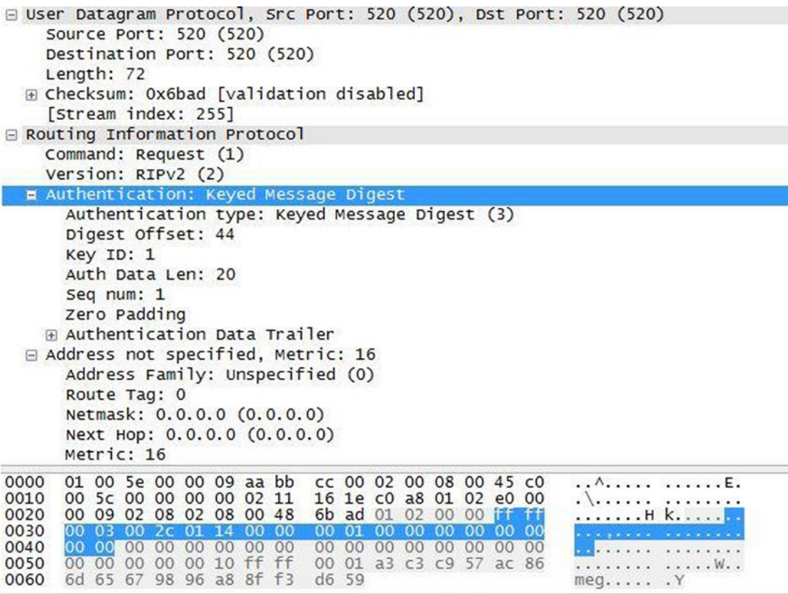
Figure 6-9. RIP authentication MD5
