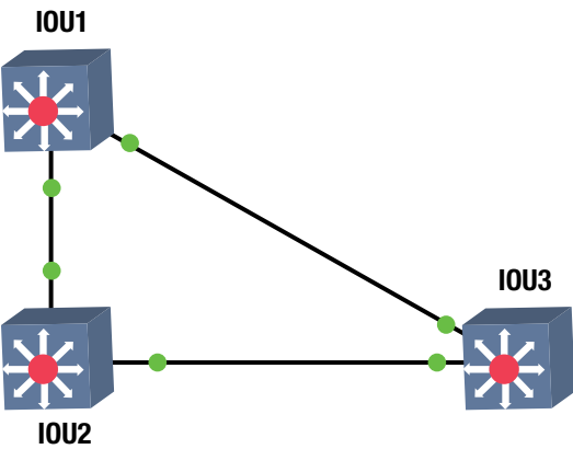
Figure 8-5. STP example
