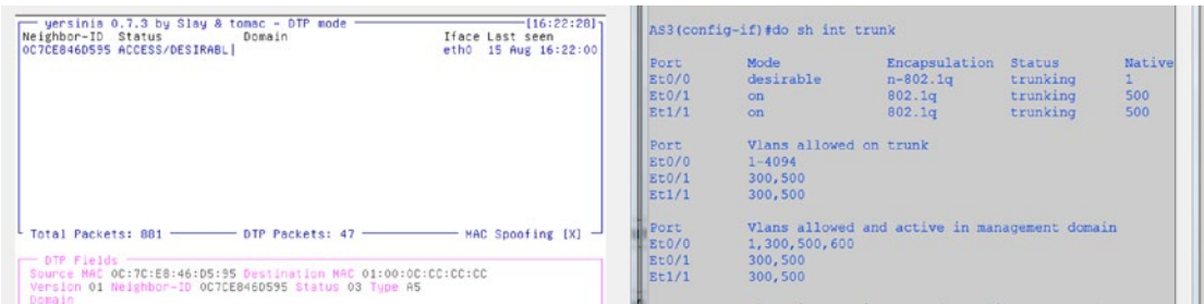
Figure 16-14. Attacker trunks on port Eth0/0 setup as “dynamic desirable”
