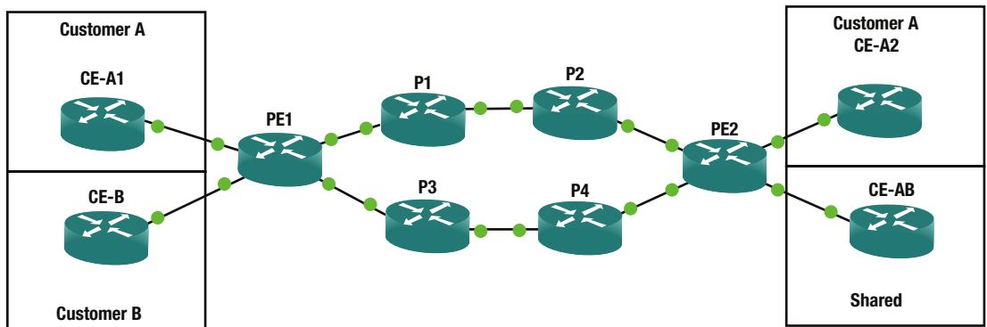
Figure 23-2. MPLS VPN
