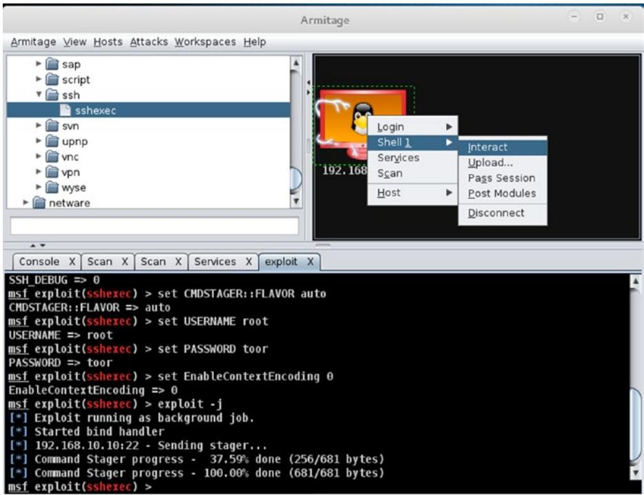
Figure 22-13. Armitage host interaction
