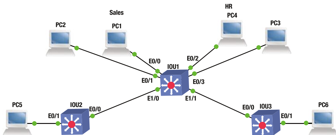
Figure 7-3. 802.1Q VLAN diagram
