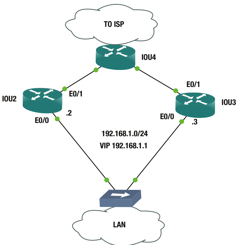
Figure 13-5. VRRP example
