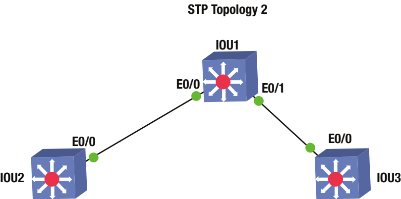
Figure 7-7. Spanning-Tree diagram
