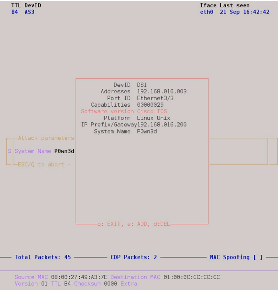
Figure 16-51. Crafting CDP PDUs from Yersinia
