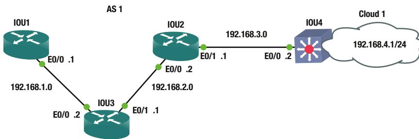
Figure 6-10. EIGRP routing diagram
