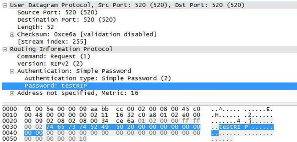
Figure 6-8. RIP authentication clear text PCAP
