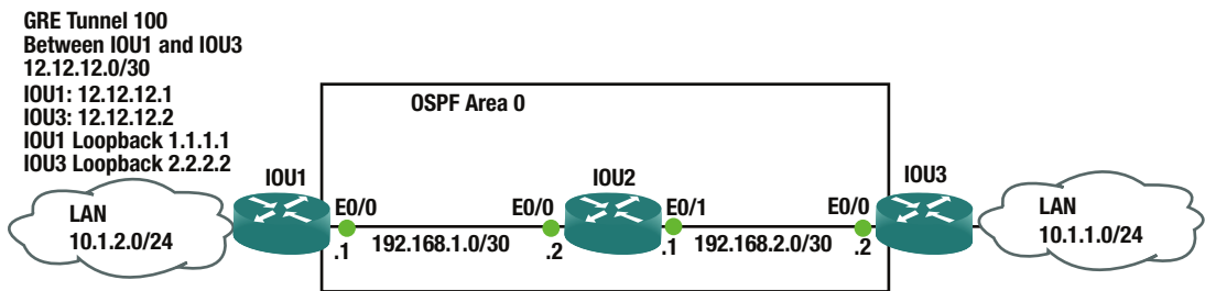
Figure 17-9. GRE example diagram
