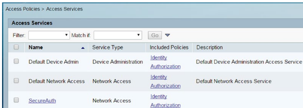
Figure 16-39. Defining access services
