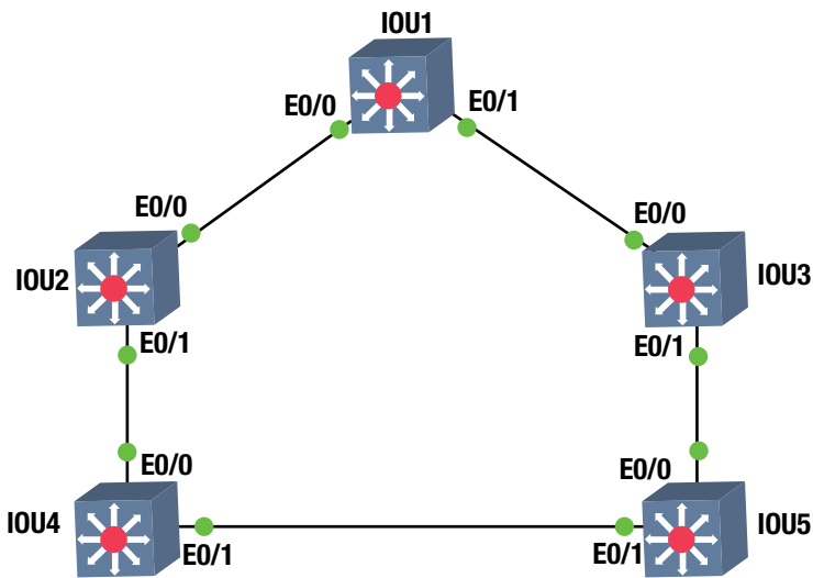
Figure 5-8. STP answer diagram
