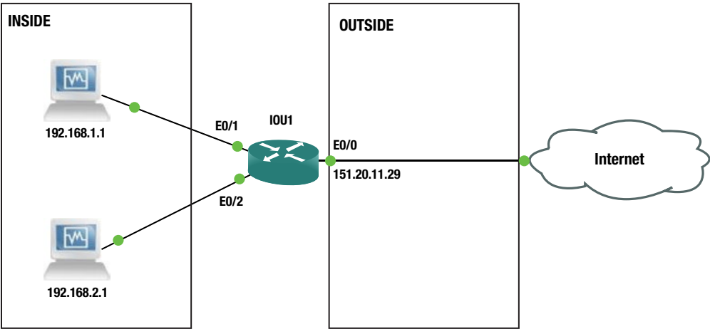
Figure 9-4. PAT example
