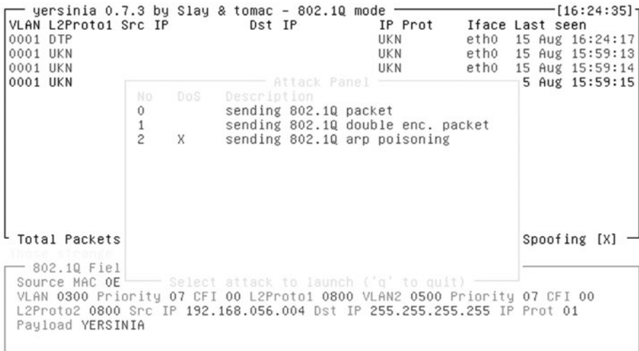
Figure 16-15. Attack options for 802.1Q
