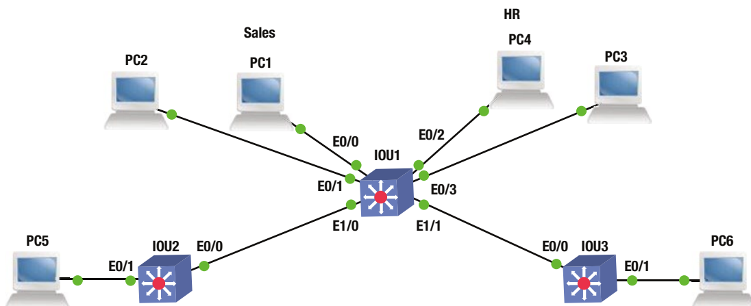
Figure 7-5. VTP architecture example
