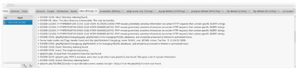
Figure 21-14. Sparta port 80 scan vulnerabilities listing
