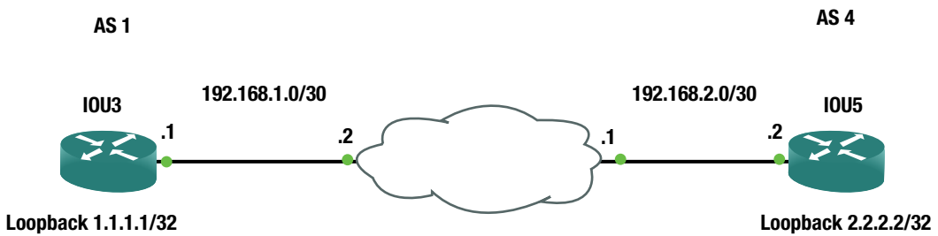
Figure 8-13. BGP example
