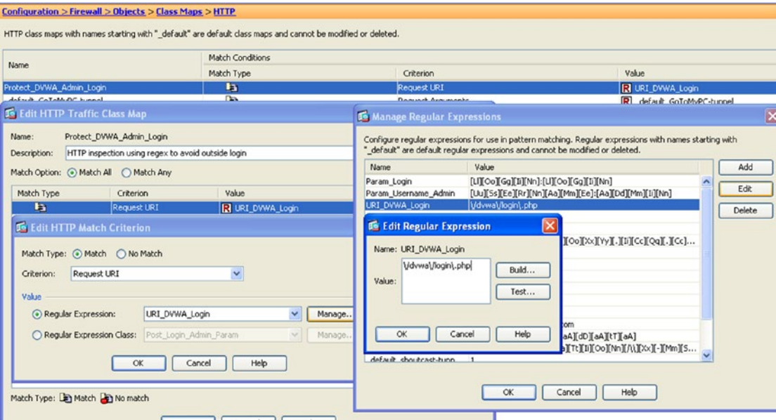
Figure 21-34. Constructing the first element of the HTTP inspection policy to look for the /dvwa/login.php URL path within the client's request
