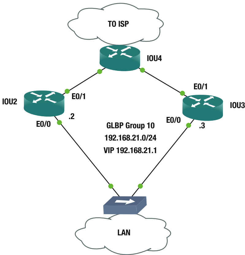
Figure 13-6. GLBP example
