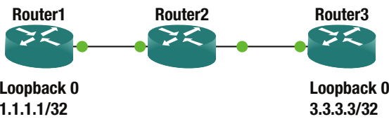
Figure 18-7. IP SLA example network
