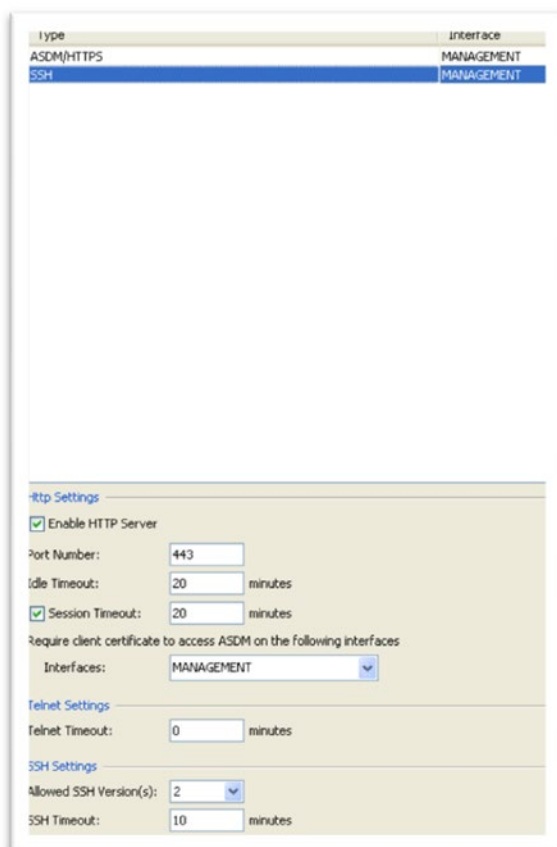
Figure 21-2. ASA management access parameters
