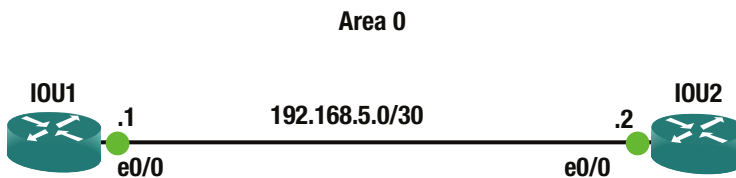
Figure 17-6. OSPF example diagram
