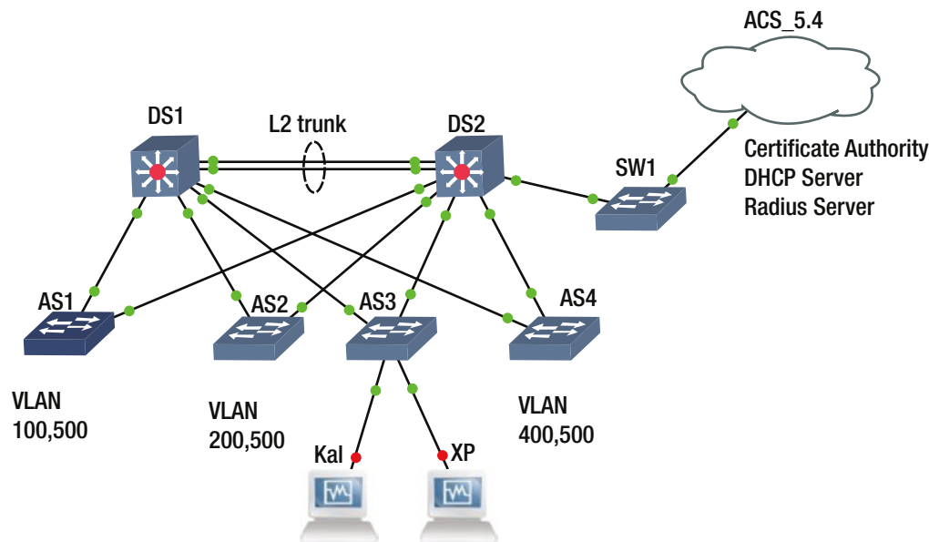
Figure 16-18. Diagram of the MAC flood scenario
