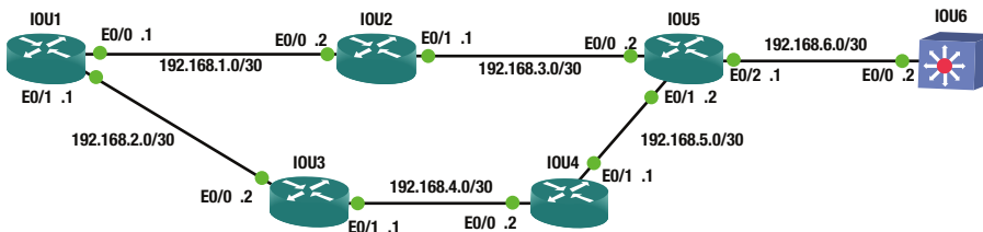
Figure 6-21. RIP routing answer diagram
