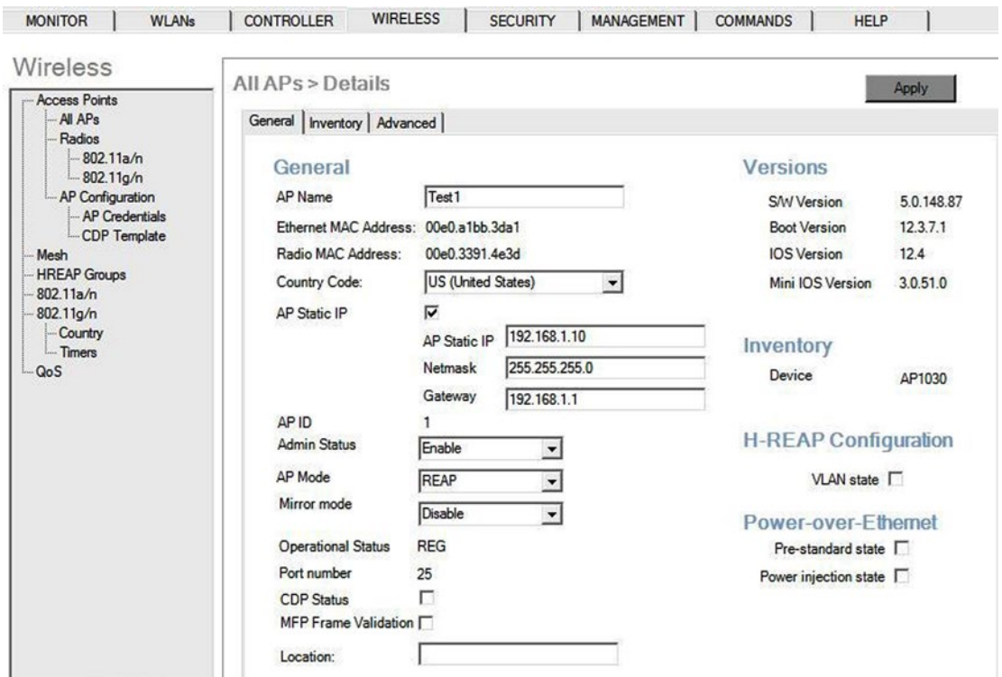
Figure 20-8. Wireless controller GUI 7
