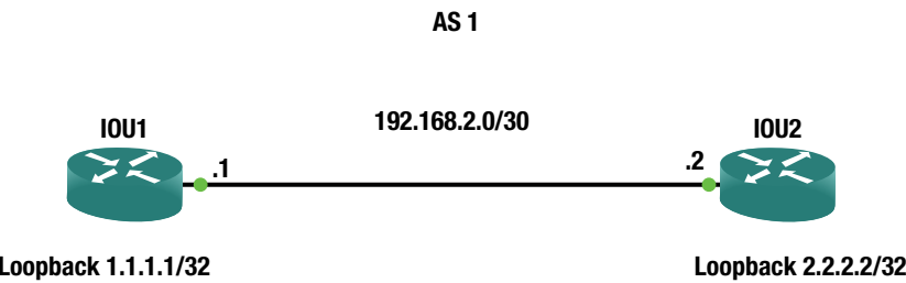
Figure 8-12. BGP example diagram
