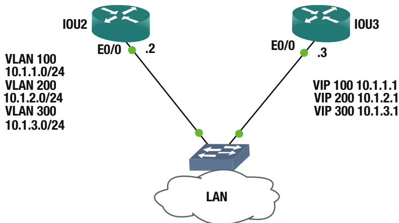
Figure 14-1. HSRP diagram
