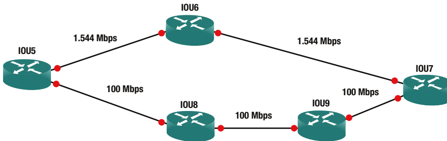
Figure 6-5. Link-State diagram
