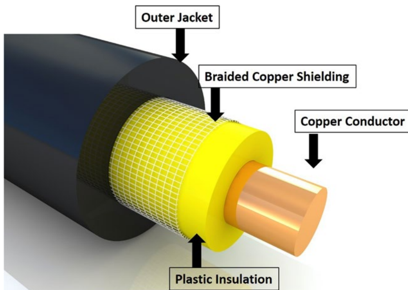
Figure 2-4. Coaxial cable (Photo copyright Solomonkein | Dreamstime.com .)
