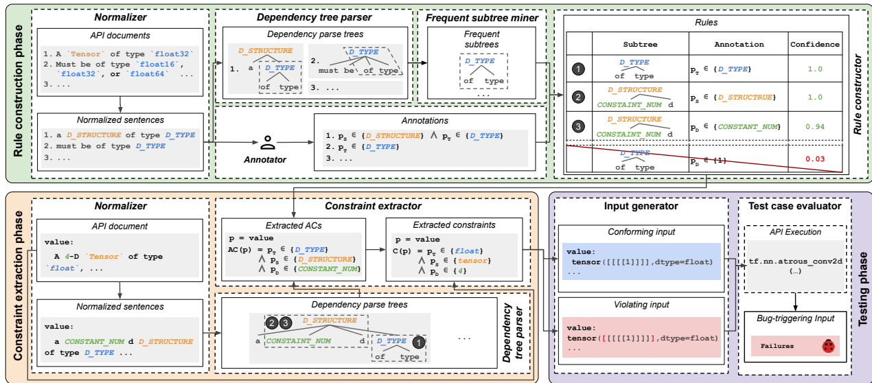
Figure 2: Overview of DocTer. p_T , p_S , and p_D are the abstract constraints representing the data type , data structure , and number of dimensions of parameter p , respectively. Detailed constraint formats are explained in Section 2.2.
