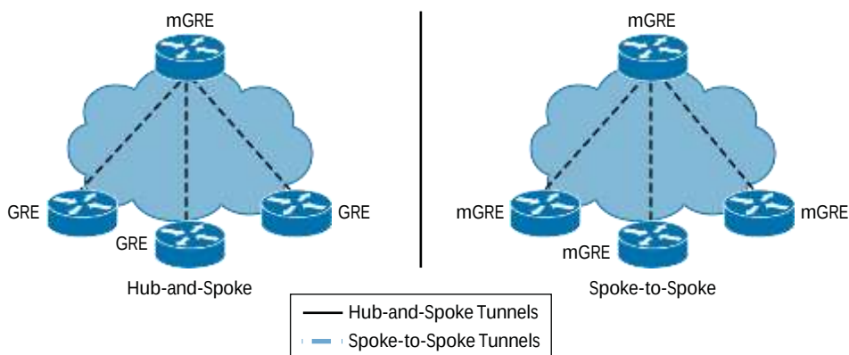
Figure 1-20 GRE Options
