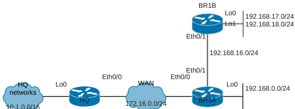
Figure 2-14 EIGRP Topology for Configuring Stub Routers
