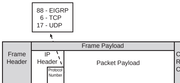
Figure 2-1 EIGRP Encapsulation
