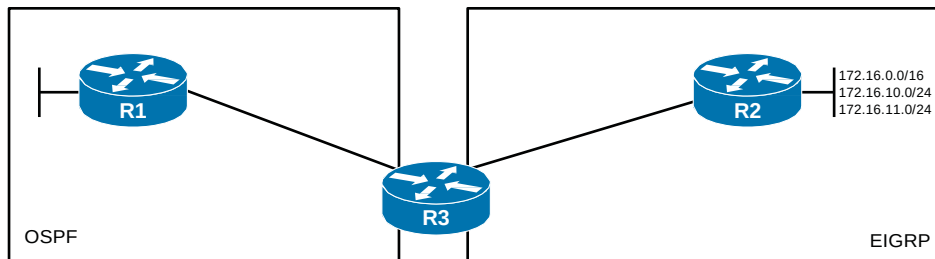
Figure 4-16 Network Used in Prefix List Option Testing
