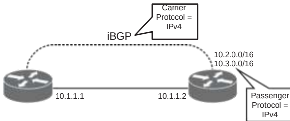
Figure 7-23 BGP with IPv4 as Both the Carrier and Passenger Protocol
