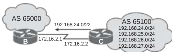
Figure C-2 BGP Network for Summarization Examples
