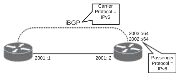
Figure 7-25 BGP with IPv6 as Both the Carrier and Passenger Protocol
