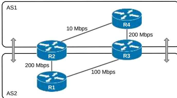
Figure 4-11 Two-Way Multipoint Redistribution Issue
