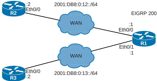
Figure 8-13 EIGRP for IPv6 Routing Authentication Reference Topology
