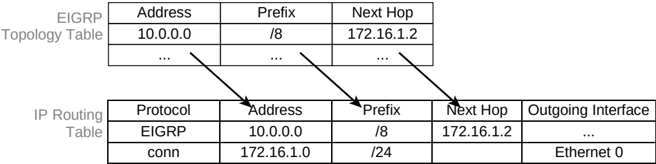
Figure 5-4 EIGRP Entry Added to the Routing Table
