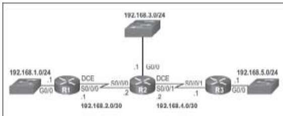
Figure 1-25 RIPv2 Topology
