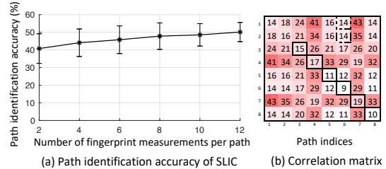
Figure 7: Accuracy of path-identification attack. The identification accuracy increases as the number of labeled fingerprints increases. The errorbar denotes the standard deviation.
