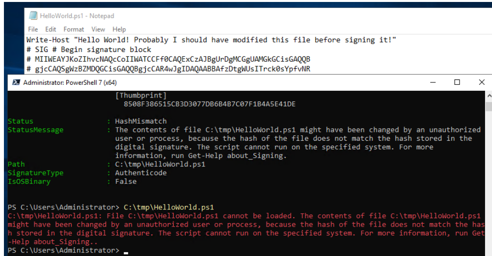
Figure 11.10 – HashMismatch after changing the signed file's content
