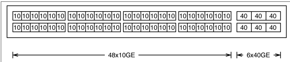
Figure 1-24. The front panel of the Juniper QFX5100-48T
