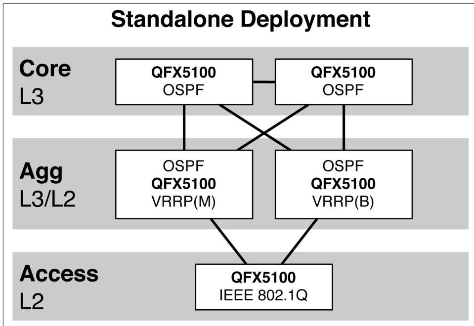
Figure 4-2. Standalone deployment
