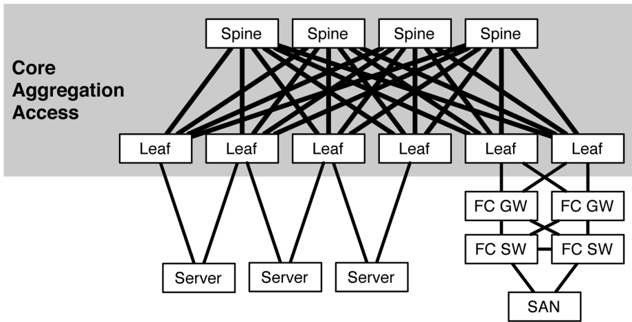
Figure 4-8. FCoE transit with VCF
