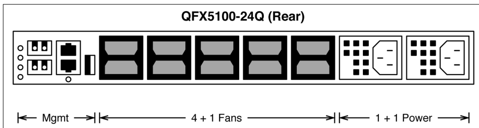
Figure 1-15. View of the rear of the Juniper QFX5100-24Q
