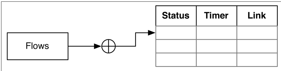
Figure 5-3. Flowlet hashing
