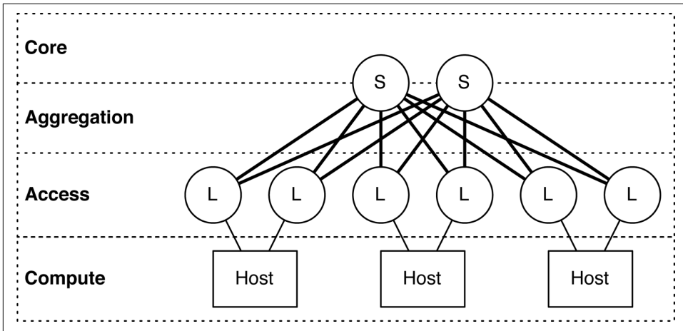
Figure 1-19. Spine-and-leaf topology, with the Juniper QFX5100-48S as a leaf
