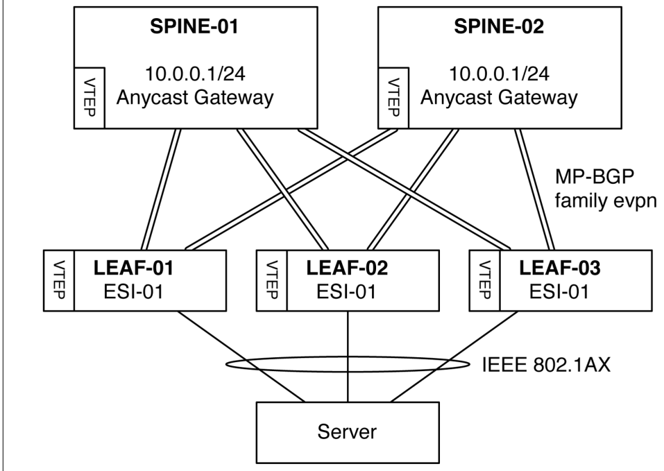
Figure 8-9. Illustration of EVPN Anycast gateway and ESI overview
