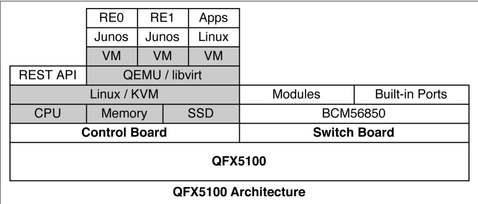
Figure 2-1. QFX5100 architecture
