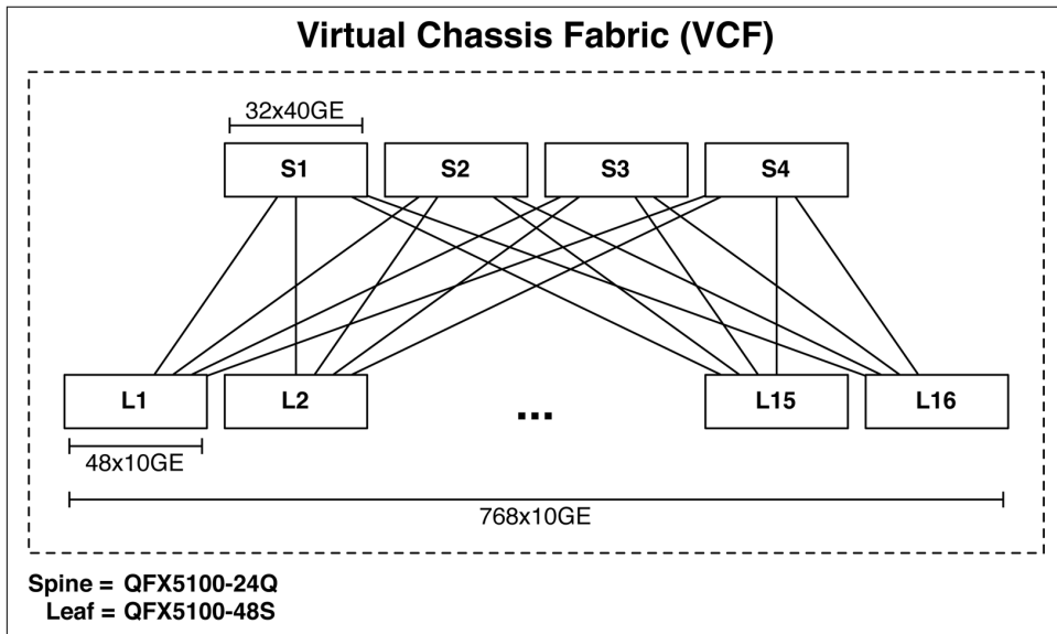
Figure 1-32. 768 10GbE VCF
