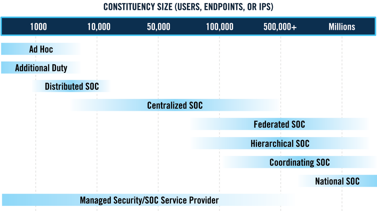
Figure 6. SOC Organizational Model Versus Constituency Size
