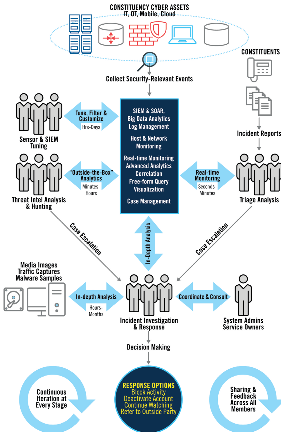
Figure 3. Basic SOC Workflow
