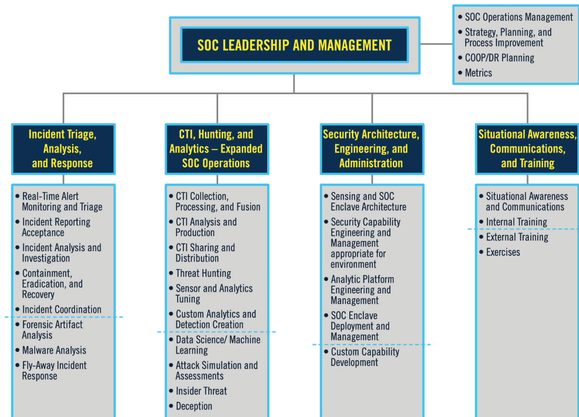
Figure 7. Notional Centralized SOC
