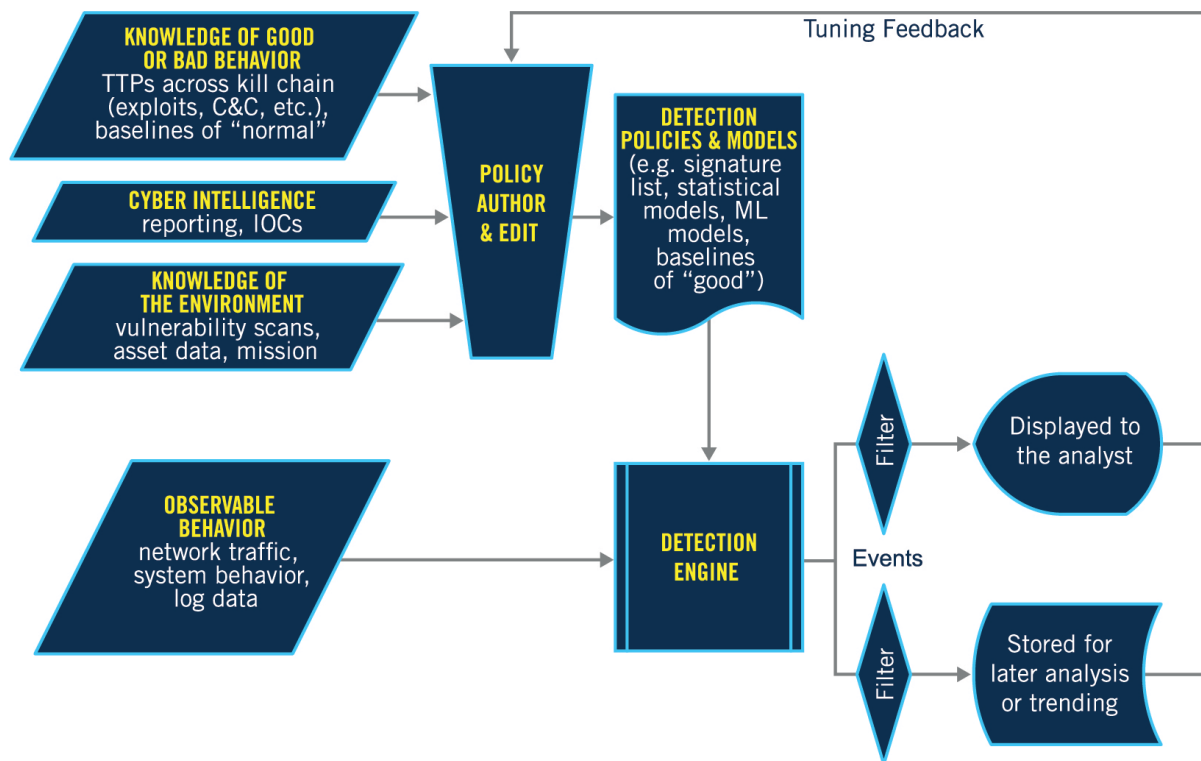
Figure 20. SOC Data and Detection in the Abstract
