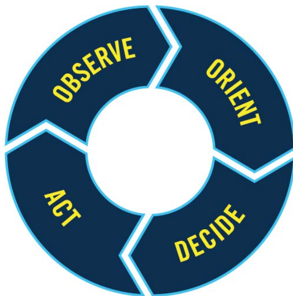
Figure 4. OODA Loop [16], [17]
