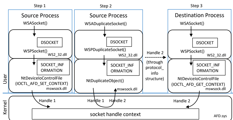
Figure 4: Winsock Duplication
