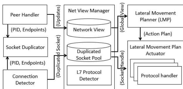
Figure 2: ShadowMove Architecture
