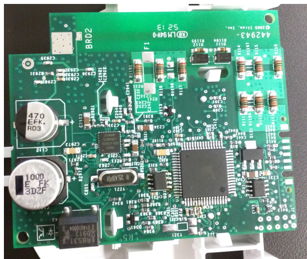
Fig. 7. Smart Meter CL200 Daughterboard
