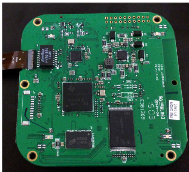
Fig. 2. SmartCare Hardware Platform
