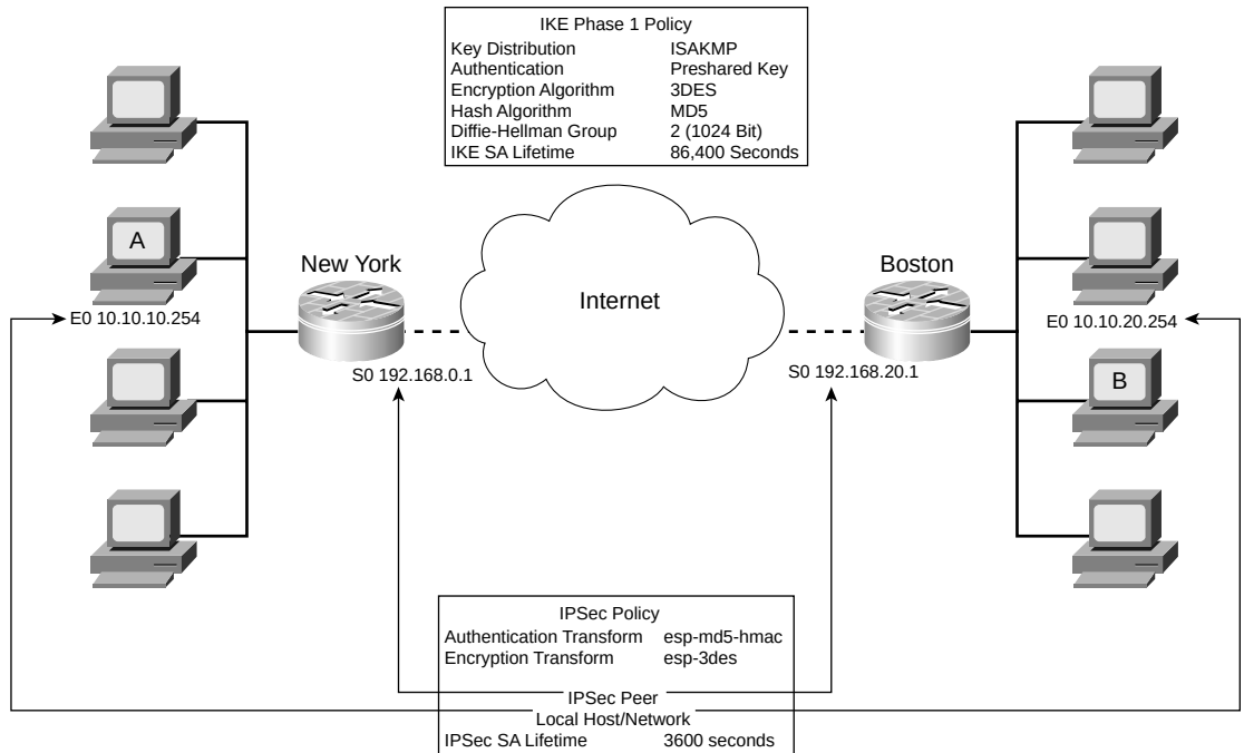
Figure 17-8 IPSec Configuration Settings
