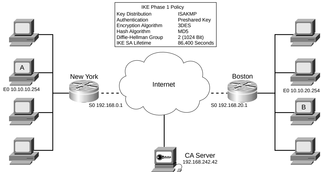
Figure 18-3 IKE Configuration Parameters
