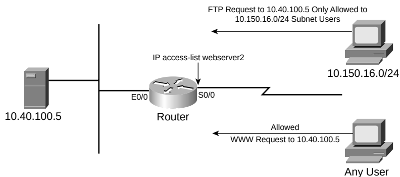
Figure 12-4 ACL webserver2 Being Applied to the Serial Interface of a Router
