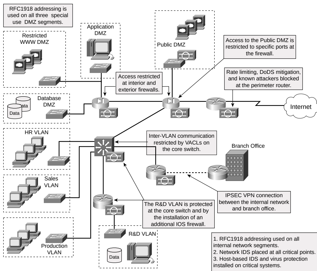
Figure 3-1 Network Segmentation
