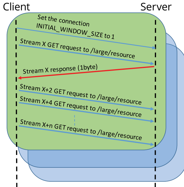
Figure 13: Nginx Slow GET Attack
