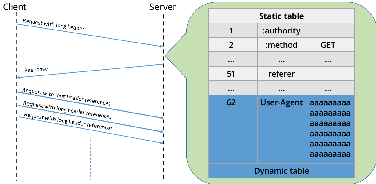
Figure 23: HPACK Bomb
