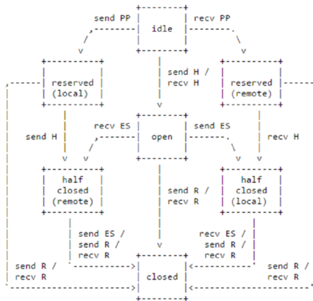
Figure 2: Stream states
