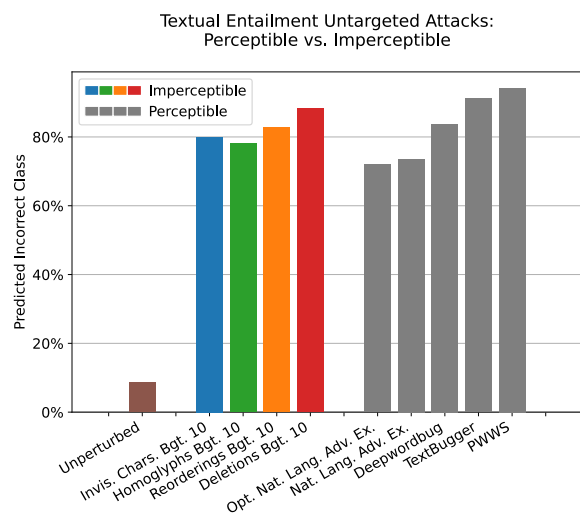
Fig. 12. Perceptible and imperceptible attack success rates against Facebook Fairseq RoBERTa MNLI.
