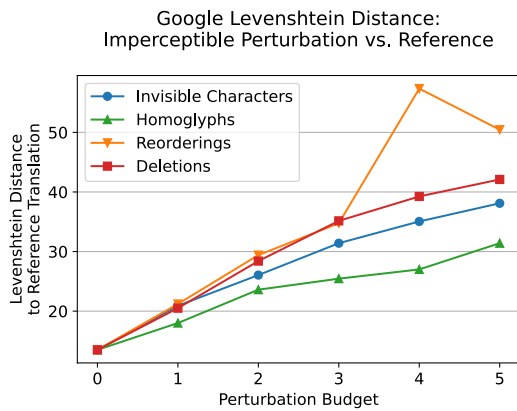
Fig. 18. Levenshtein distances between imperceptible perturbations and unperturbed WMT data on Google Translate’s EN-FR model
