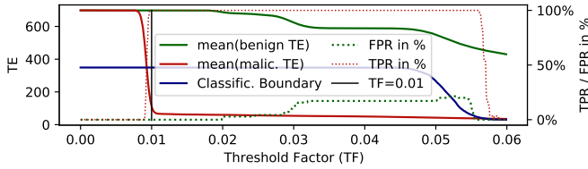
Fig. 8: Average number of benign Threshold Exceedings (mean(benign TF)), average number of malicious Threshold Exceedings (mean(malic. TE)), Classification boundary, FPR, and TPR for different Threshold Factors (TF).
