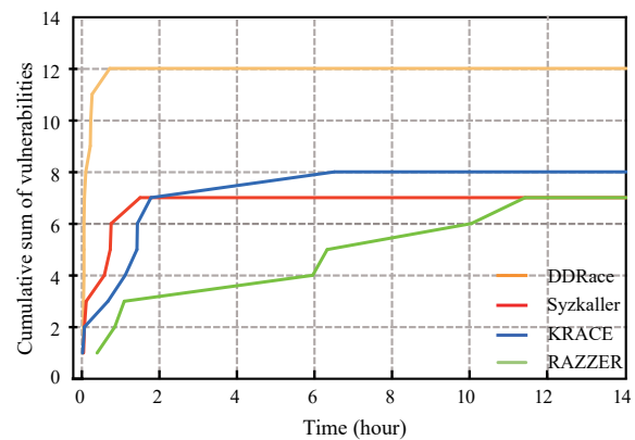
Figure 6: Comparison of vulnerability-finding time for 12 concurrency UAF vulnerabilities.
