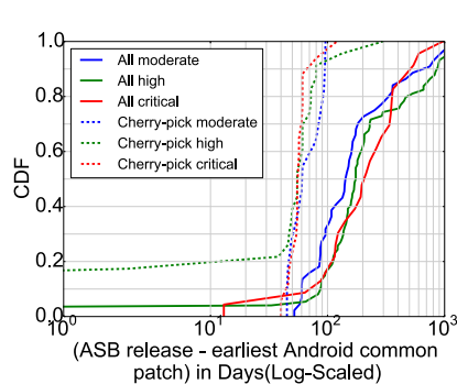
Figure 17: Notification delays of Linux CVEs (by severity)
