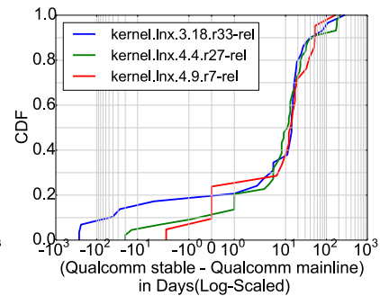
Figure 9: Qualcomm mainline to stable (Qualcomm CVEs)
