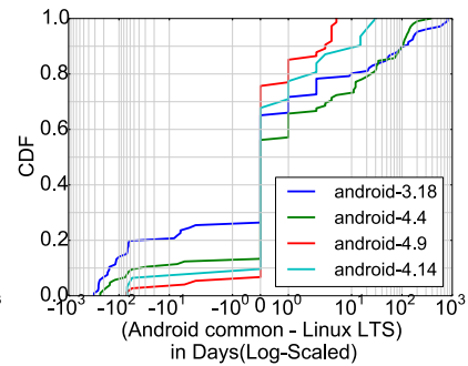
Figure 6: LTS to Android common (Linux CVEs)
