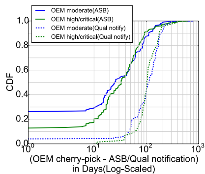
Figure 19: Post-notification delays of cherry-picked patches (by severity)
