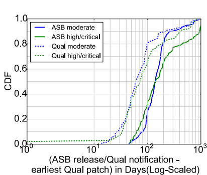
Figure 18: Notification delays of Qualcomm CVEs (by severity)
