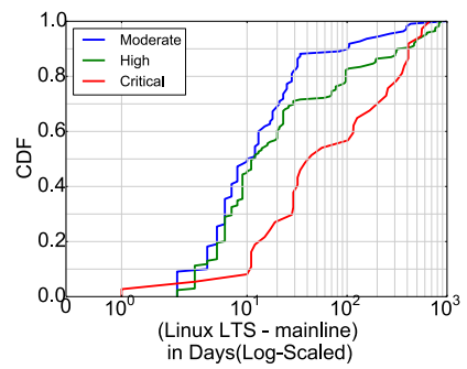
Figure 15: Patch delays from Linux mainline to LTS (by severity)
