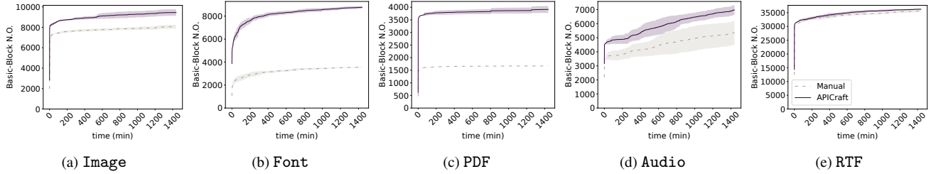
Figure 7: Basic block coverage per time for both APICRAFT generated and manually written fuzz drivers for the five attack surfaces
