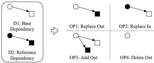
Figure 5: Possible mutation operations (OP1-4) for a given data dependency (D1), different \langle Func, In/Out \rangle are simplified to circles and rectangles with different colors.
