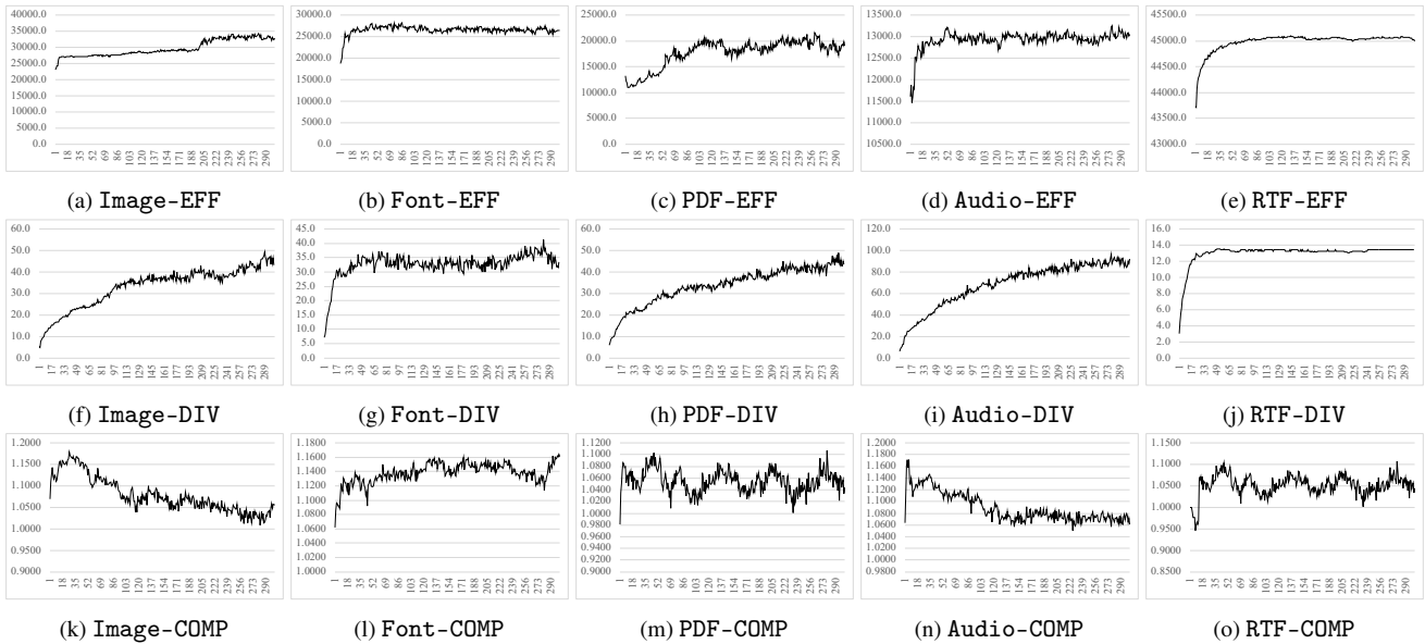
Figure 11: EFF/DIV/COMP objective scores per time during the dependency combination for the five attack surfaces. The x-axis is the round of the genetic algorithm, the y-axis is the value of the score.
