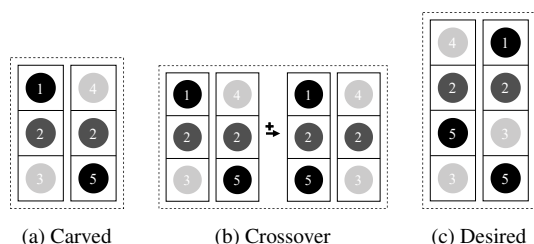
Figure 3: Potential fuzz driver suites (rectangles with dashed border) generated based on the consumer programs. Each circle represents a function in Fig. 2. Each chain of circles represents a fuzz driver (made up of function calls).
