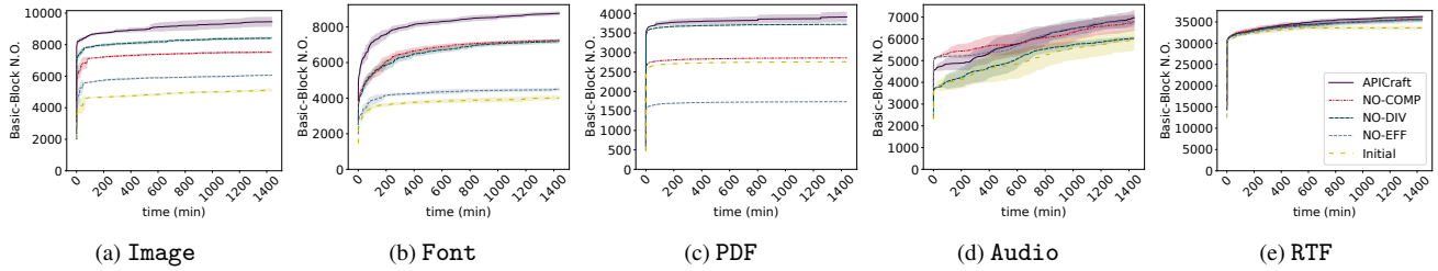
Figure 8: Basic block coverage per time for both APICRAFT generated with three objectives (APICRAFT), without COMP (NO-COMP), without DIV (NO-DIV), without EFF (NO-EFF), and initial (Initial) fuzz drivers for the five attack surfaces
