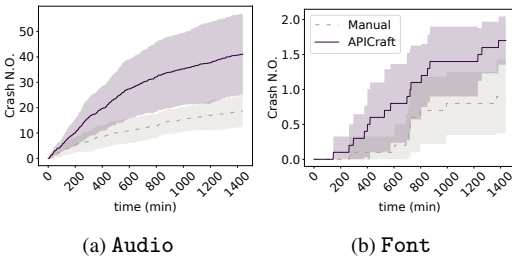
Figure 9: Unique crash per time for both APICRAFT generated and manually written fuzz drivers for Audio and Font attack surfaces (The rest three attack surfaces have found no crash in 24 hours)
