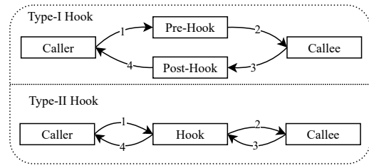
Figure 6: Two types of binary function hook mechanism.
