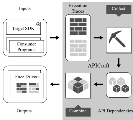
Figure 1: The overview of APICRAFT.
