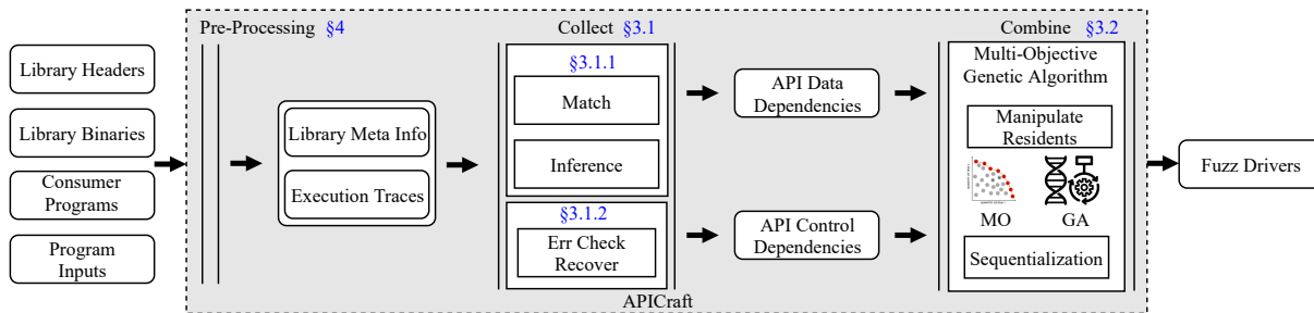
Figure 4: The workflow of APICRAFT.
