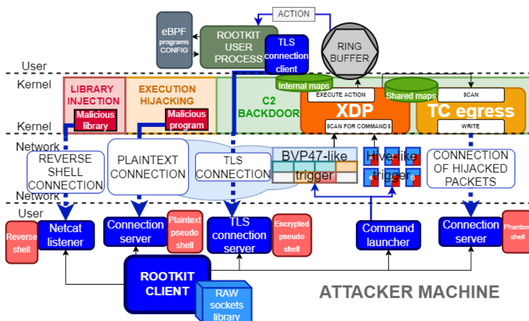
Fig. 4.26. Command and Control infrastructure of the rootkit.
