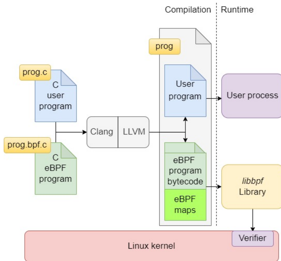
Fig. 2.9. Compilation and loading process of a program developed with libbpf.
