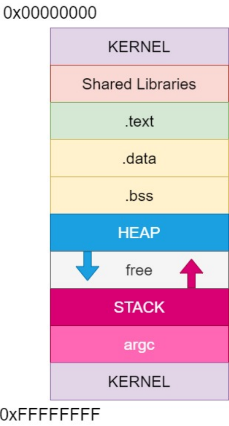
Fig. 2.13. Virtual memory architecture of a process [71].
