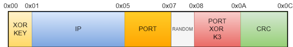
Fig. 4.23. Data payload sent by rootkit client using multi-packet trigger.
