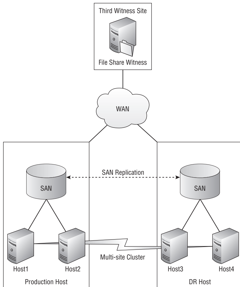
FIGURE 11.11 A File Share Witness running in a third, independently net- worked site
