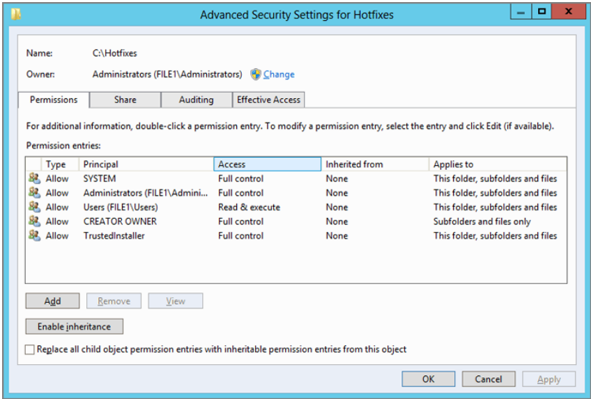
FIGURE 8.10 NTFS permissions
