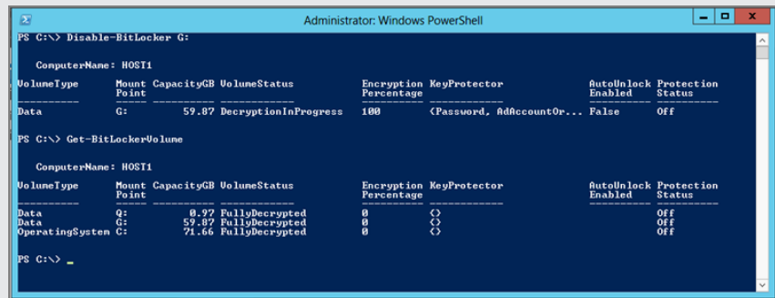
FIGURE 8.7 Disabling BitLocker
