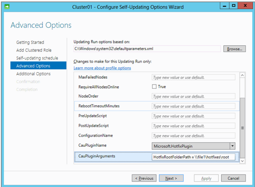
FIGURE 8.19 Advanced options
