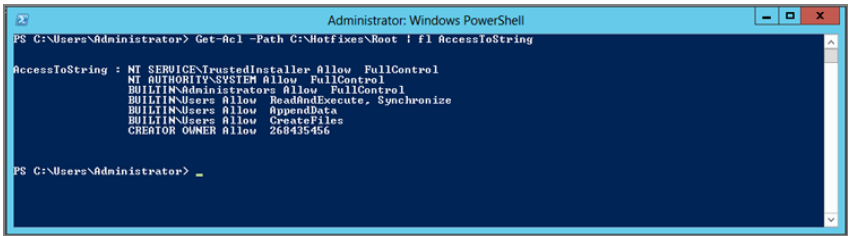
FIGURE 8.11 Get-ACL output
