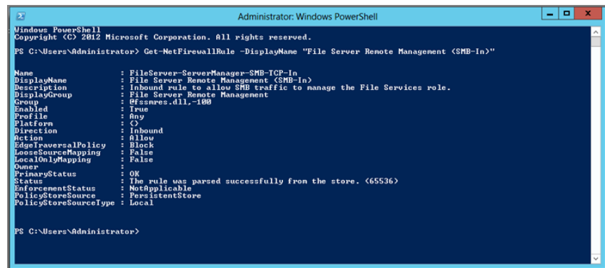
FIGURE 8.9 Get-NetFireWall- Rule output
