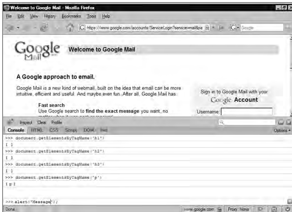
Figure 2.14 Firebug Console Screen
