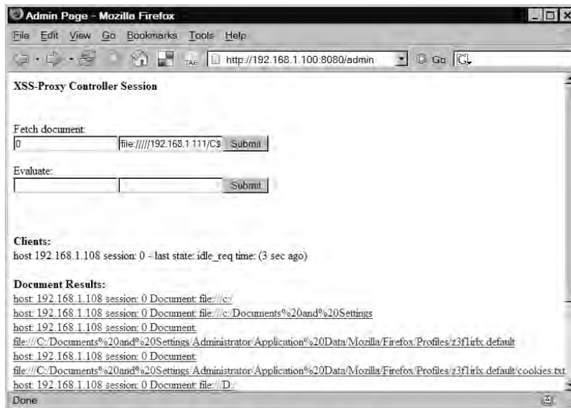
Figure 7.65 Load Document Share File
