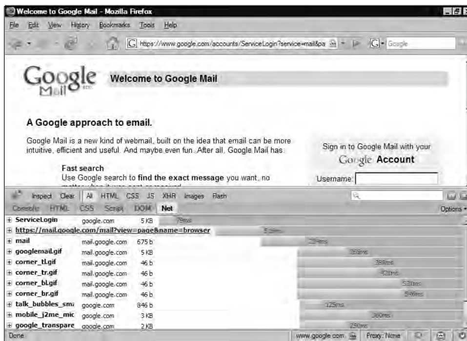
Figure 2.18 Firebug Network Screen
