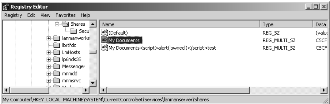
Figure 6.16 The Updated Registry
