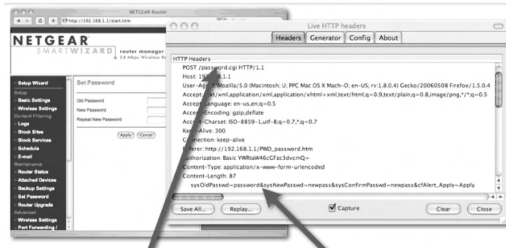
Figure 4.10 How to Change the Default Username and Password
