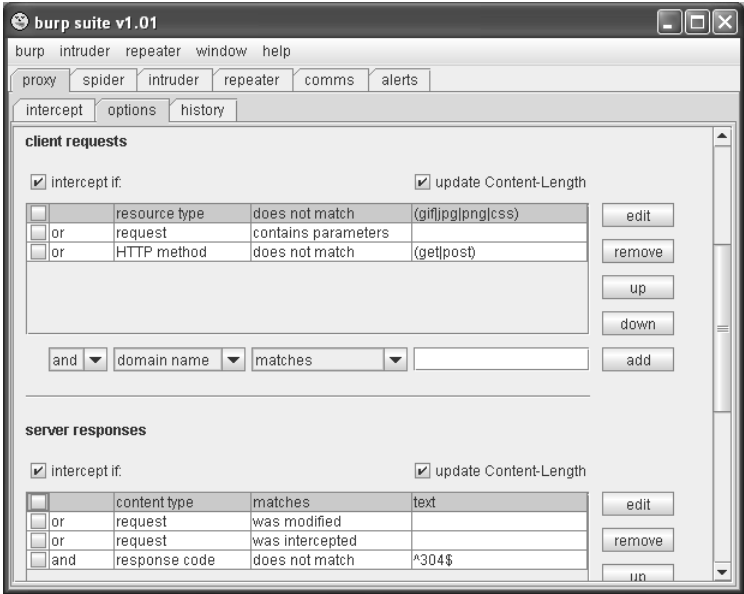
Figure 2.3 Burp Suite Proxy Options Configuration Screen
