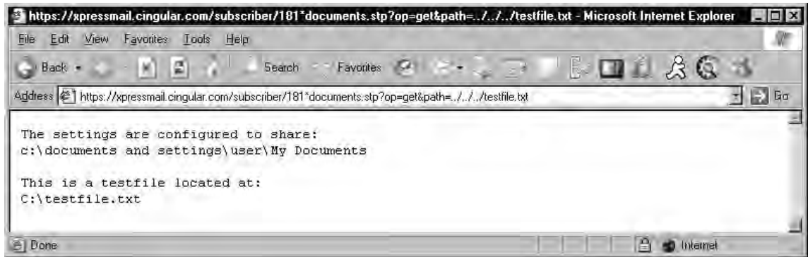
Figure 6.8 Breaking Out of the Specified Folder
