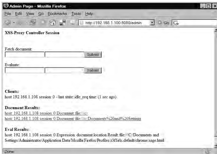
Figure 7.49 Results of Eval
