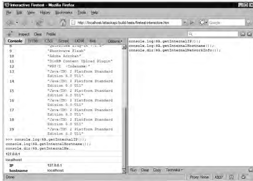
Figure 7.6 Enumerating the Network
