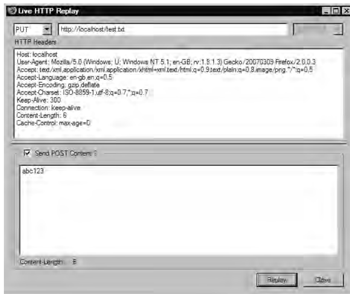
Figure 2.23 Simulating HTTP PUT with LiveHTTPHeaders
