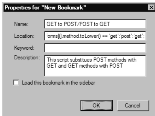
Figure 2.43 Bookmarklets Are Standard Bookmarks
