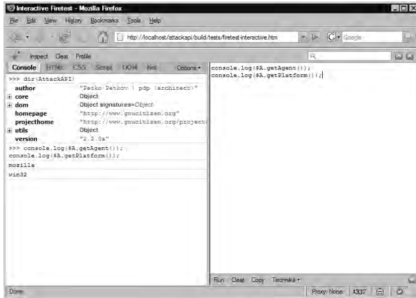
Figure 7.4 Enumerating the Platform
