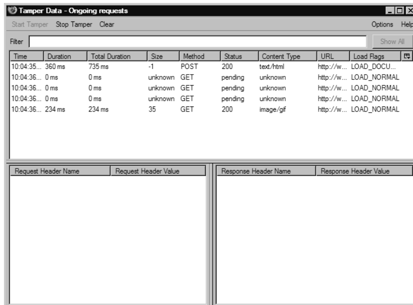
Figure 2.32 TamperData Collected Request Window
