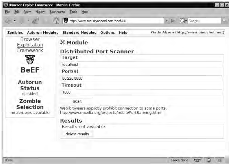
Figure 7.23 Distributed Port Scanner
