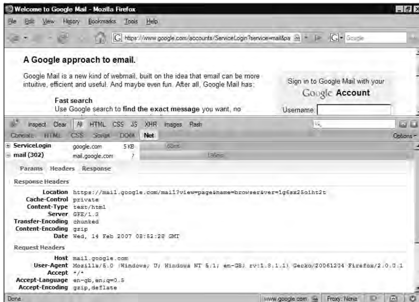
Figure 2.19 Firebug Network Requests
