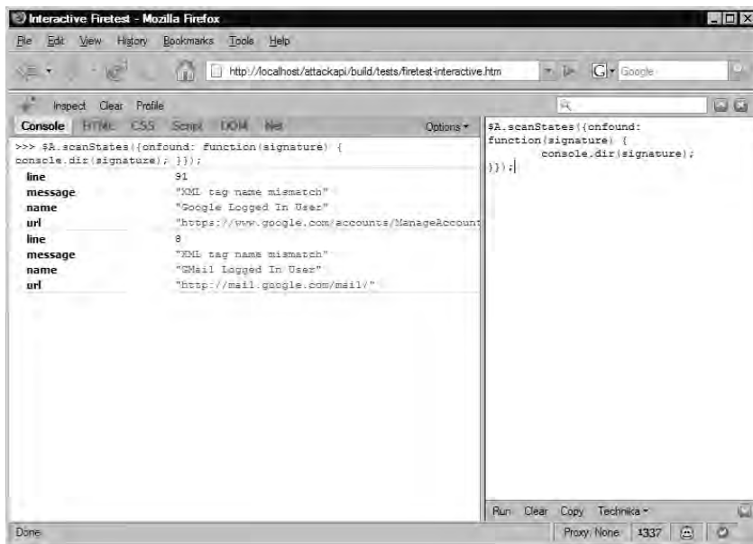
Figure 7.8 AttackAPI State Scanner
