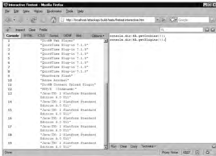
Figure 7.5 Enumerating the Cookies and Plug-ins
