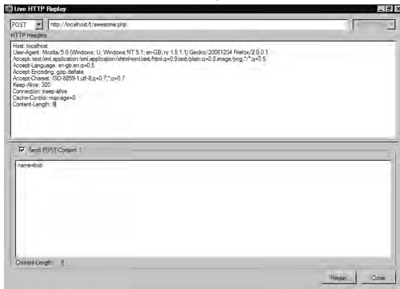
Figure 2.22 Live HTTP Headers POST Replay
