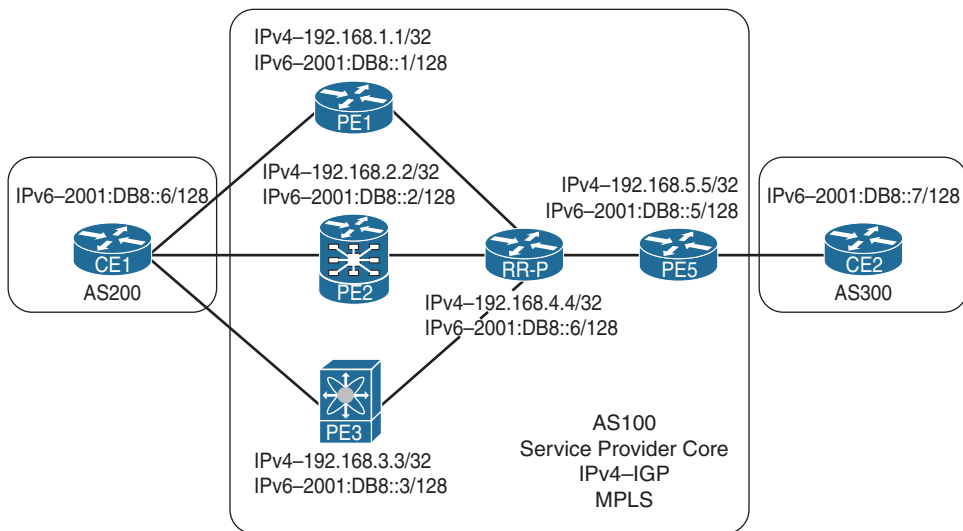
Figure 12-1 IPv6 Topology
