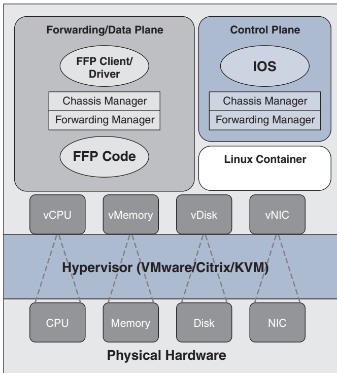
Figure 7-21 CSR1000v Architecture
