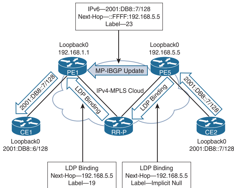
Figure 12-5 6PE Control-Plane Flow
