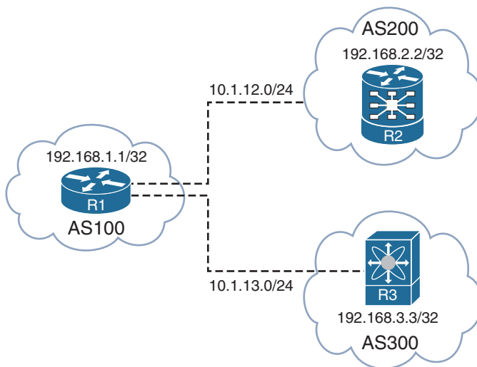
Figure 14-7 EBGPeering with BFD
