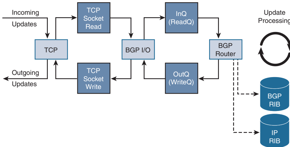
Figure 6-1 BGP Processes on Cisco IOS Software
