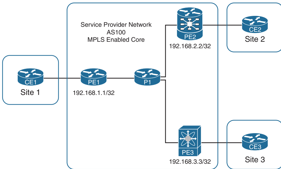
Figure 11-5 Topology
