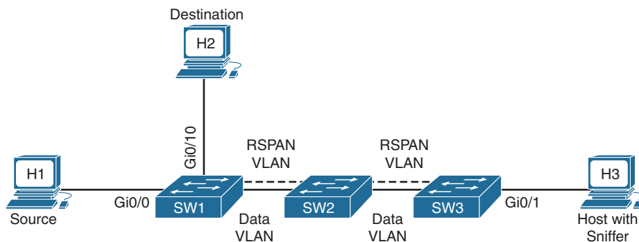
Figure 2-4 Remote SPAN
