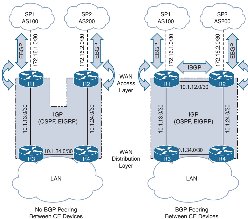
Figure 8-15 Options for Exchanging Routes Between LAN and WAN
