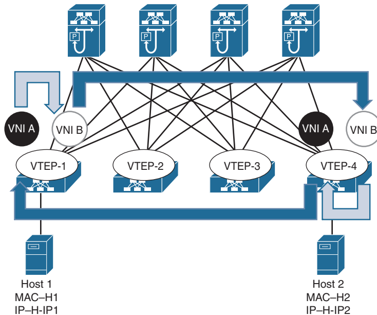
Figure 13-7 Asymmetric IRB Flow
