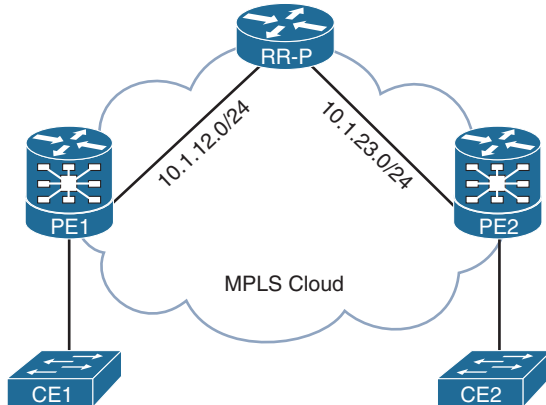
Figure 15-10 PBB-EVPN Topology
