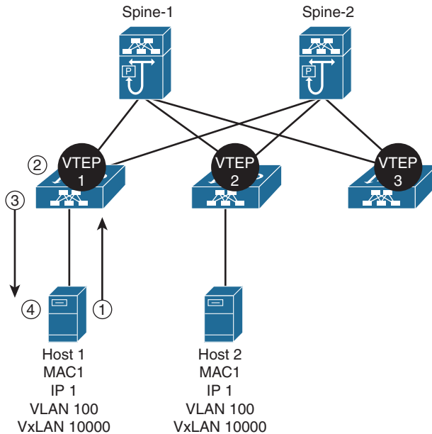
Figure 13-6 ARP Suppression
