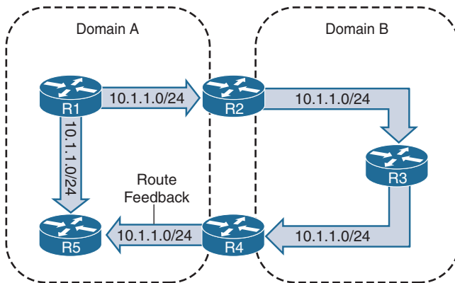
Figure 8-16 Route Feedback
