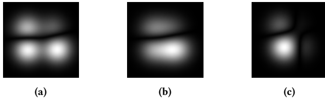
Figure 4: (a) LLSI simulation on golden layout, (b) LLSI analysis on fabricated chip, (c) difference between LLSI analysis of the fabricated IC and the golden layout.
