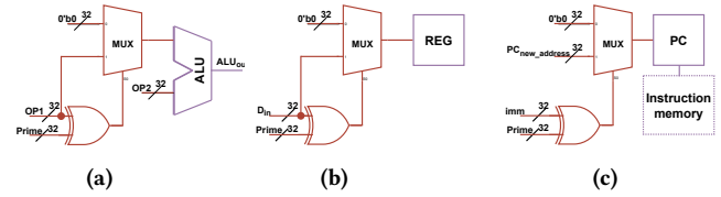
Figure 5: (a) TRJ1 is placed in the ALU, (b) TRJ2 is placed in register, (c) TRJ3 is in program counter.
