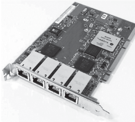
FIGURE 1.6 NIC card.
