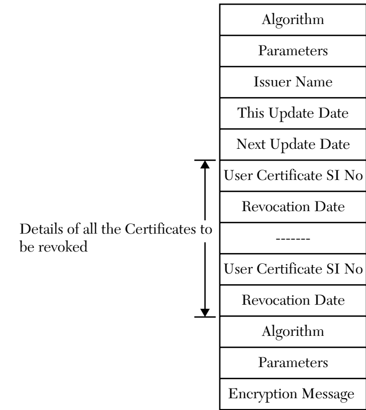
FIGURE 10.3 A schematic diagram of the format of the Certificate Revocation List.
