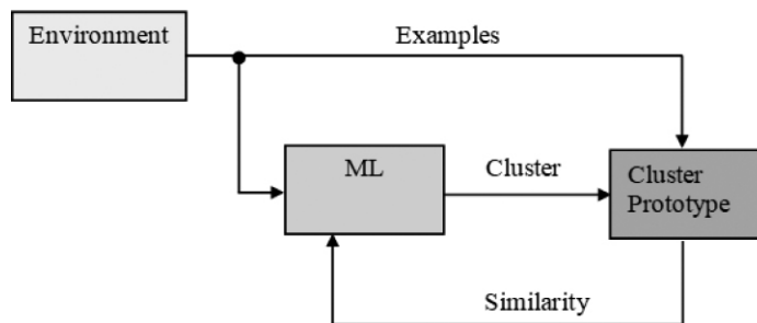
FIGURE 15.7 Unsupervised learning.
