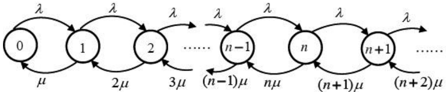
FIGURE 2.28 State transition diagram for M/M/∞ queueing system.
