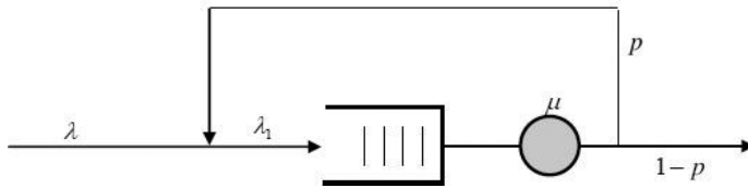
FIGURE 2.34 A queueing system with a (Bernoulli) feedback.
