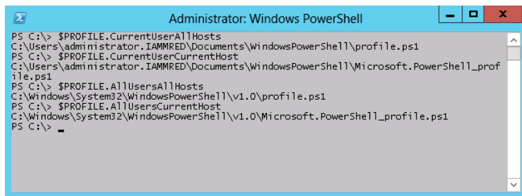
FIGURE 9-2 Use dotted notation to access the various properties of the $profile variable.
