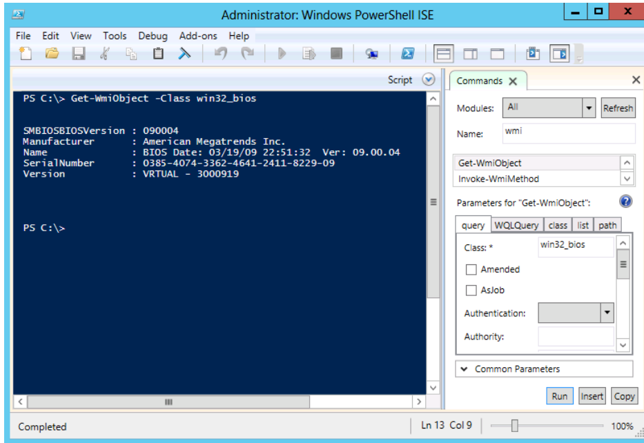
FIGURE 8-4 Select the command to run from the Commands add-on, fill out the required parameters, and click Run to execute Windows PowerShell cmdlets inside the Windows PowerShell ISE.
