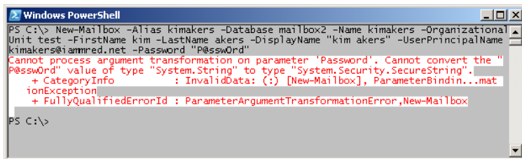
FIGURE 20-3 An error is returned when a password is supplied directly.
