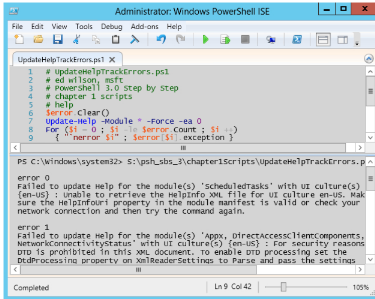
FIGURE 1-2 Cleaner error output from updatable help generated by the UpdateHelpTrackErrors script.
