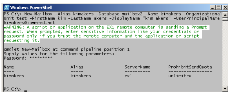
FIGURE 20-4 The New-Mailbox cmdlet prompts for the password.
