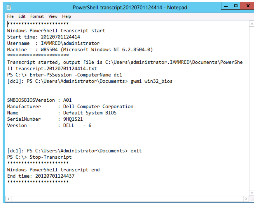
FIGURE 4-4 The Windows PowerShell transcript tool records commands and output received from a remote Windows PowerShell session.
