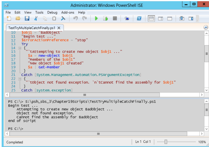
FIGURE 19-8 The Catch portion of Try...Catch...Finally catches specific errors in the order derived.
