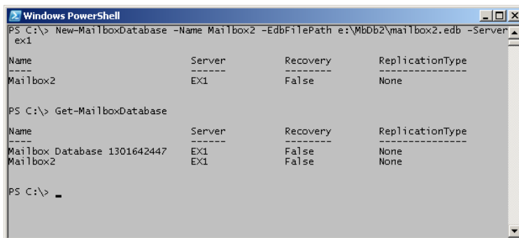
FIGURE 20-6 Creating a new mailbox database via the New-MailboxDatabase command.
