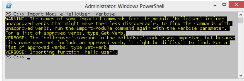
FIGURE 7-6 The -Verbose parameter of Import-Module displays information about each function exported, as well as illegal verb names. The hello verb used in Hello-User is not an approved verb.
