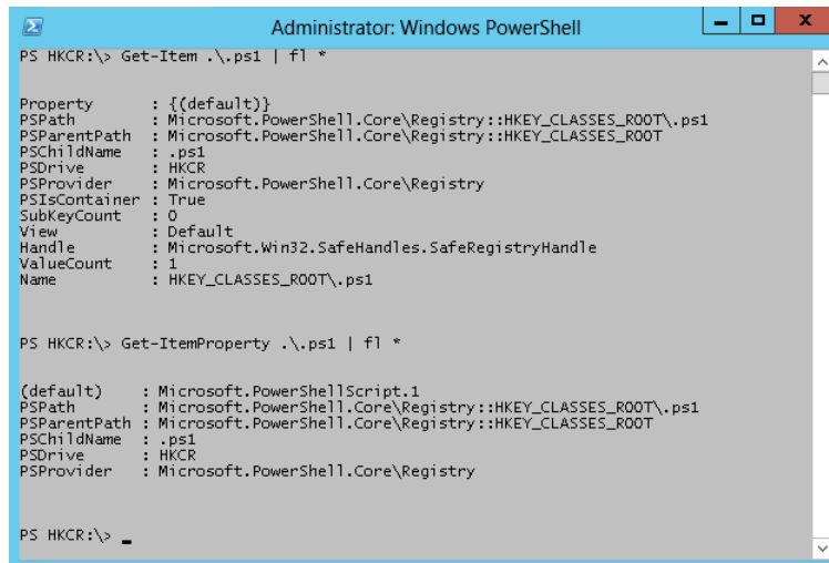
FIGURE 3-7 Use the Get-ItemProperty cmdlet to access registry property values.
