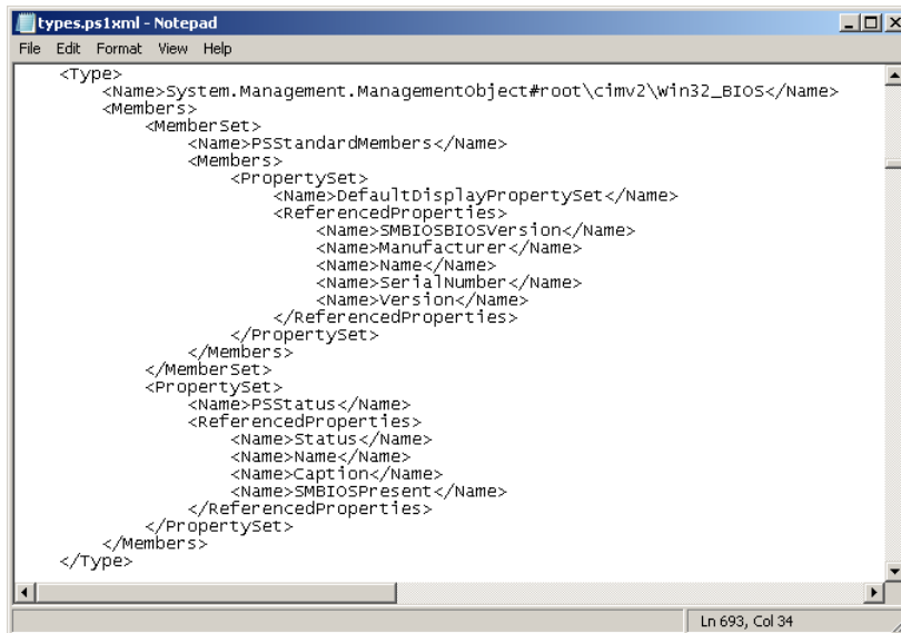
FIGURE 10-6 The Types.ps1xml file controls which properties are displayed for specific WMI classes.
