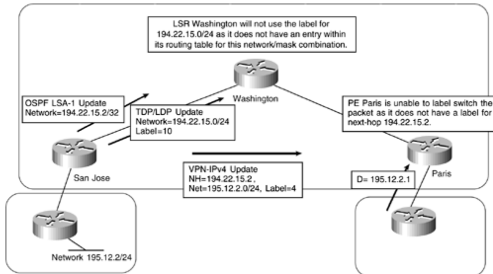
Figure 14-4. PE Loopback Address Assignment
