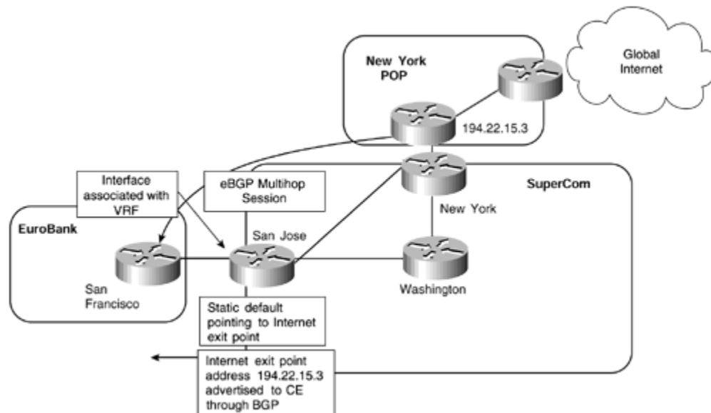
Figure 13-27. Use of eBGP Multihop for Internet Connectivity
