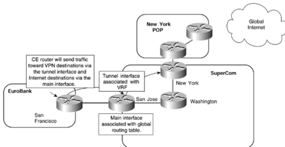
Figure 13-24. Internet Connectivity—Tunnel Interface for VPN Routes
