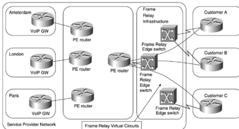
Figure 8-21. Combination of Peer-to-peer VPN with Overlay VPN
