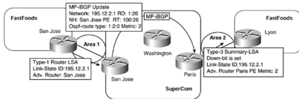
Figure 11-7. PE-to-CE Connectivity—Without Site Area 0 Support
