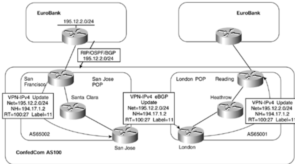
Figure 13-14. BGP Confederations—Single IGP Environment
