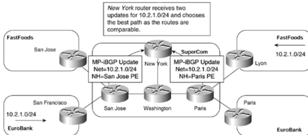
Figure 10-2. PE Router Comparison of BGP Routes
