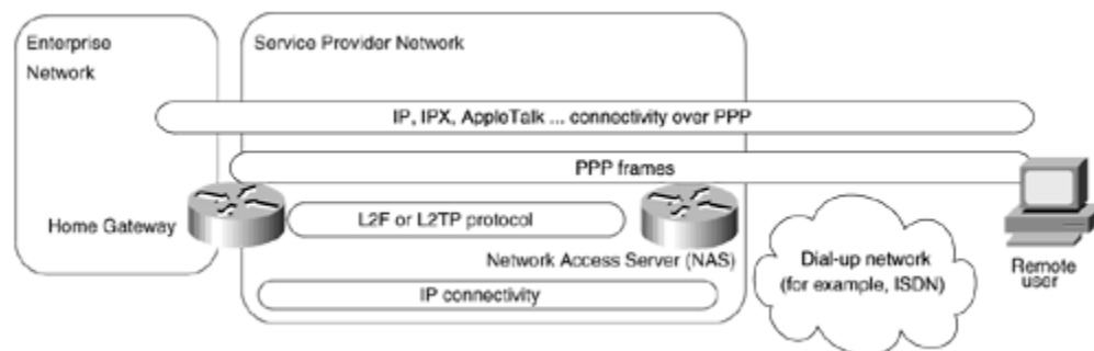
Figure 8-23. Protocol Stack in a VPDN Solution
