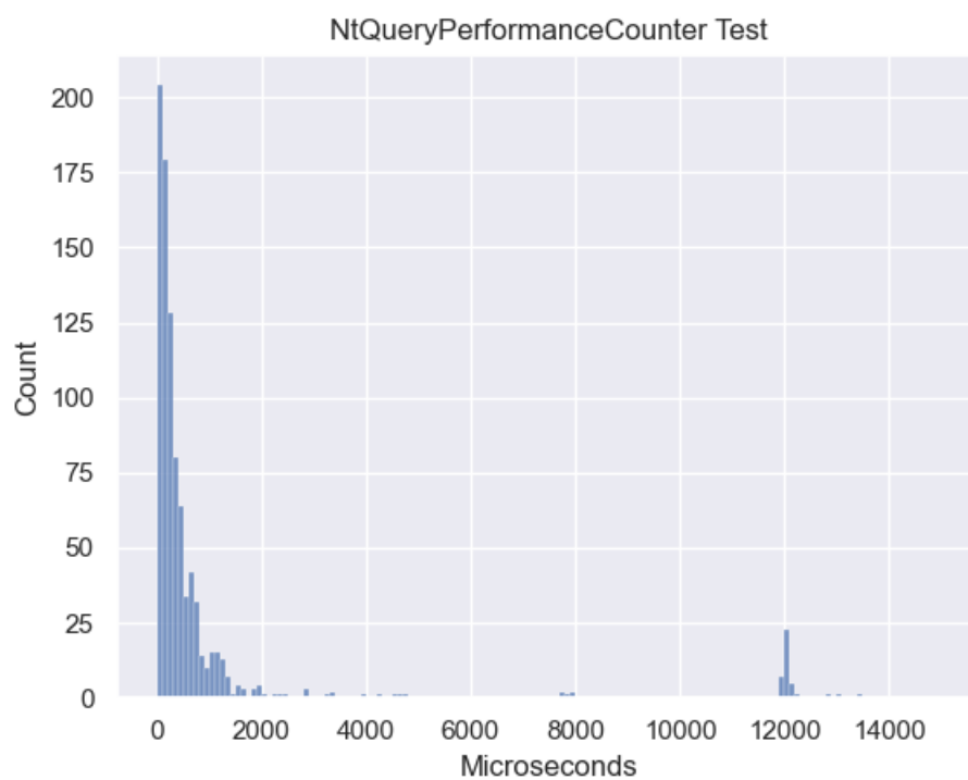
Figure 24 – NtQueryPerformanceCounter Test Distribution of Data (Windows)
