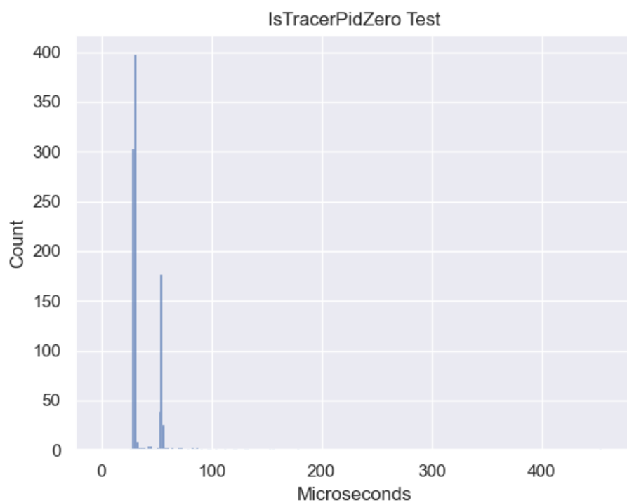
Figure 42 – IsTracerPidZero Test Distribution of Data (Linux, Intel)
