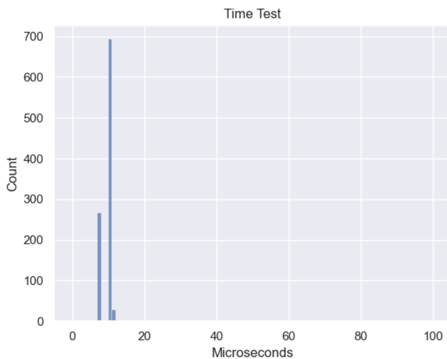
Figure 47 – Time Test Distribution of Data (Linux, Intel)
