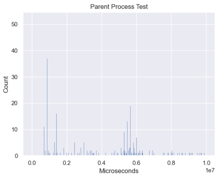
Figure 28 – Parent Process Test Distribution of Data (Windows)
