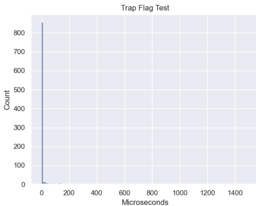
Figure 32 – Trap Flag Test Distribution of Data (Windows)
