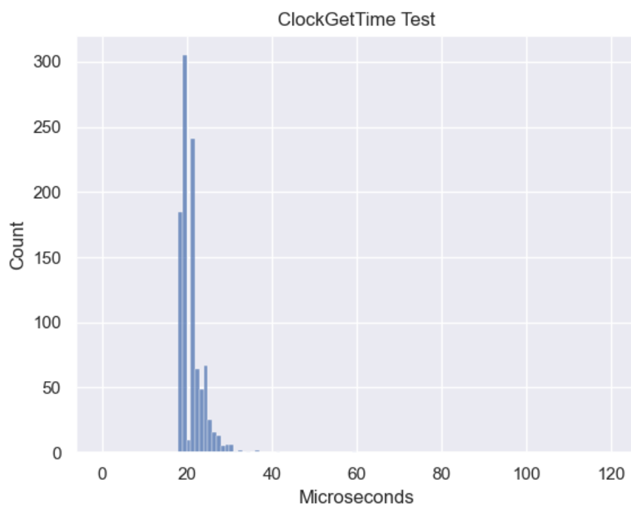
Figure 50 – ClockGetTime Test Distribution of Data (Linux, ARM)
