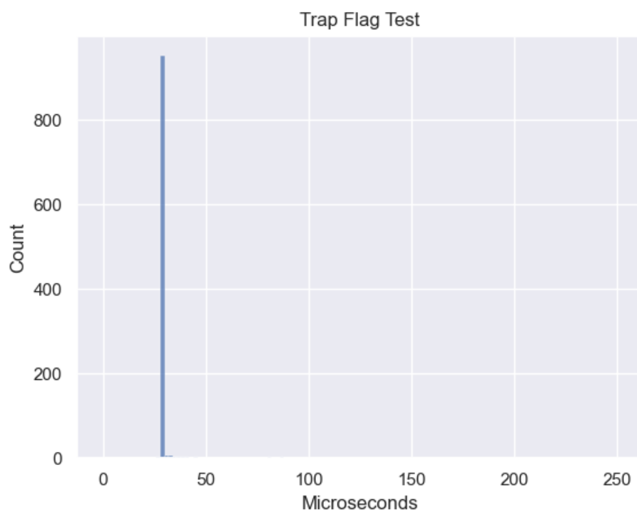
Figure 48 – Trap Flag Test Distribution of Data (Linux, Intel)
