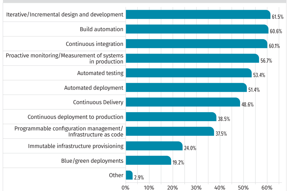
Figure 7. Technical Practices and Automation Technologies in Use
