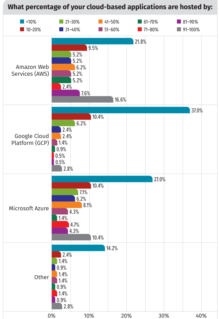
Figure 4. Cloud Hosting Providers
