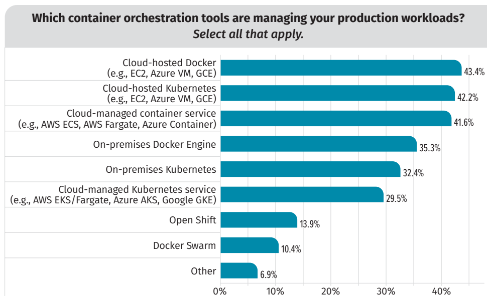
Figure 5. Container Orchestration Tools in Use
