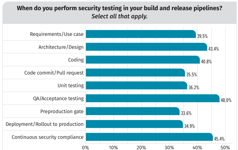
Figure 10. Timing of Security Testing in Development/Deployment
