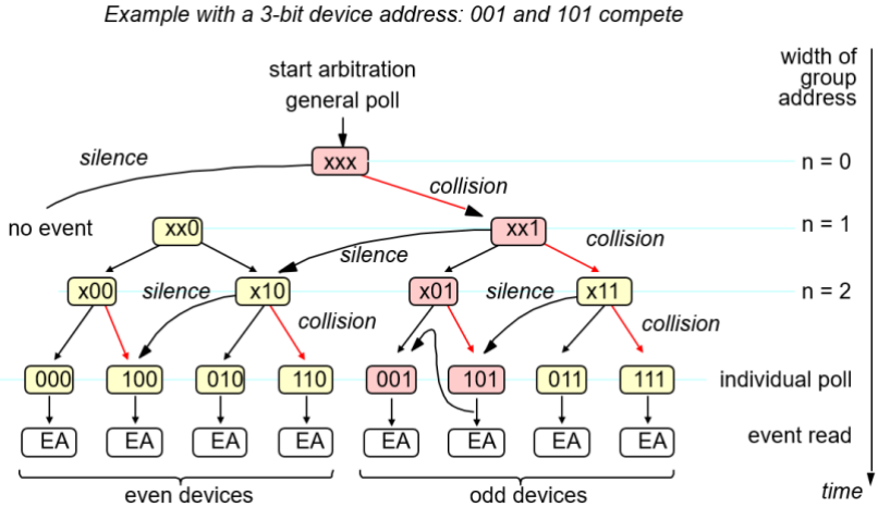
Figure 7. MVB collision resolution
