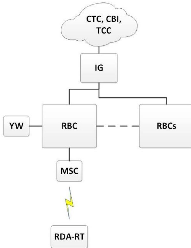
Figure 28. Interaction between CBCSs in ETCS
