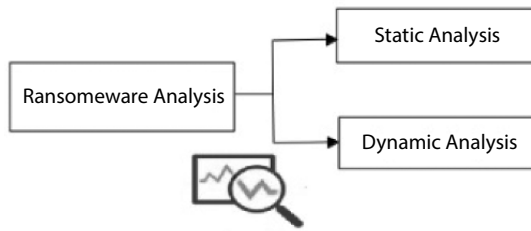
Figure 16.4 Ransomware analysis.
