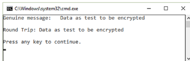
Figure 17-4. Functional encryption using X509 certificates for encryption and decryption
