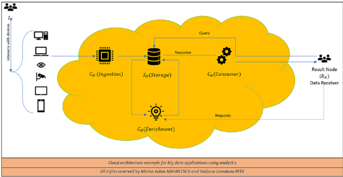
Figure 16-1. Example of cloud architecture with big-data analytics applications
