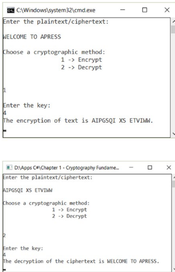
Figure 1-10. Caesar Cipher (encoding and decoding)
