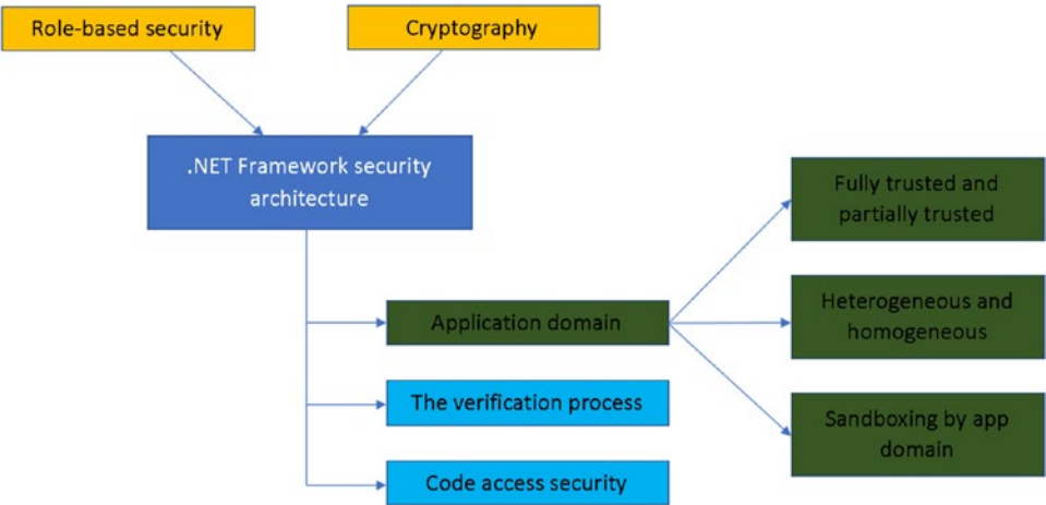
Figure 8-3. .NET Framework security architecture with application domain components
