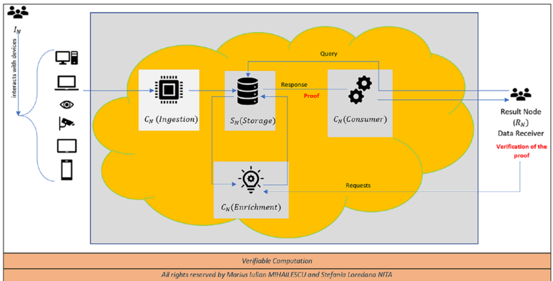
Figure 16-2. Verifiable computation scenario. The nodes of the cloud don't have any trustiness level for integrity protection.
