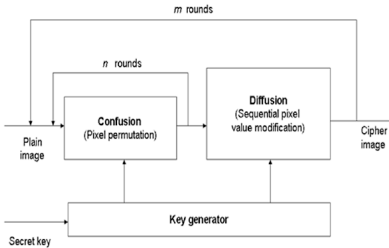
Figure 15-3. Block diagram for image encryption cryptosystem [15]
