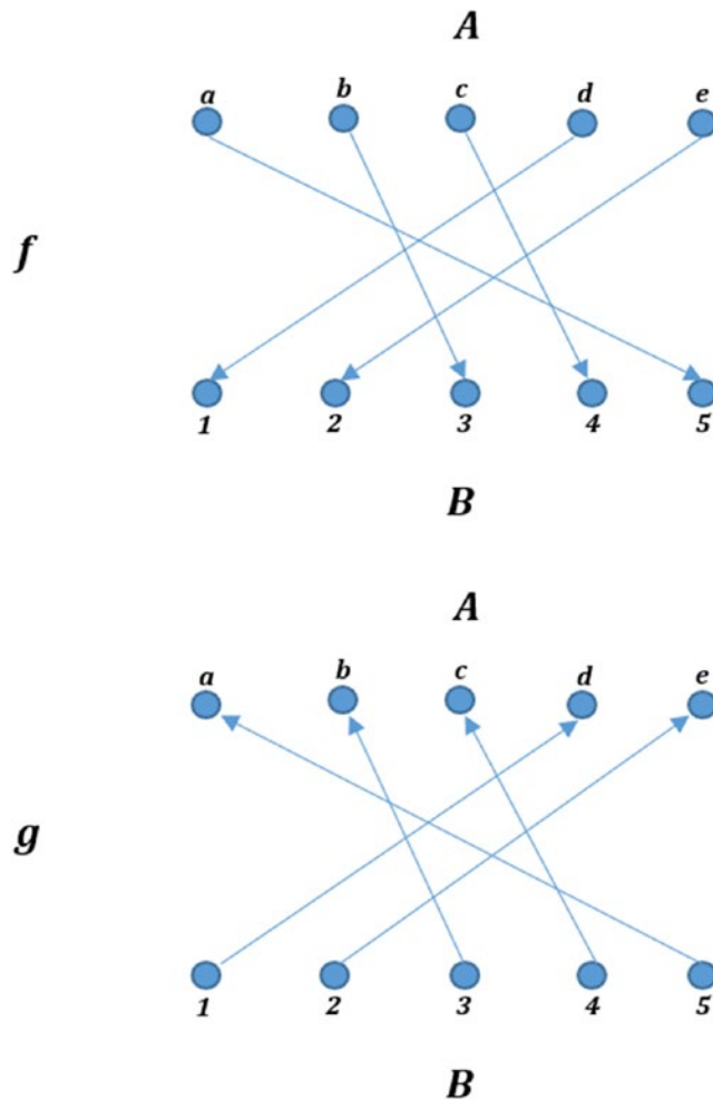
Figure 1-3. Representation of bijection f and its inverse, g = f^{-1}
