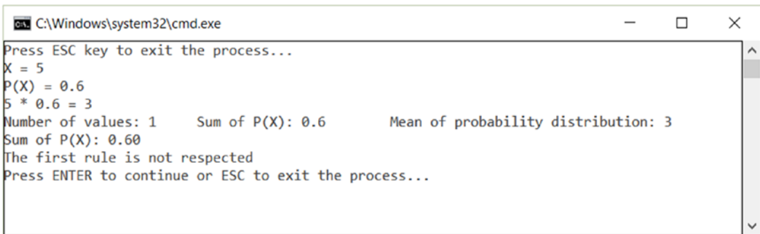
Figure 2-3. Computing the mean of probability distribution
