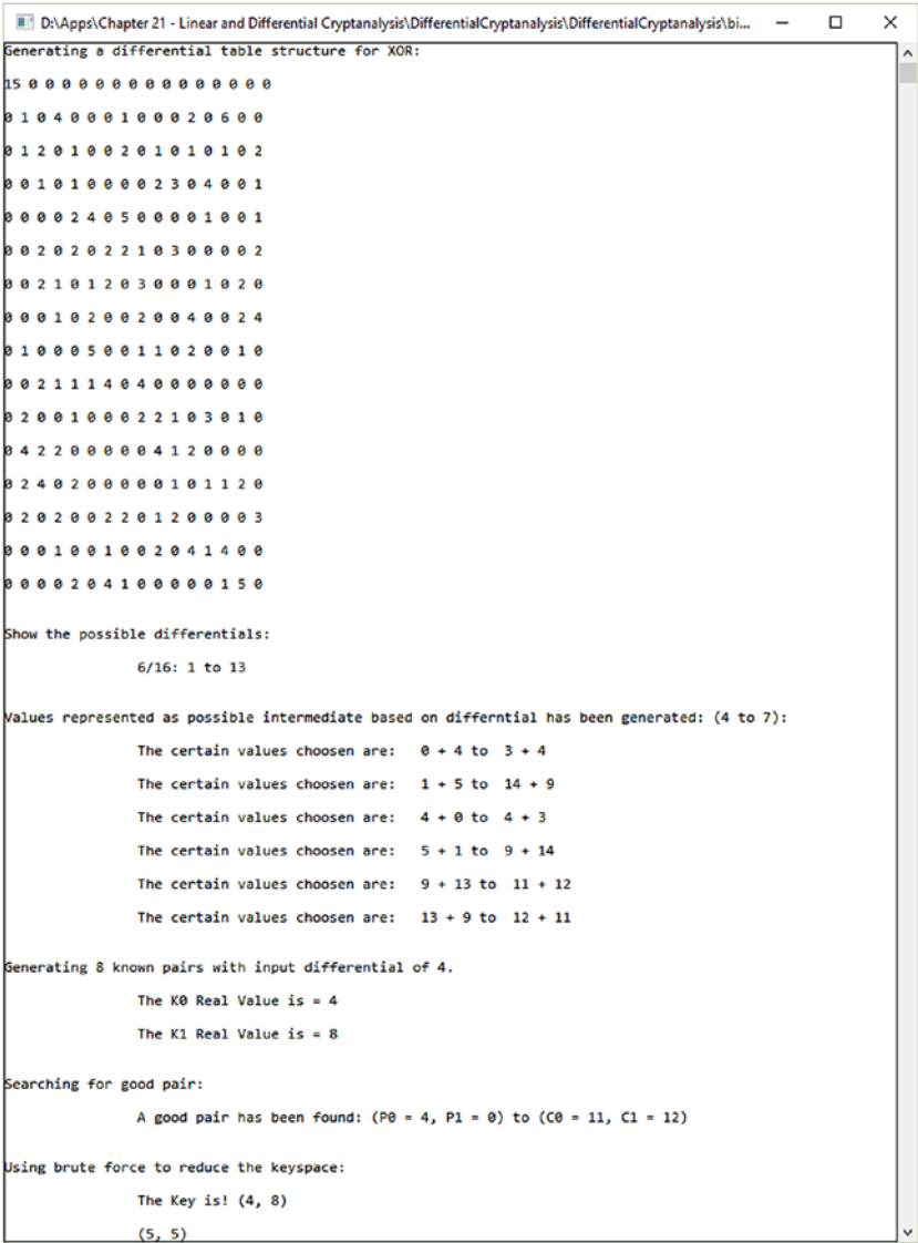
Figure 20-1. Differential cyptanalysis example
