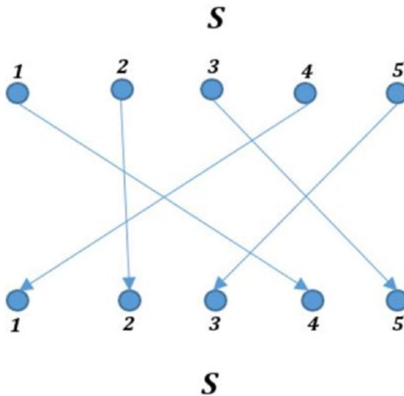
Figure 1-4. Representation of an involution with a set of S with five elements
