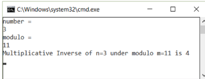
Figure 2-9. Modular multiplicative inverse application
