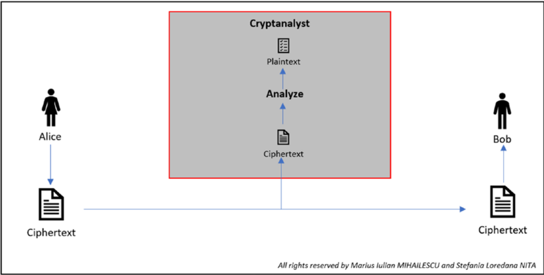
Figure 24-2. COA representation
