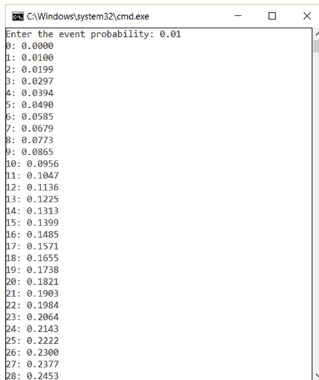
Figure 2-1. Computing the probability application form
