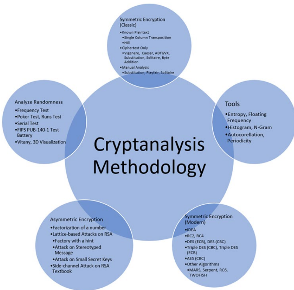
Figure 24-1. Cryptanalysis methodology
