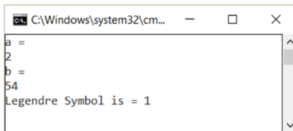
Figure 2-11. Computation of the Legendre Symbol
