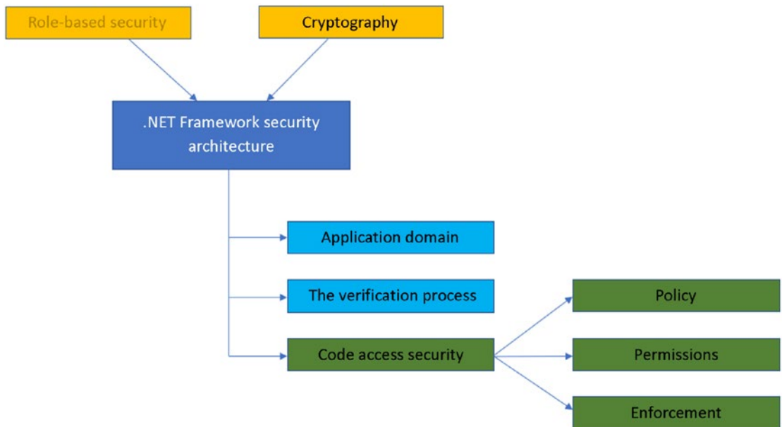
Figure 8-7. The .NET Framework security architecture with the code access security components
