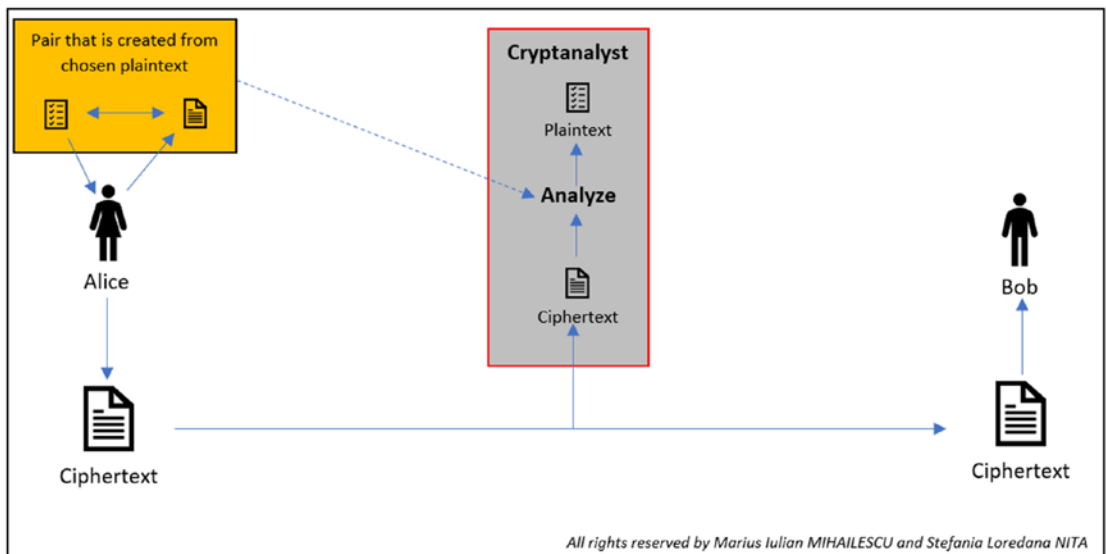
Figure 24-4. CPA representation
