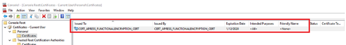
Figure 17-3. Importing certificates
