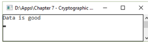
Figure 7-10. Digital signature
