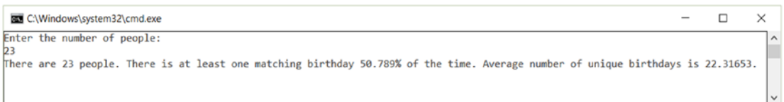
Figure 2-6. Birthday paradox application
