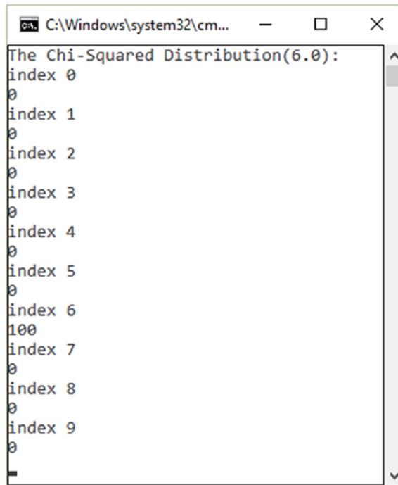
Figure 23-1. Chi-distribution output
