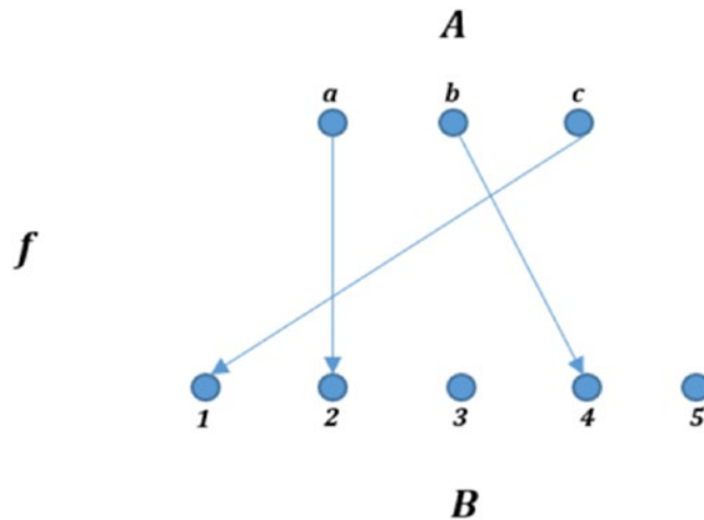
Figure 1-2. Function f from a set A formed from three elements to a set B formed from five elements
