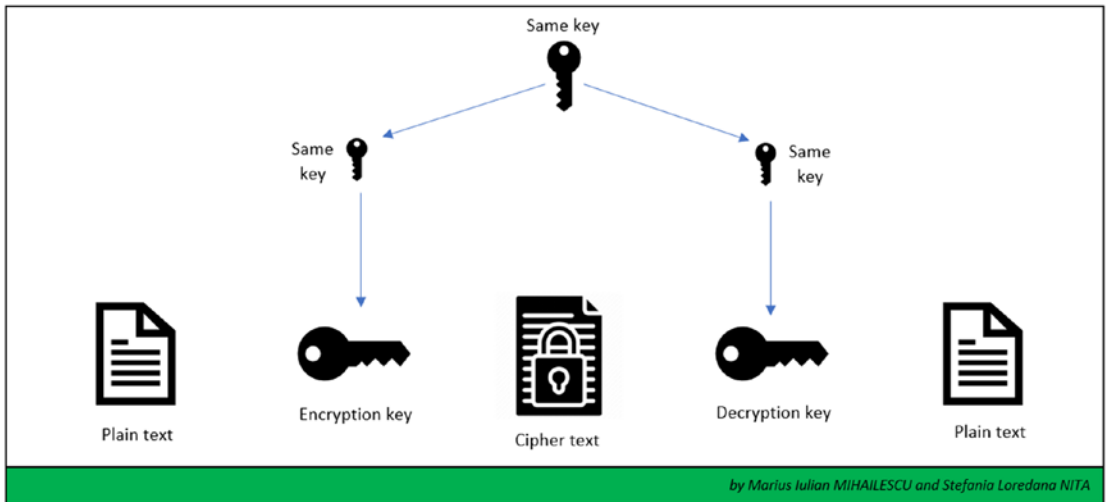
Figure 7-1. Symmetric encryption
