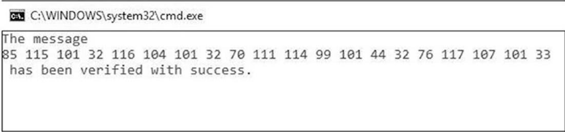
Figure 9-1. NSec output
