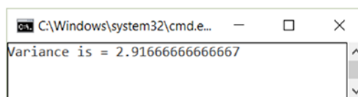
Figure 2-4. Calculating the variance
