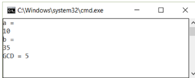
Figure 2-7. Euclidean Algorithm application form
