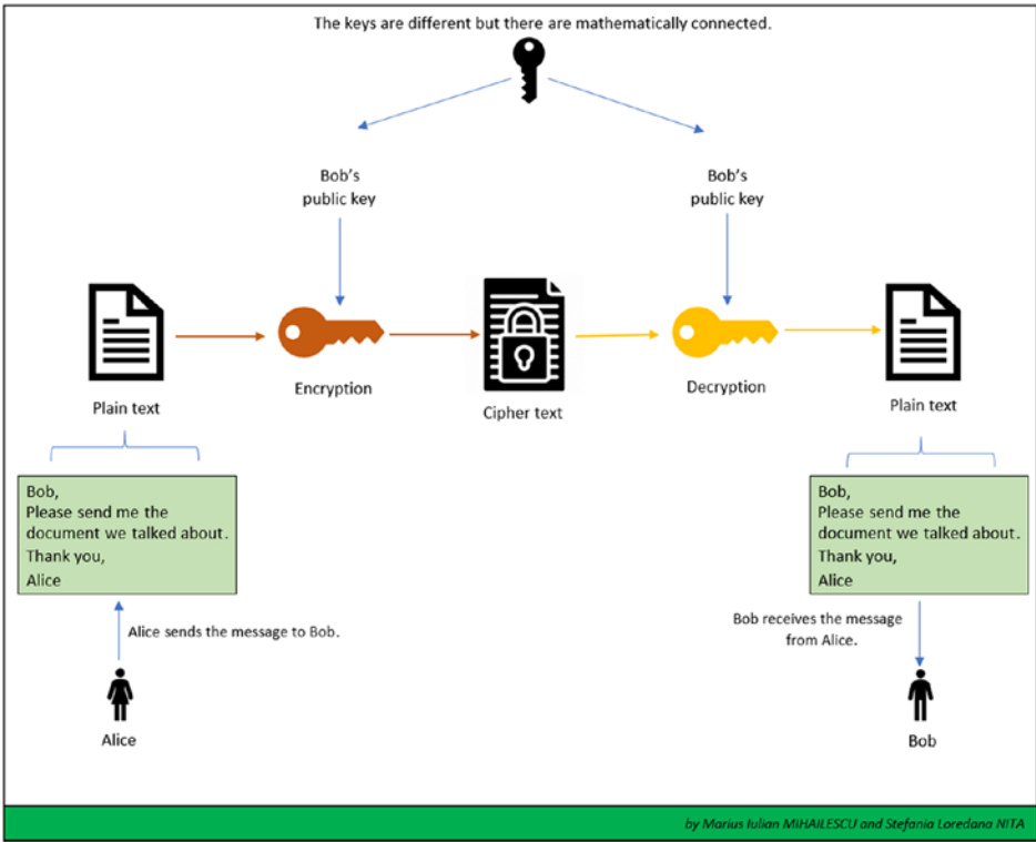
Figure 7-7. Public-key encryption
