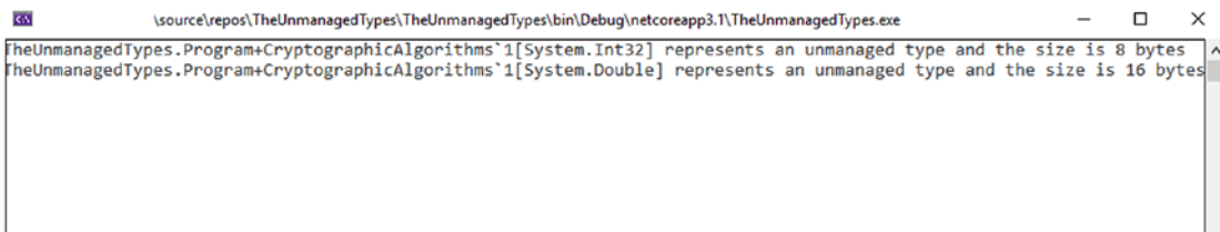
Figure 5-10. The result of Listing 5-17
