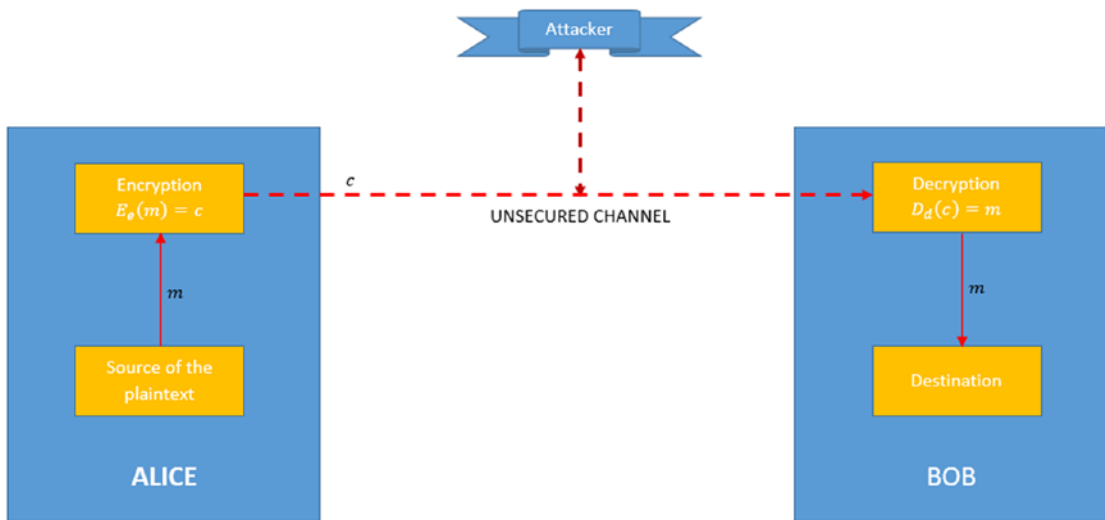
Figure 1-5. Two-party communication process using encryption
