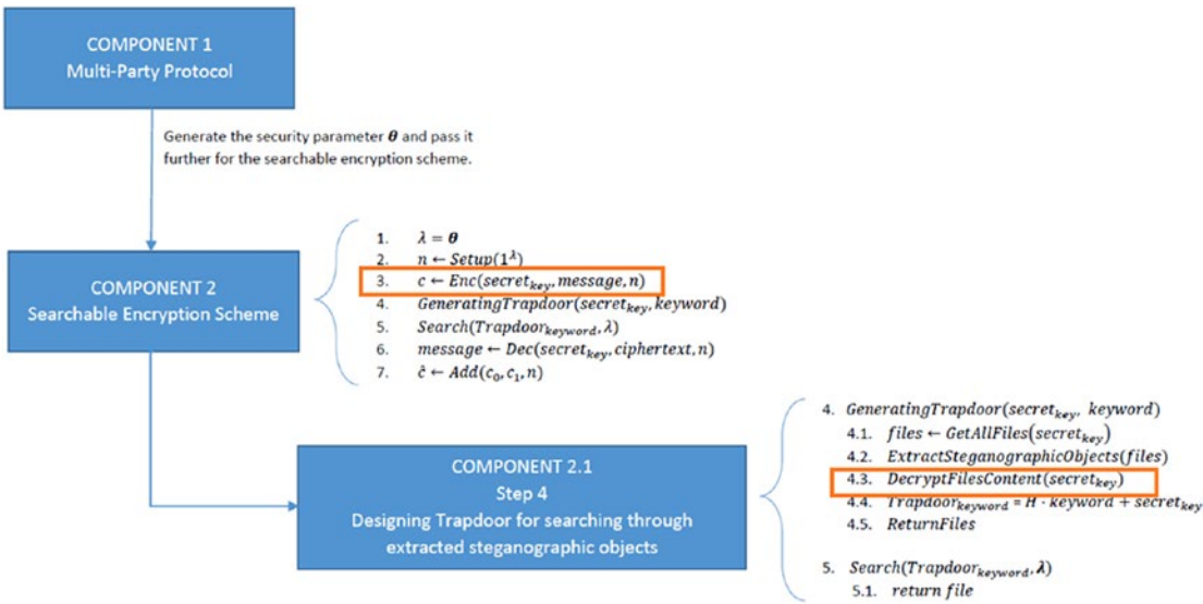
Figure 16-5. MPC in big data
