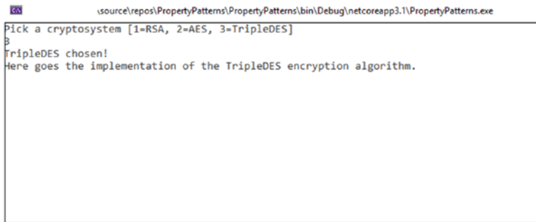
Figure 5-3. The result of the code in Listing 5-6
