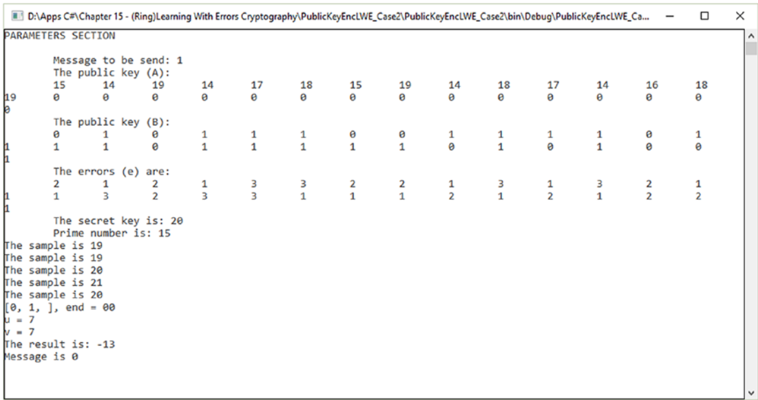
Figure 14-2. The output of public key encryption example using LWE
