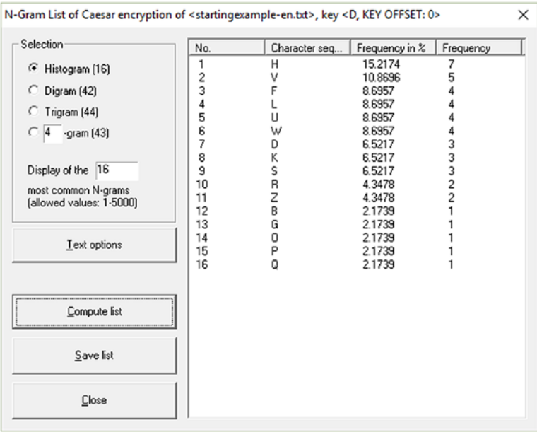
Figure 23-2. Letter frequency for encrypted text
