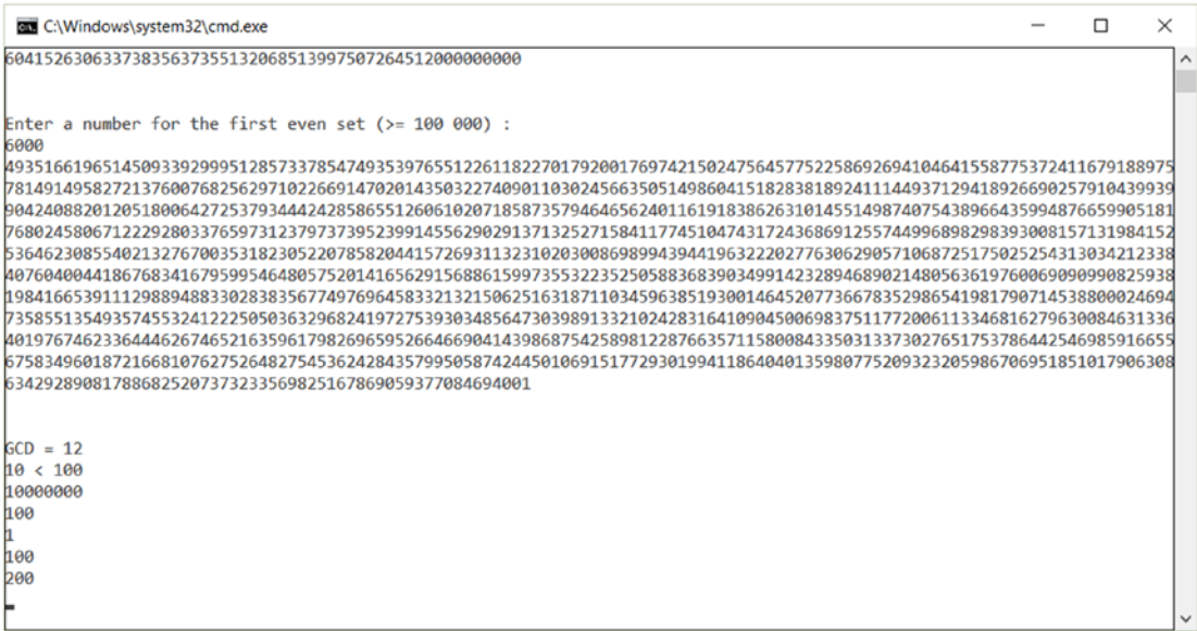
Figure 3-1. BigInteger example for computing GCD
