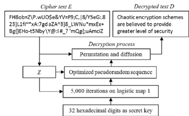
Figure 15-2. Block diagram for text encryption using logistic map [14]
