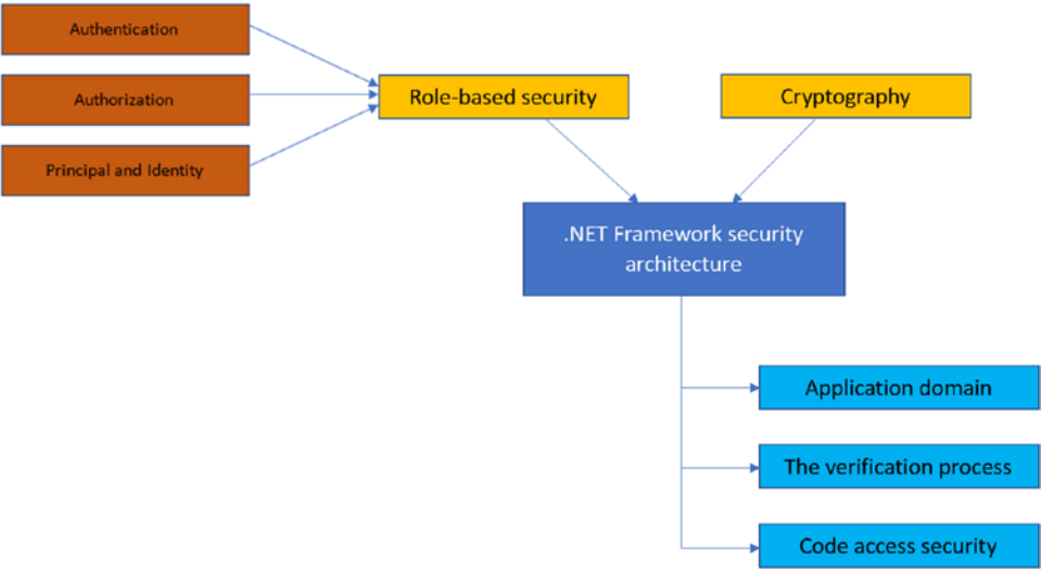
Figure 8-2. .NET Framework security architecture with role-based security
