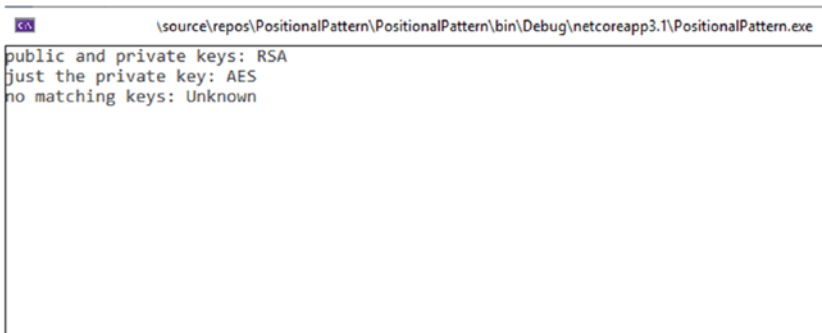
Figure 5-5. The result of Listing 5-8
