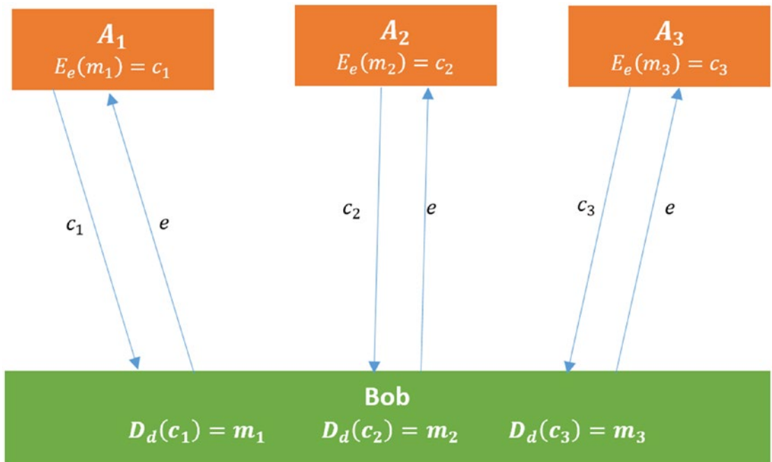
Figure 1-7. How public-key encryption is used
