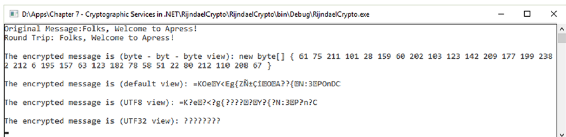
Figure 7-3. Example of RijndaelManaged
