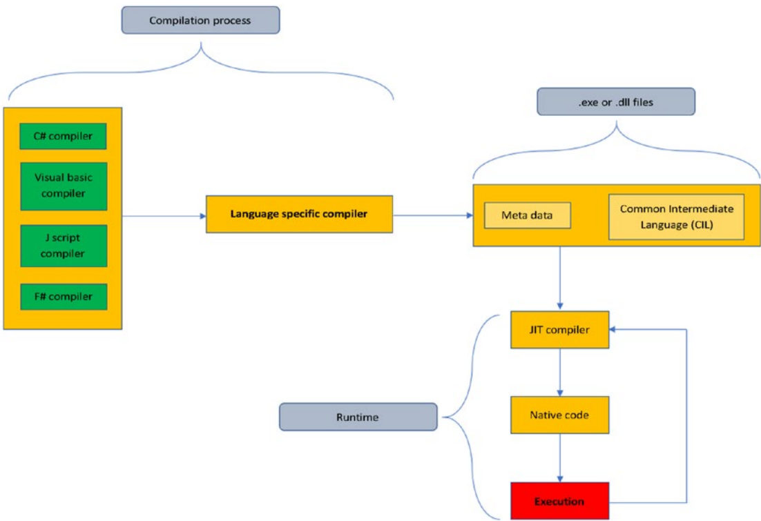
Figure 8-6. JIT compilation process
