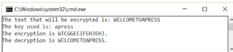
Figure 1-11. Vigenère Cipher, encryption and decryption operations
