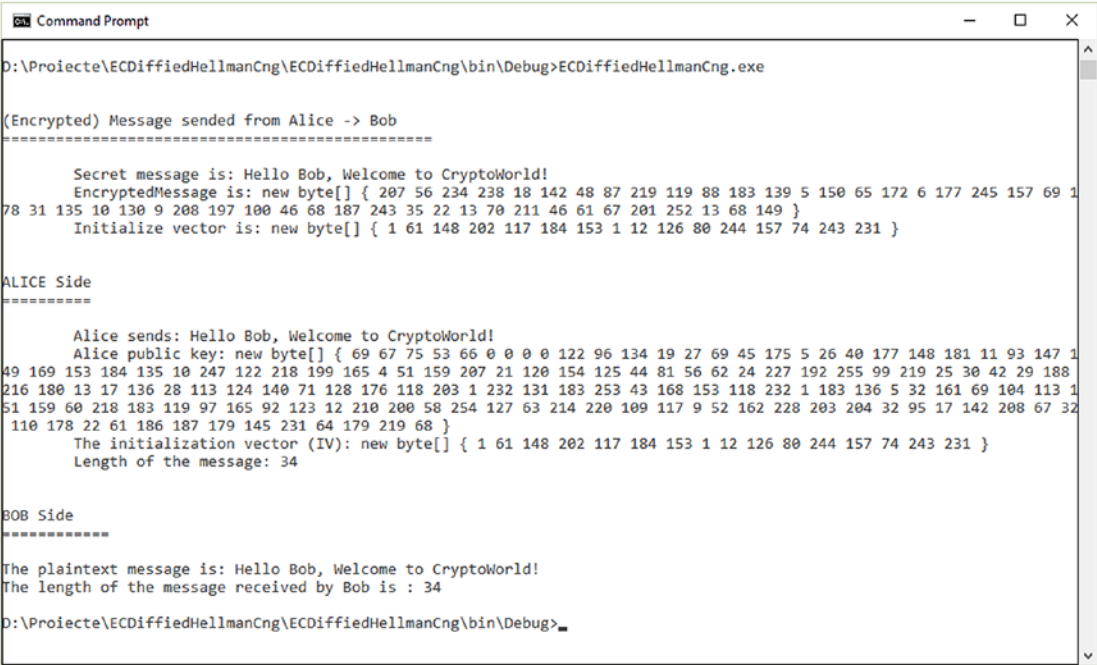
Figure 10-1. Output of encryption using ECDiffieHellmanCng
