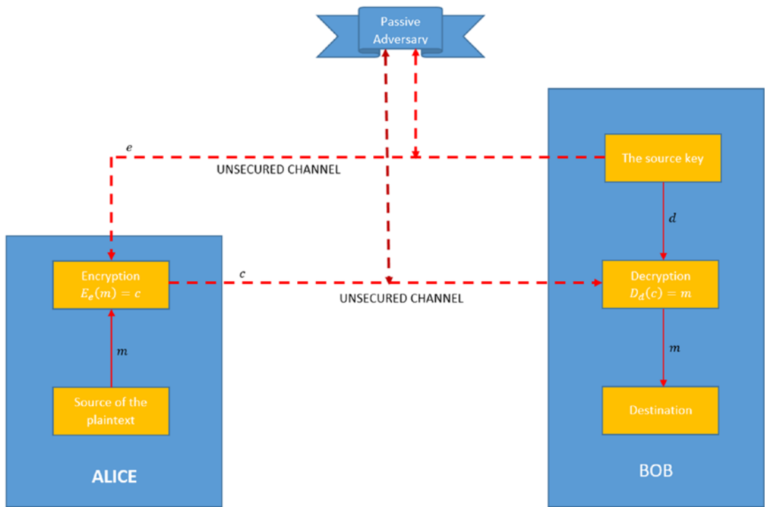
Figure 1-6. The process of encryption using public-key mechanism
