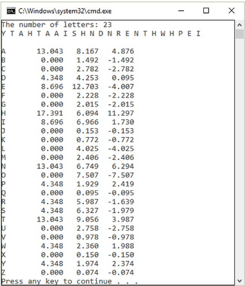
Figure 23-3. Encryption letter frequency (%) 2
