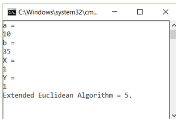
Figure 2-8. Extended Euclidean Algorithm application form
