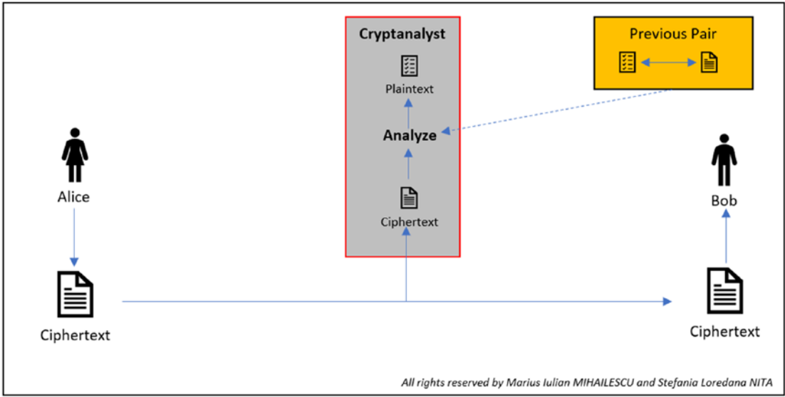
Figure 24-3. KPA representation
