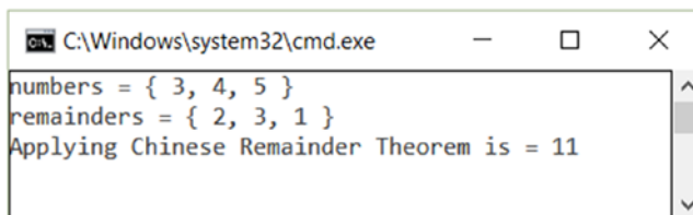
Figure 2-10. Chinese Remainder Theorem application
