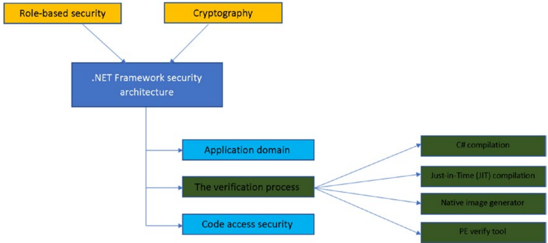
Figure 8-5. .NET Framework security architecture with the verification process components
