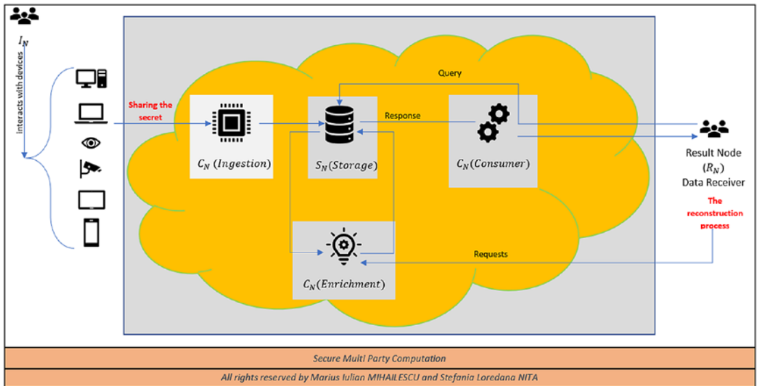
Figure 16-4. Secure multi-party computation
