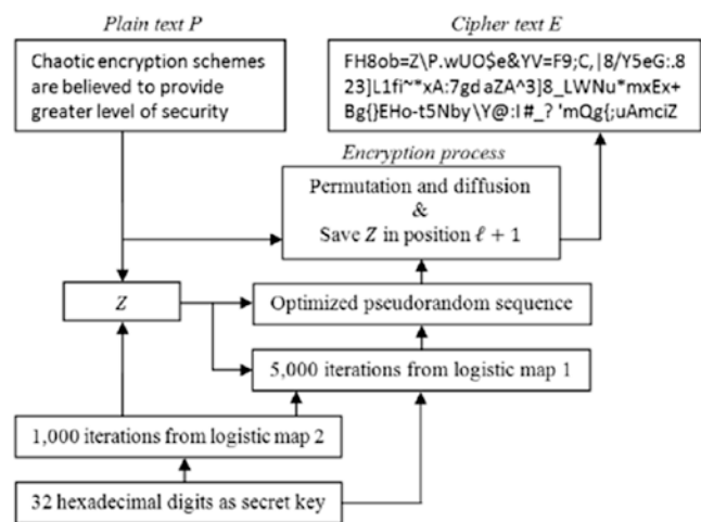
Figure 15-1. Block diagram for text encryption using logistic map [14]
