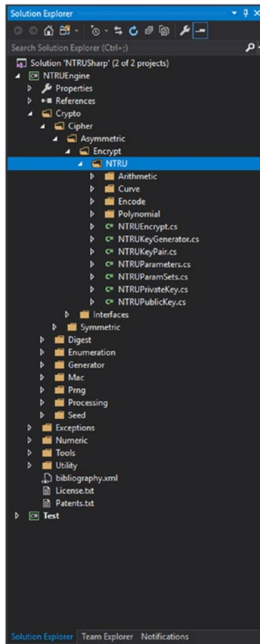
Figure 11-1. NTRU library structure
