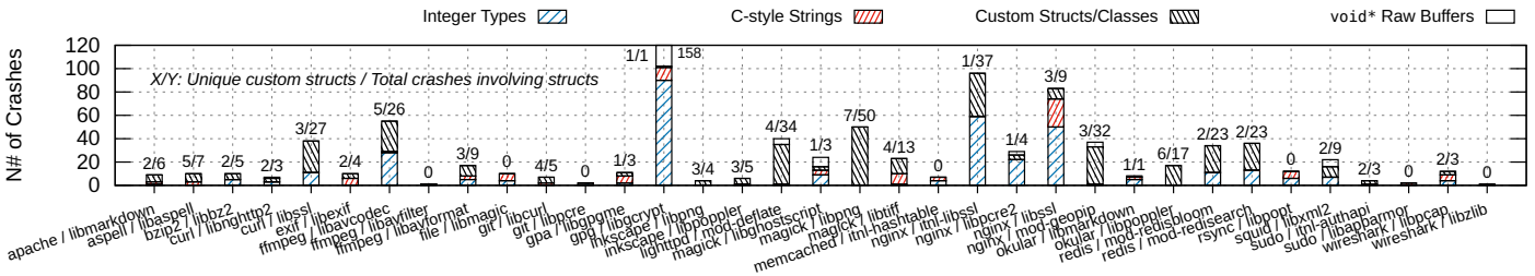
Fig. 3: High-level type classes involved in CIVs for each scenario.
