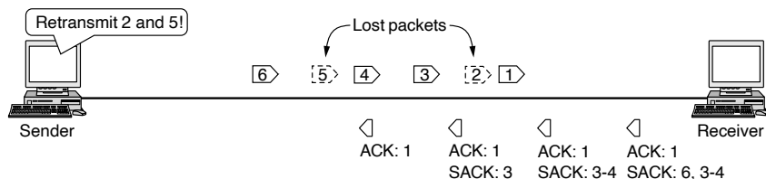
Figure 6-48. Selective acknowledgements.
