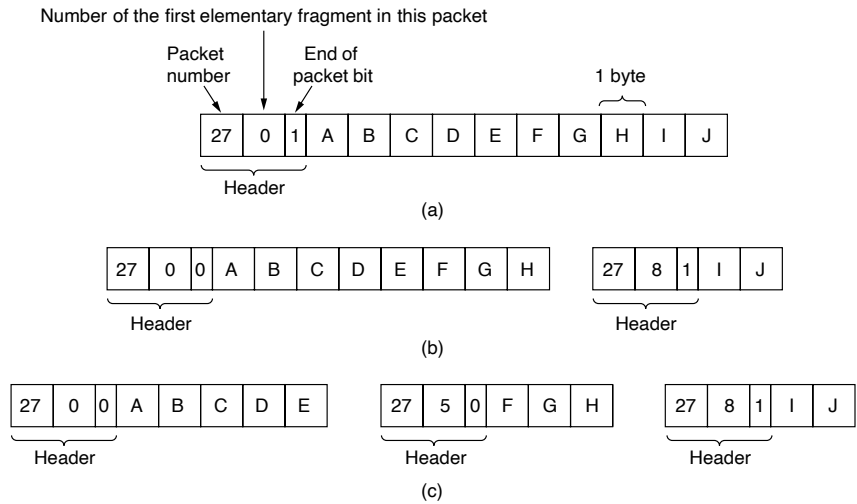
Figure 5-41. Fragmentation when the elementary data size is 1 byte. (a) Original packet, containing 10 data bytes. (b) Fragments after passing through a network with maximum packet size of 8 payload bytes plus header. (c) Fragments after passing through a size 5 gateway.
