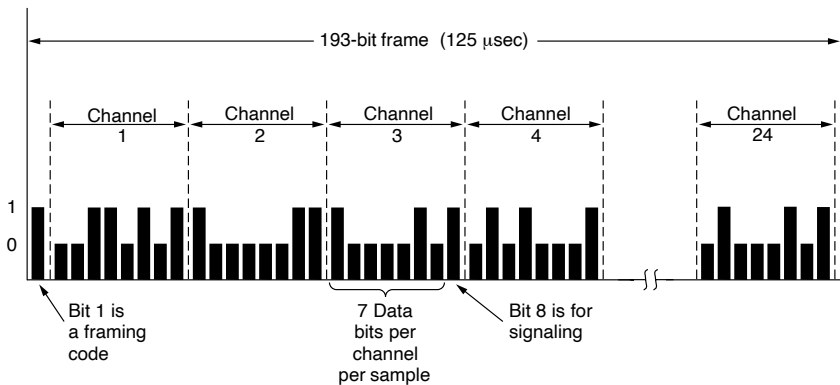
Figure 2-32. The T1 carrier (1.544 Mbps).
