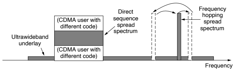
Figure 2-9. Spread spectrum and ultra-wideband (UWB) communication.
