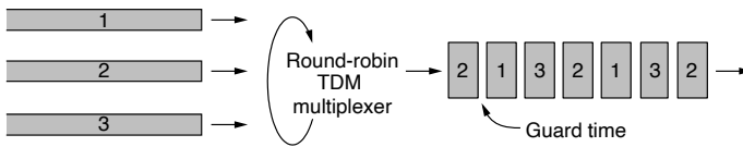
Figure 2-21. Time Division Multiplexing (TDM).
