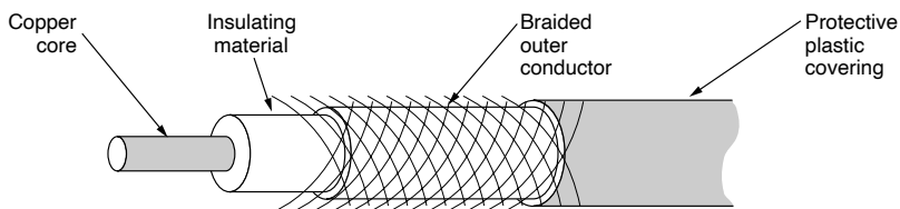
Figure 2-2. A coaxial cable.
