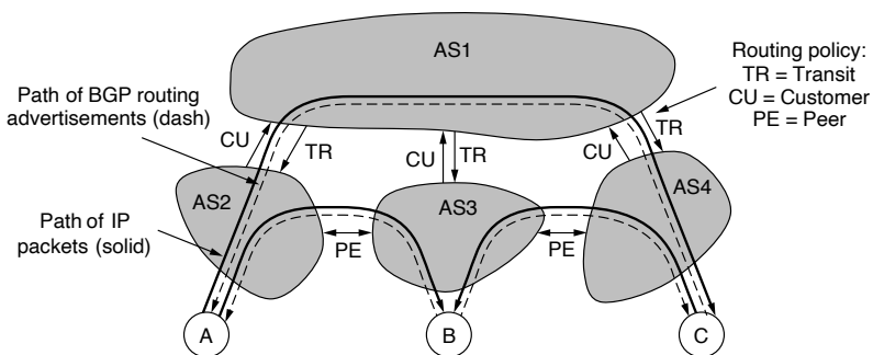
Figure 5-68. Routing policies between four autonomous systems.
