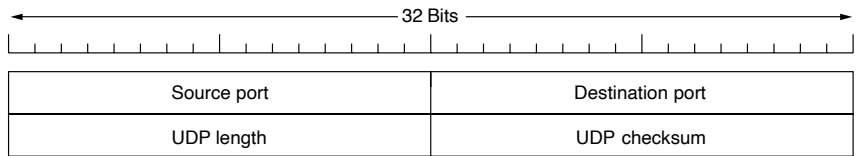
Figure 6-27. The UDP header.
