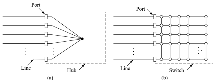
Figure 4-17. (a) Hub. (b) Switch.
