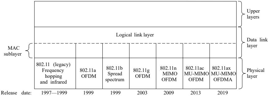
Figure 4-24. Part of the 802.11 protocol stack.
