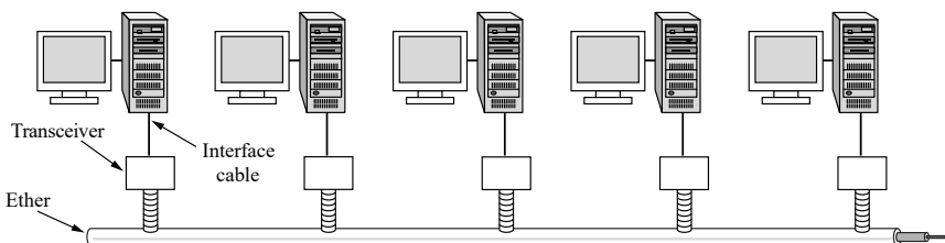
Figure 4-13. Architecture of classic Ethernet.
