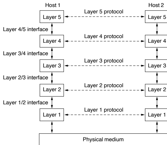
Figure 1-25. Layers, protocols, and interfaces.
