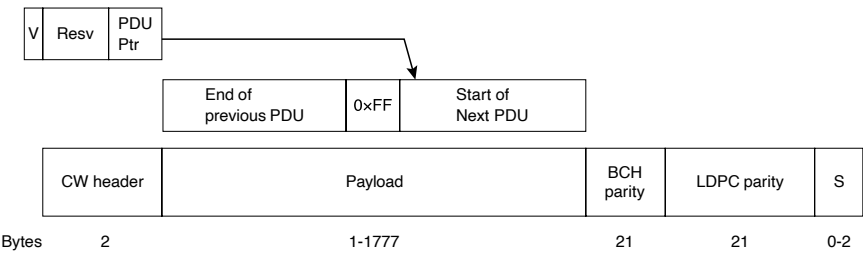
Figure 3-28. DOCSIS Frame to codeword mapping.
