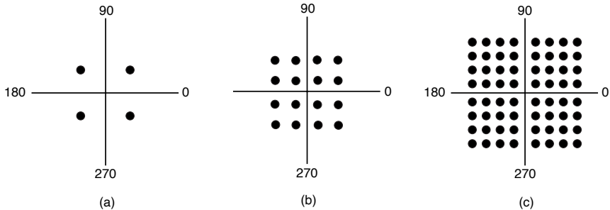
Figure 2-17. (a) QPSK. (b) QAM-16. (c) QAM-64.
