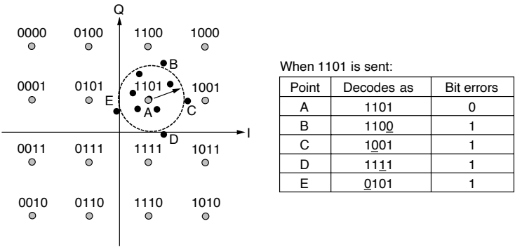
Figure 2-18. Gray-coded QAM-16.
