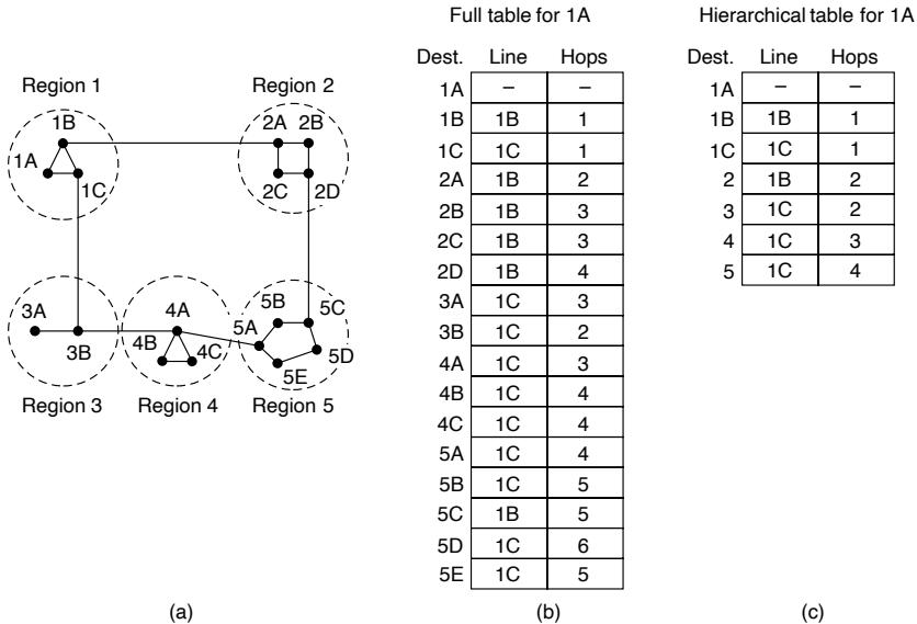
Figure 5-14. Hierarchical routing.
