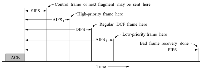
Figure 4-28. Interframe spacing in 802.11.
