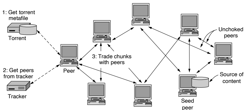
Figure 7-47. BitTorrent.
