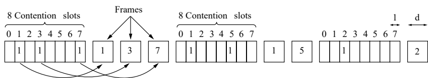
Figure 4-6. The basic bit-map protocol.
