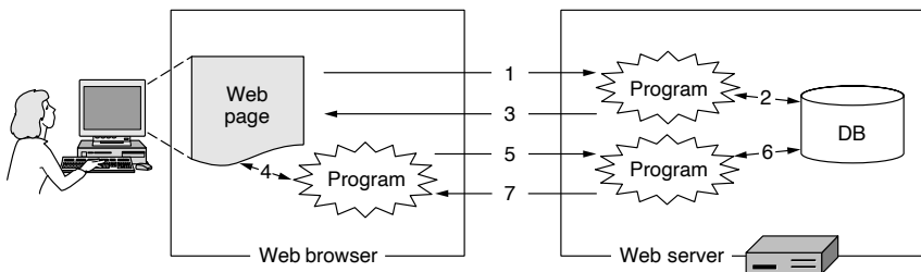
Figure 7-23. Dynamic pages.
