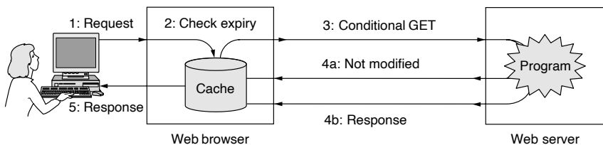
Figure 7-28. HTTP caching.
