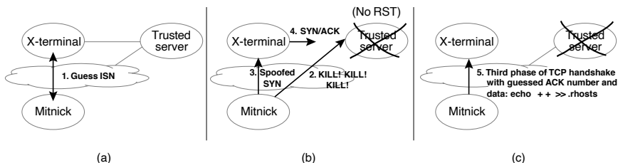
Figure 8-6. Mitnick's attack
