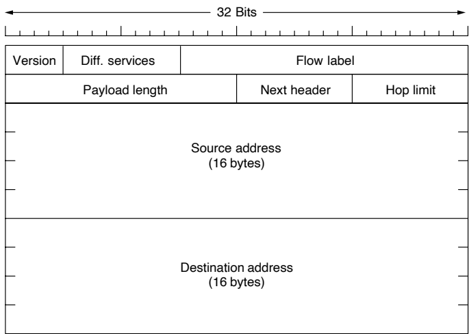
Figure 5-57. The IPv6 fixed header (required).
