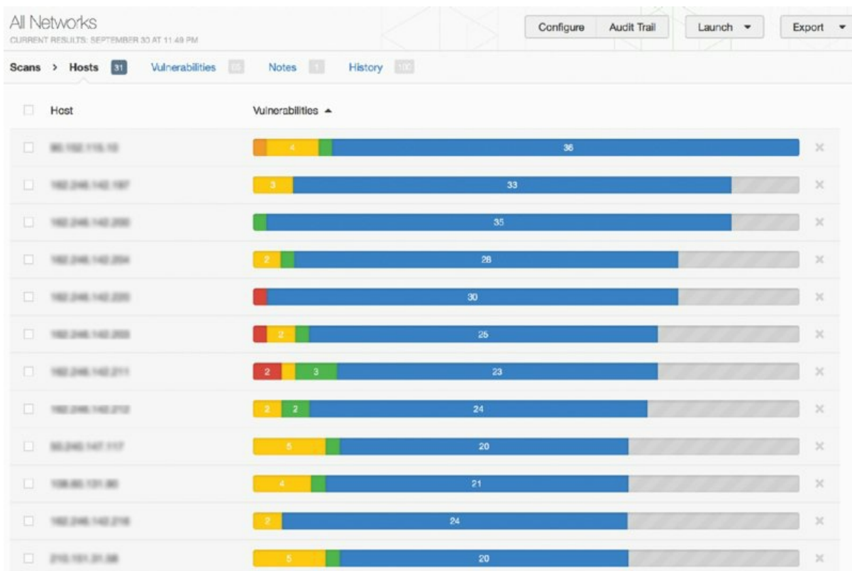
Figure 3.13 Nessus report example by IP address
