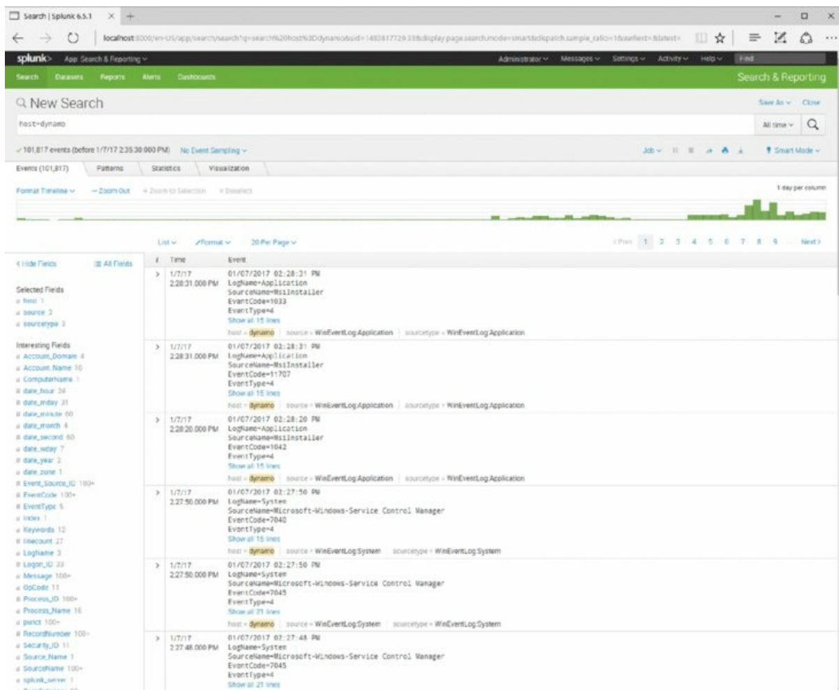
Figure 13.4 Splunk
