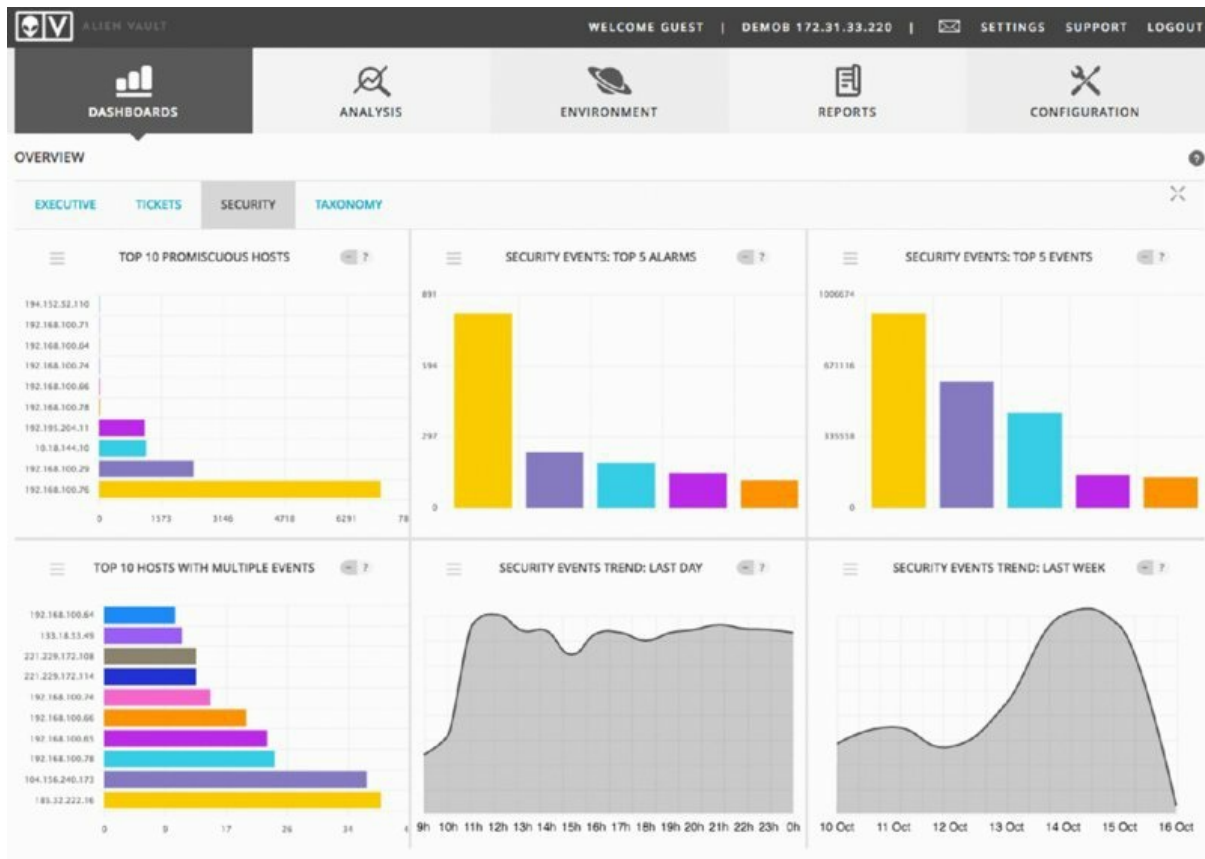
Figure 13.5 AlienVault SIEM
