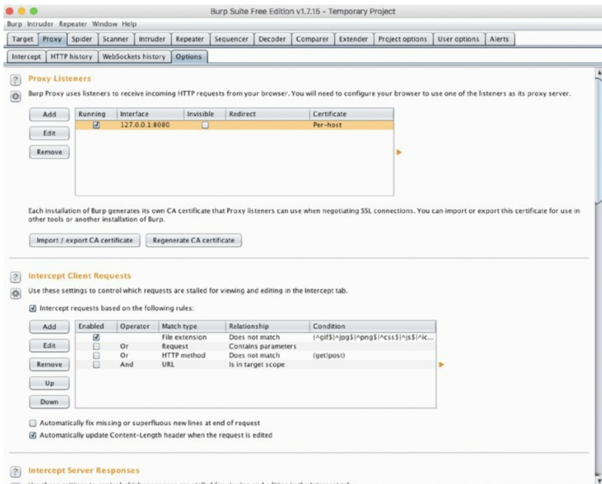
Figure 13.28 Burp Proxy
