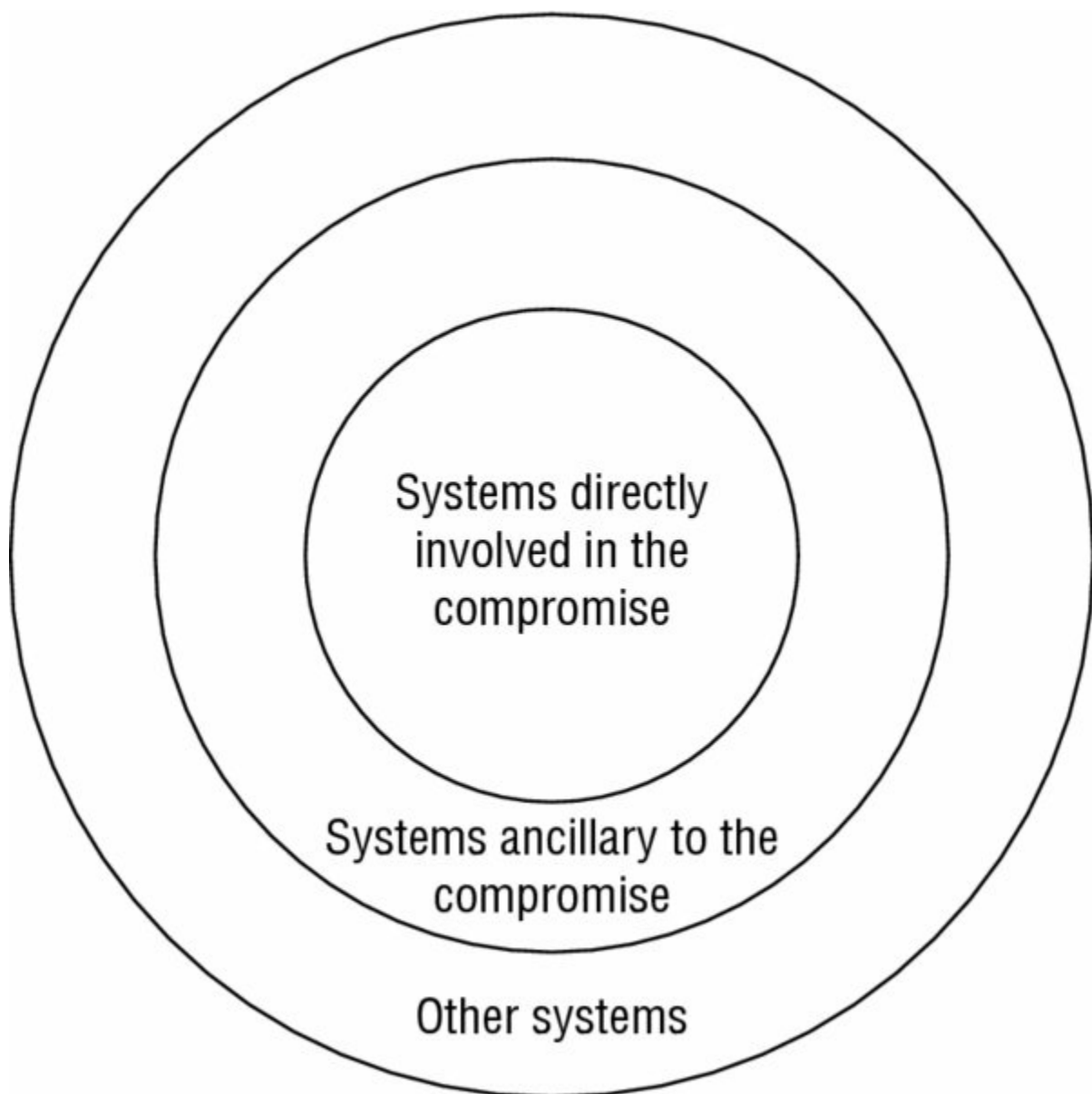
Figure 8.6 Patching priorities
