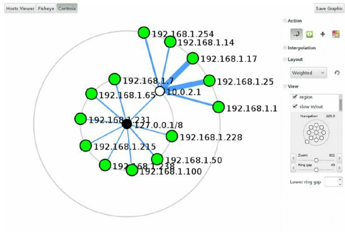
Figure 2.1 Zenmap topology view
