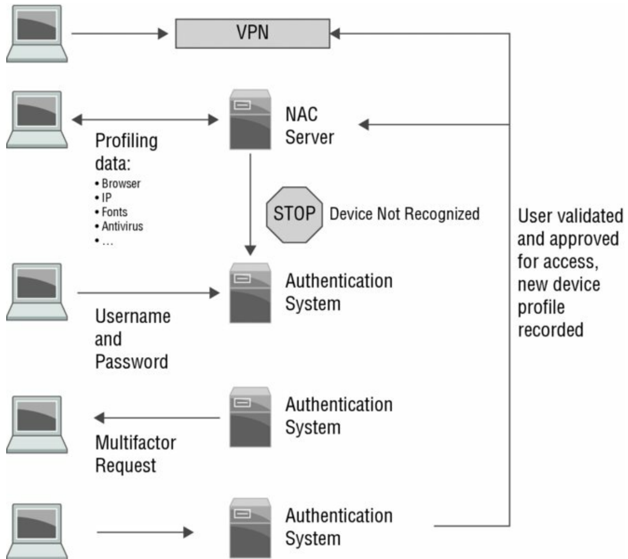
Figure 11.9 Context-based authentication
