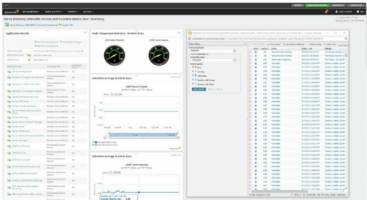
Figure 13.7 SolarWinds’s Orion
