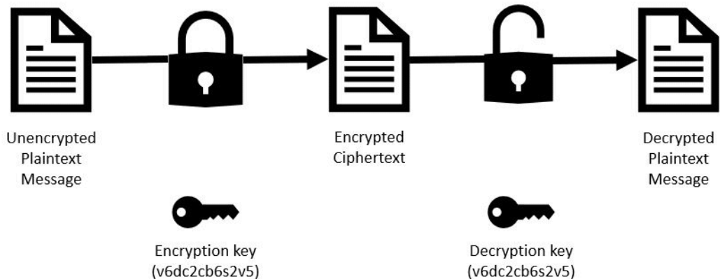
Figure 7.1 – Symmetric encryption
