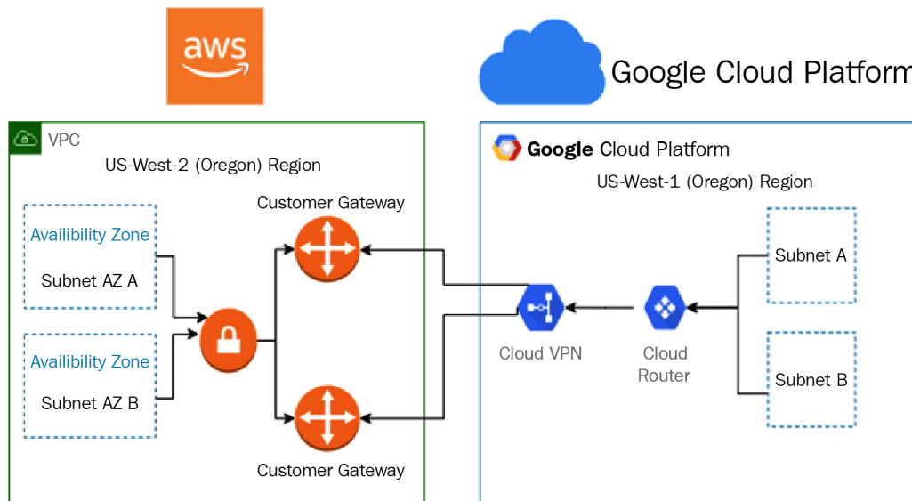
Figure 12.1 – Network connectivity from GCP to AWS
